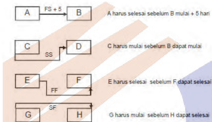
Gambar 9.1 Precedence relationship
