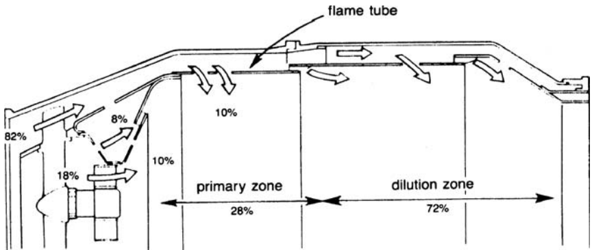
Figure 1-24. Air distribution in a typical combustor.
