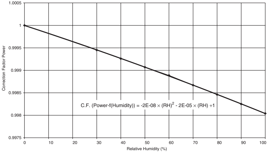
Figure 20-17. Correction factor for power as a function of inlet ambient air relative humidity.
