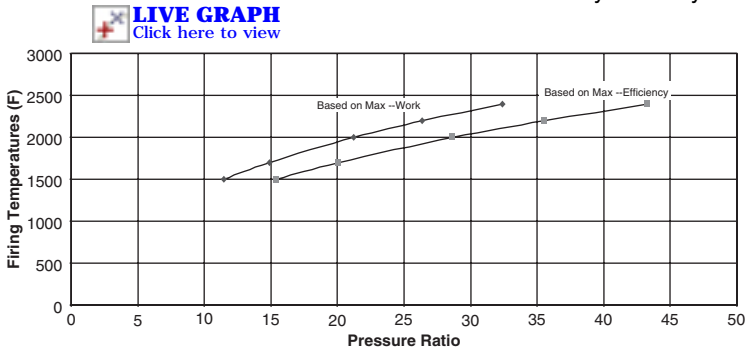
Figure 2-3. Pressure ratio based on maximum efficiency or work at various firing temperatures. Based on a compressor efficiency of 87% and a turbine efficiency of 92%.
