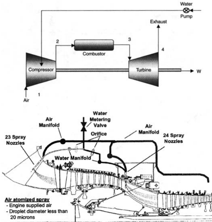
Figure 7-48. Mid-Compressor Cooling showing a schematic as well as an actual application in a GE LM 6000 Engine (courtesy GE Power Systems).
