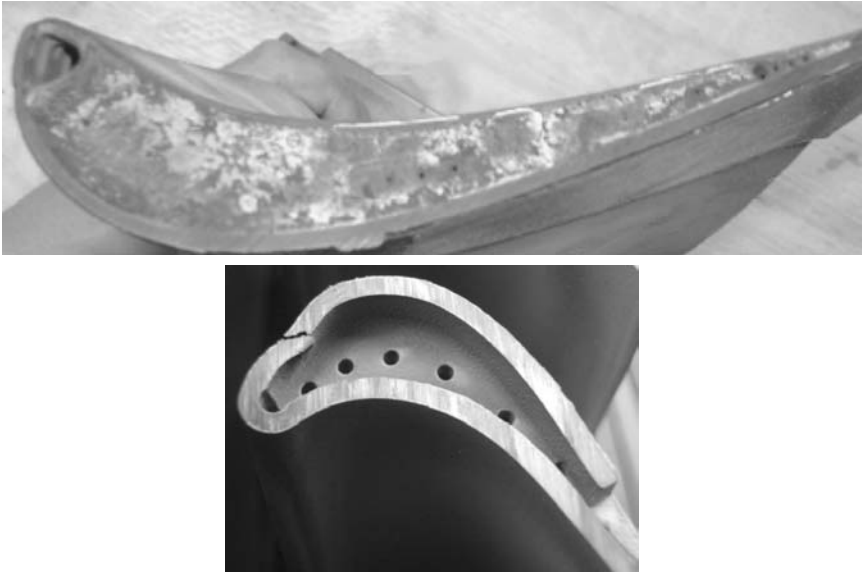
Figure 22-40. Blade tip rubs.
