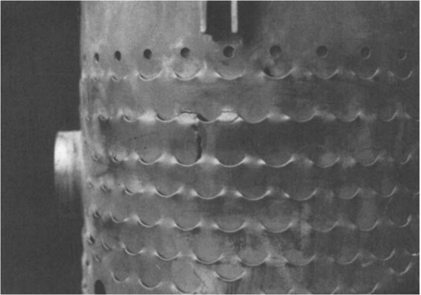
Figure 22-21. Cracks in a combustor liner.
