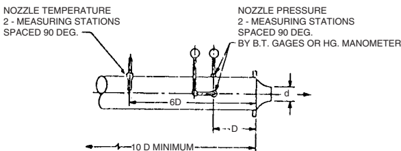
Figure 20-4. Flow nozzle for critical flow. (Power Test Code 10, Compressors and Exhausters , American Society of Mechanical Engineers, 1965.)
