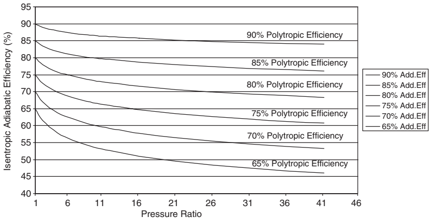
Figure 3-6. Relationship between adiabatic and polytropic efficiency.
