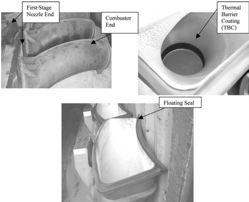
Figure 22-26. Transition pieces.
