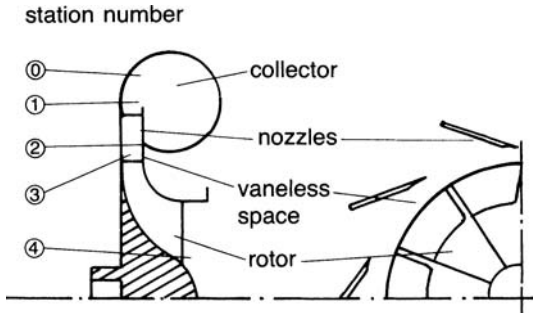
Figure 8-5. Components of a radial-inflow turbine.
