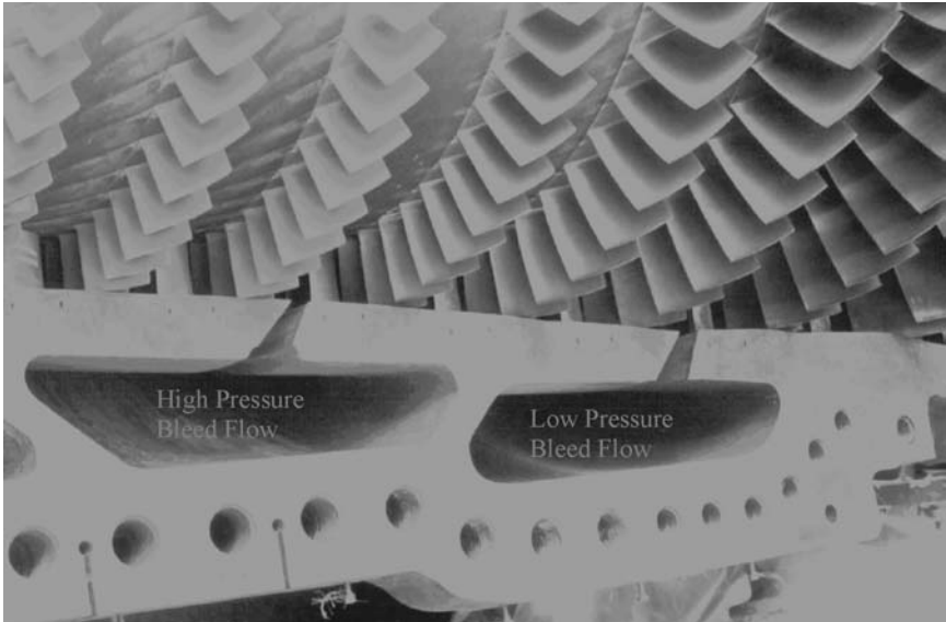
Figure 22-7. Axial-flow compressor showing bleed flow ports.
