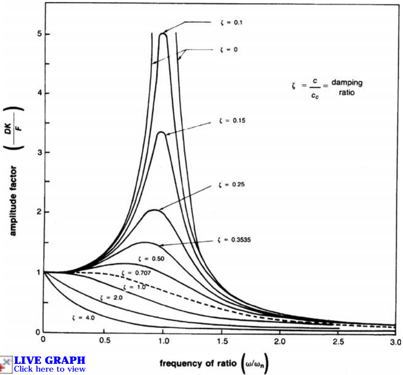
Figure 5-13a. Amplitude factor as a function of the frequency ratio r for various amounts of viscous damping.
