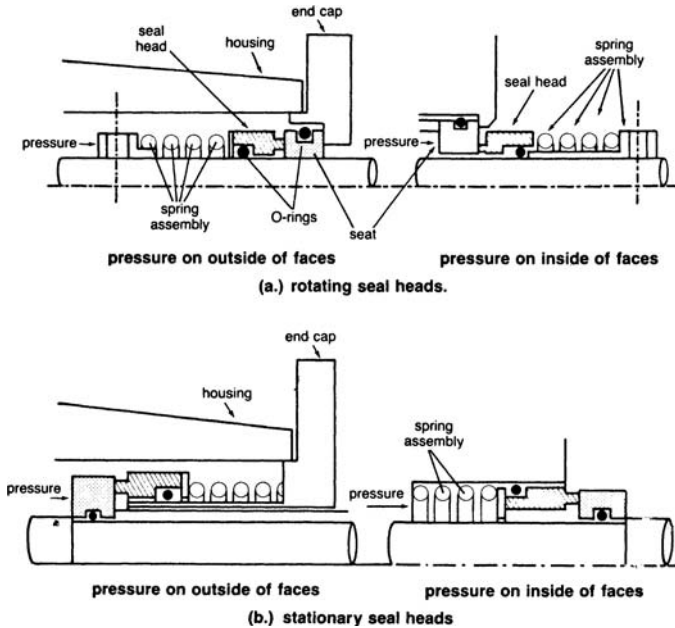
Figure 13-26. Rotating and stationary seal heads.
