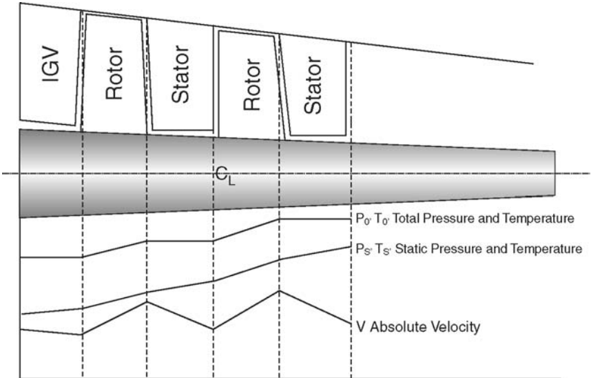
Figure 7-5. Variation of temperature (enthalpy), velocity, and pressure through an axial-flow compressor.
