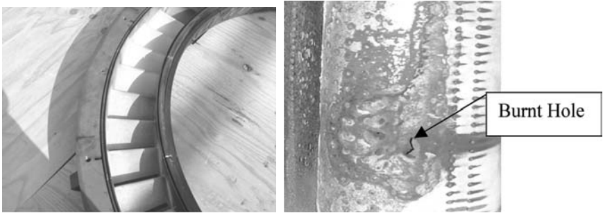
Figure 22-27. First-stage nozzle vanes.
