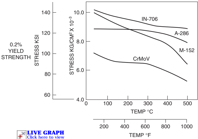
Figure 11-7. Turbine wheel alloys tensile strength comparison.
