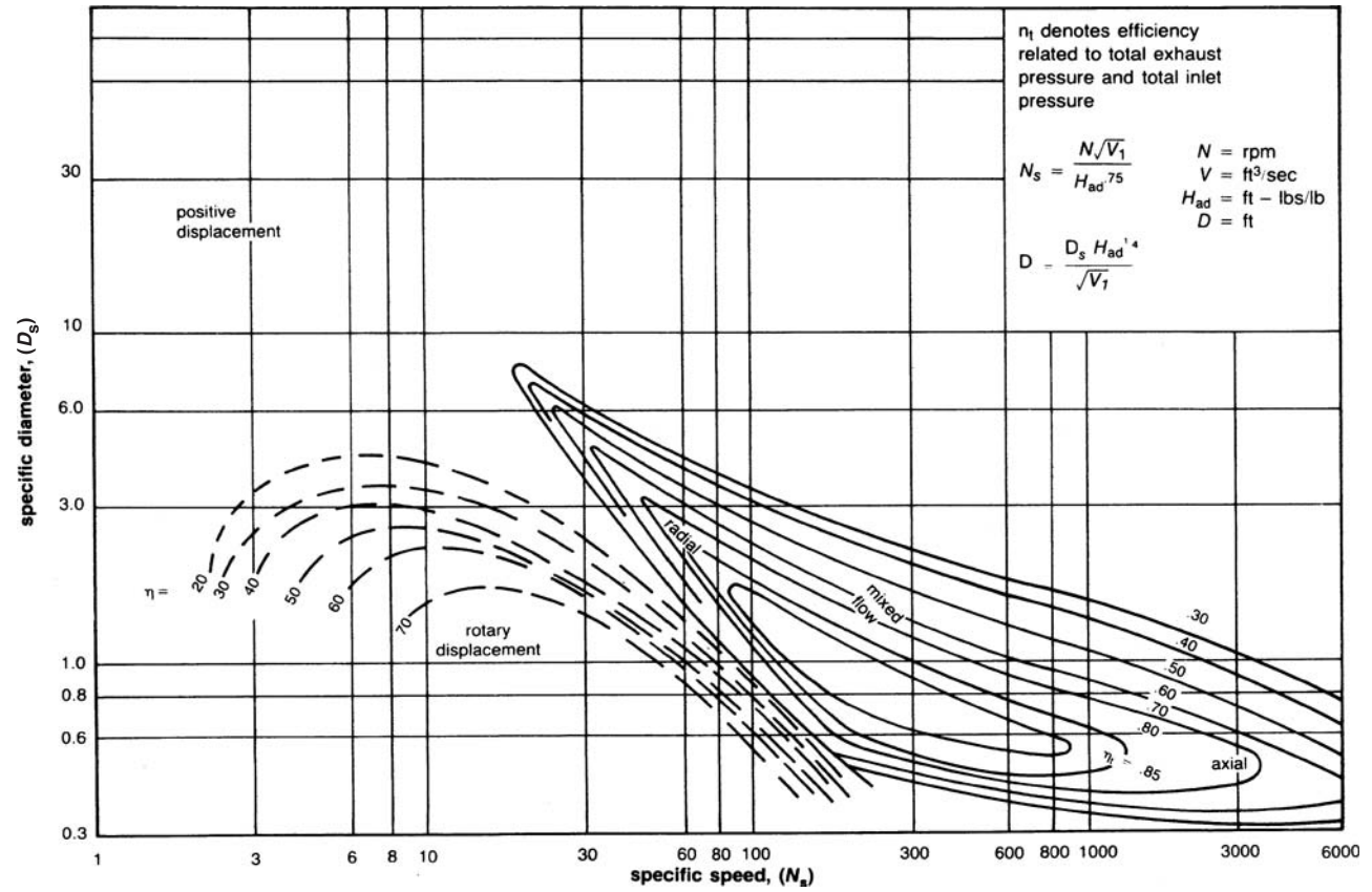
Figure 3-8a. Compressor map.
