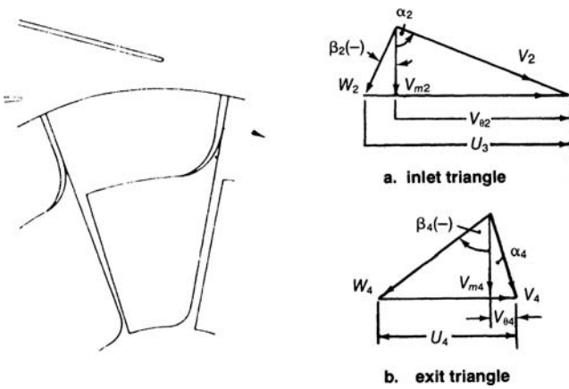
Figure 8-10. Velocity triangles for a radial-inflow turbine.
