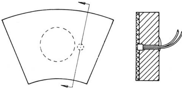
Figure 21-20. RTD embedded in bearing surface.
