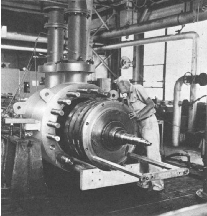
Figure 6-46. Barrel-type compressor. (Courtesy Elliott Company, Jeannette, PA.)
