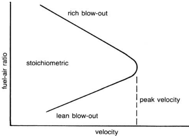
Figure 10-5. Range of burnable fuel-air ratios versus combustor gas velocity.
