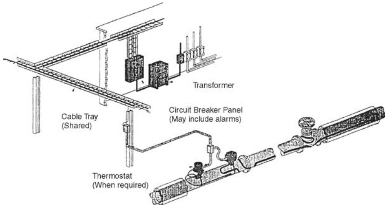
Figure 12-16. Electric heat tracing system.
