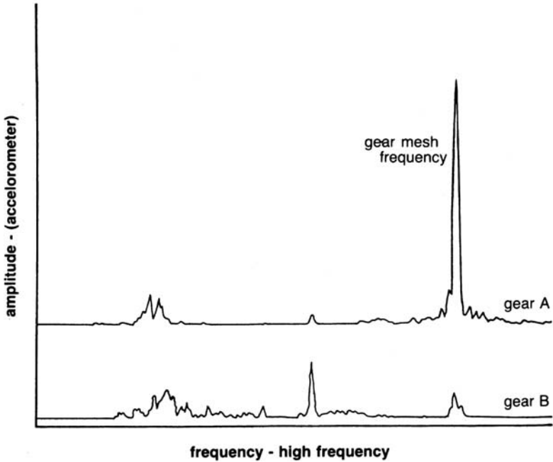
Figure 16-13. Gear box signature (high-frequency end).
