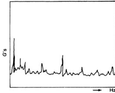
Figure 7-34. Fifth-stage bleed pressure—5800 rpm.
