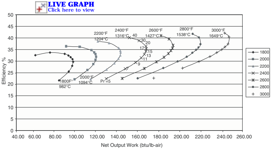
Figure 1-6. Performance map of a simple cycle gas turbine.
