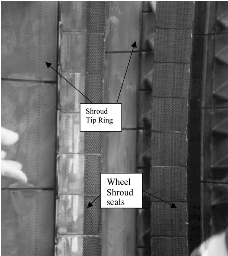
Figure 22-41. Turbine casing and vane sections.
