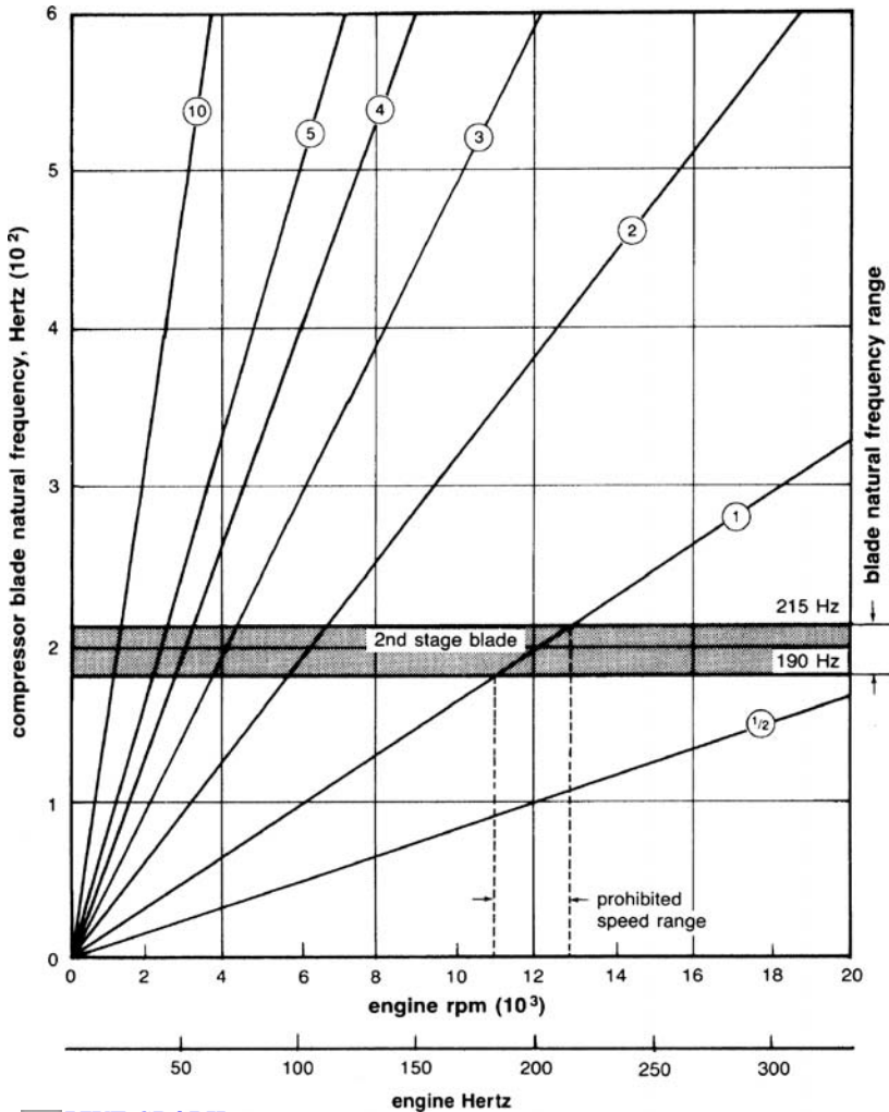
Figure 5-25. Campbell diagram.
