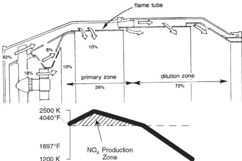
Figure 10-19. A typical combustor showing the NO x production zone.
