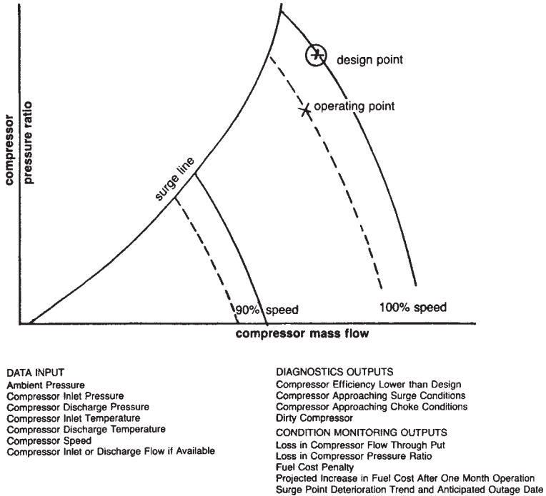
Figure 19-15. Aerothermal condition monitoring for compressors.
