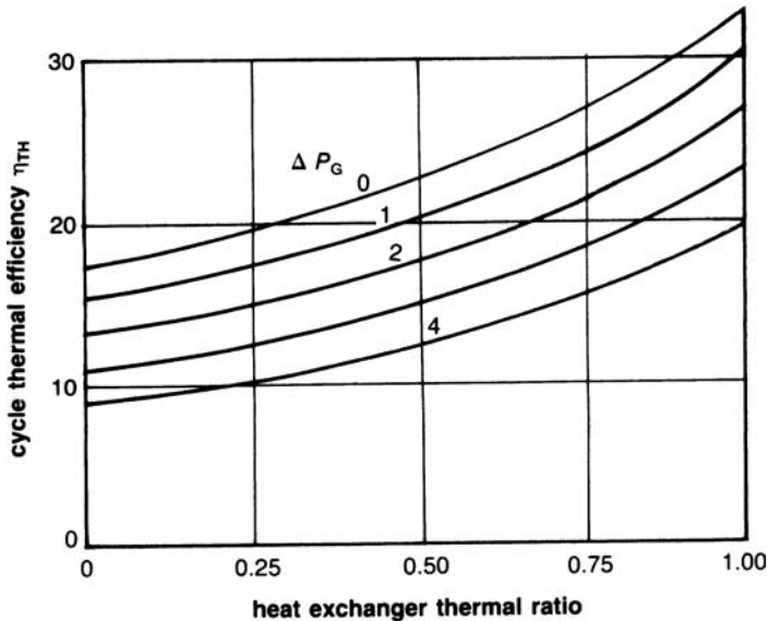
Figure 2-5. Variation of a gas turbine cycle efficiency with heat exchanger performance.
