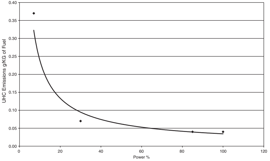
Figure 20-18. UHC emissions for a typical gas turbine.
