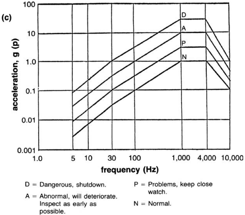
Figure 13-16. (continued). Severity chart: (c) acceleration.
