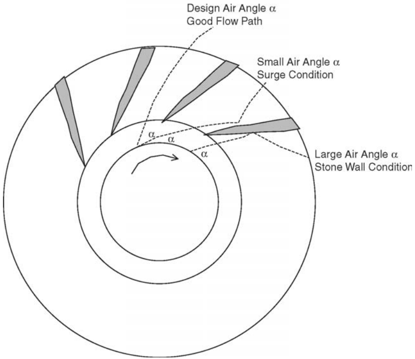
Figure 6-39. Vaned diffuser.
