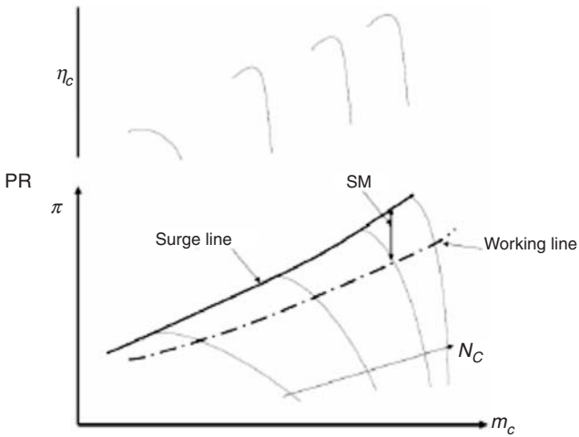
Figure 7-26. Multistage axial compressor maps.
