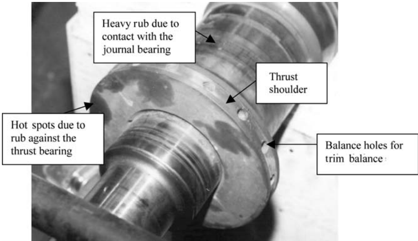
Figure 22-49. Journal shaft with thrust shoulder.
