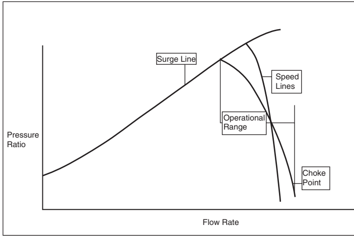
Figure 21-12. Compressor performance map.
