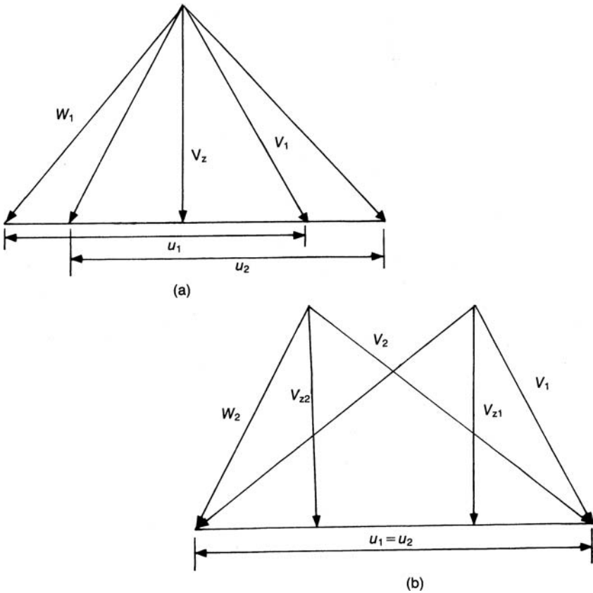
Figure 7-12. Velocity triangles.
