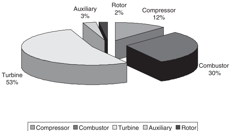
Figure 22-53. Major failures in gas turbines less than 170 MW.
