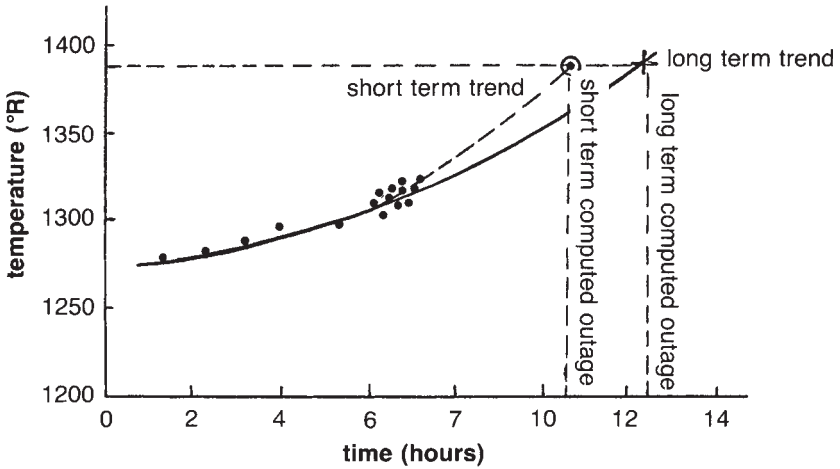
Figure 19-16. Temperature versus expected outage time.
