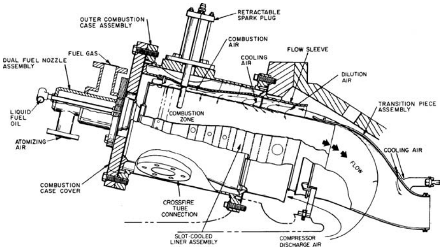
Figure 1-25. A typical reverse-flow can-annular combustor.
