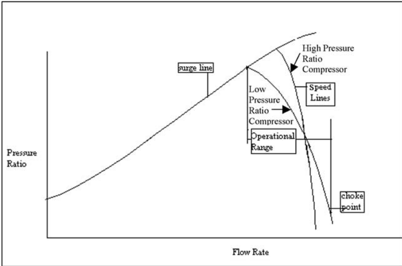
Figure 22-1. Compressor performance map.
