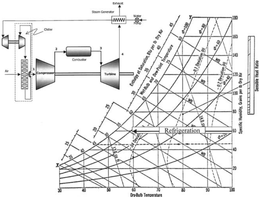
Figure 2-36. Mechanical refrigerated inlet system used to cool the inlet air of the gas turbine.
