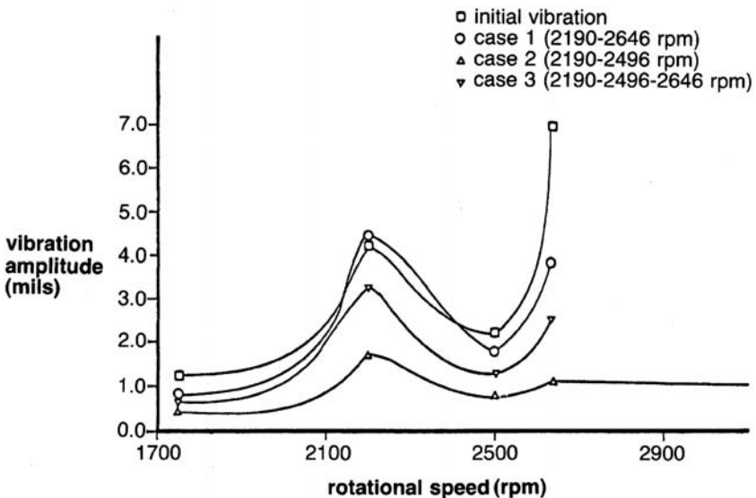
Figure 17-9. Rotor amplitude for least-square balance.
