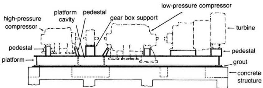
Figure 21-23. Typical compressor train containing a turbine and two compressor stages.
