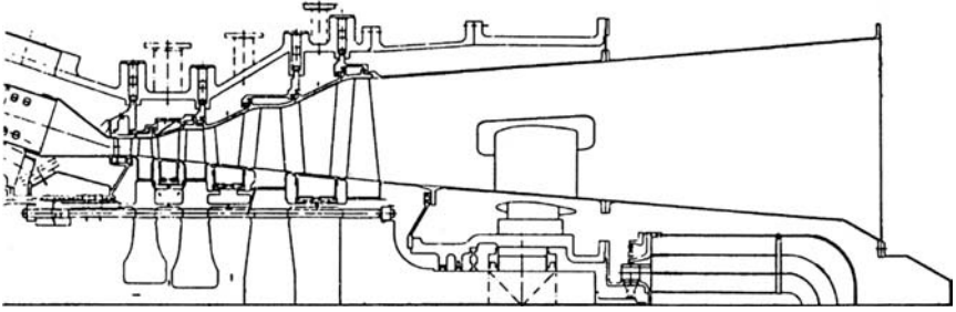
Figure 1-37. Schematic of an axial-flow turbine.
