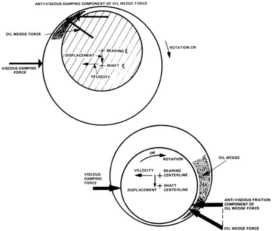
Figure 13-15. Oil whirl.
