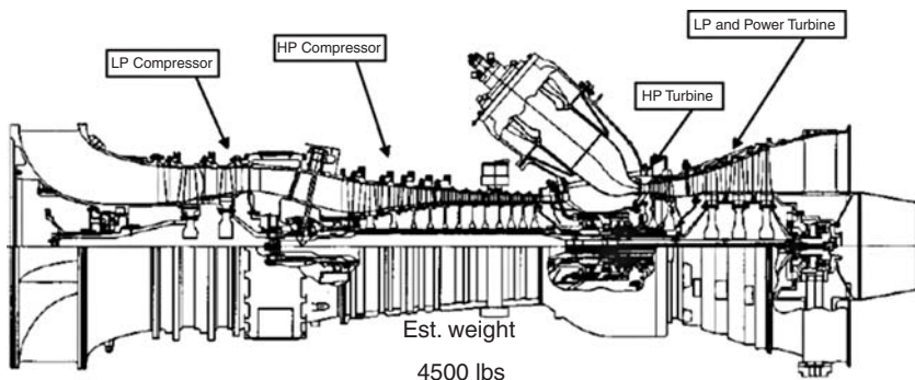
Figure 1-10. A cross section of an aero-derivative gas turbine engine.
