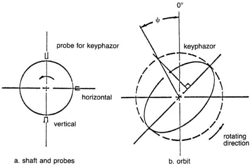
Figure 17-7. Typical probe positions and the phase angle in an elliptical orbit.
