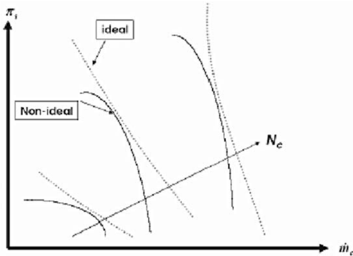
Figure 7-36. Performance map of compressor stage.
