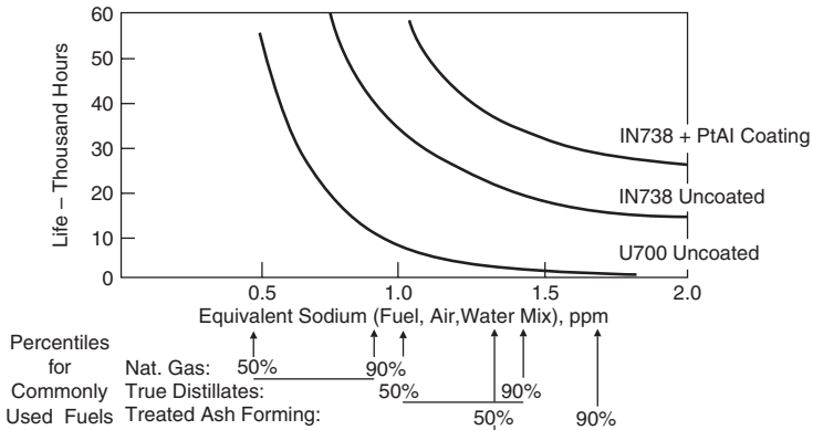
Figure 11-8. Effect of sodium corrosion on blade life.
