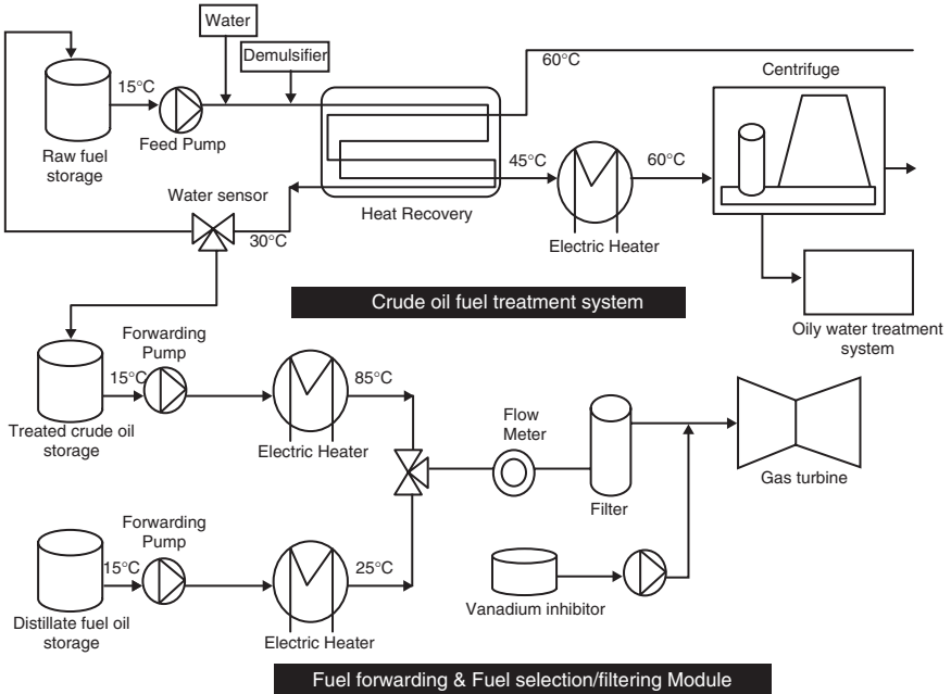
Figure 12-5. A typical fuel treatment system.
