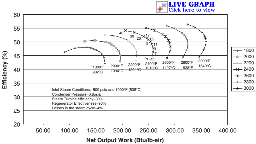
Figure 2-27. The performance map of a typical combined cycle power plant.
