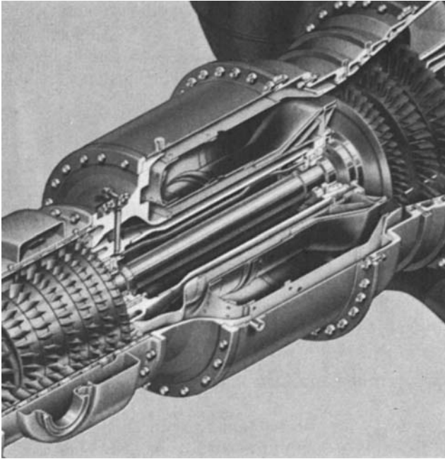
Figure 10-17. Industrial-type can-annular combustor. (Courtesy of Solar Turbines Incorporated.)
