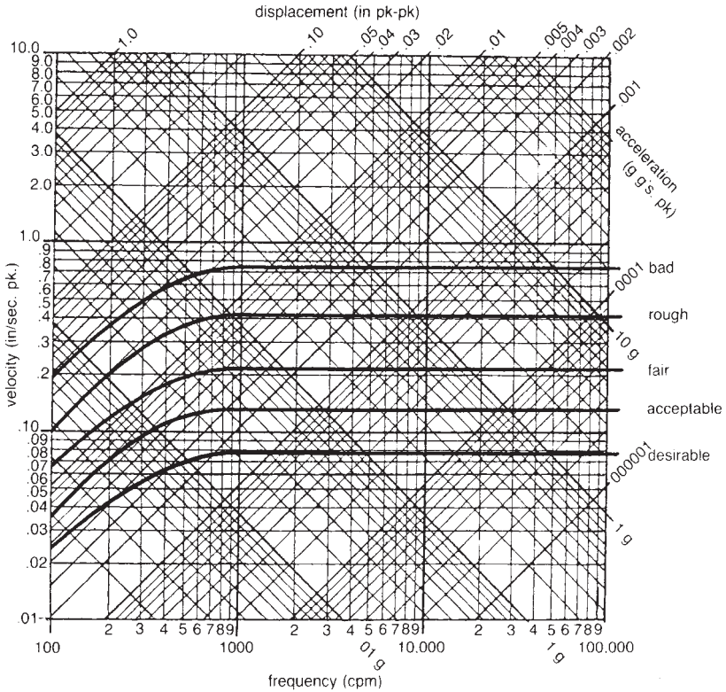
Figure 19-13. Vibration nomograph and severity chart. (Courtesy of IRD Mechanical, Inc.)
