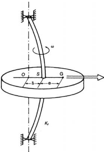
Figure 5-14a. Rigid supports.
