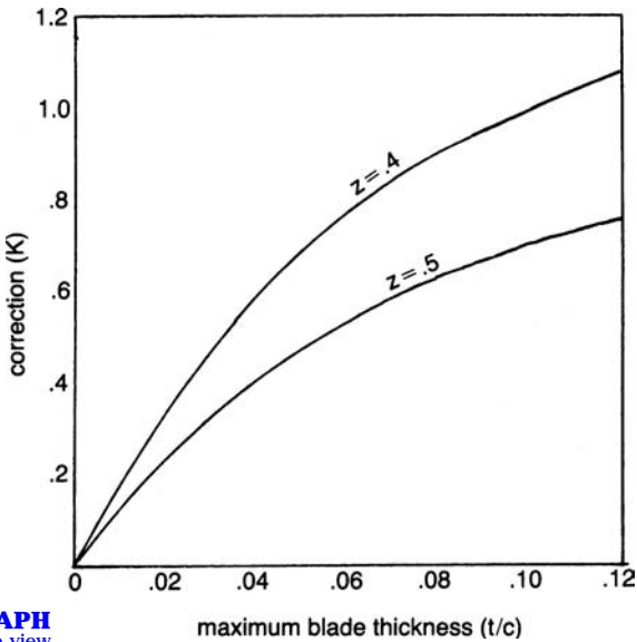
Figure 7-19. Correction factor for blade thickness and incidence angle calculation.
