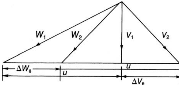
Figure 7-14. Axial-entry stage velocity diagram.
