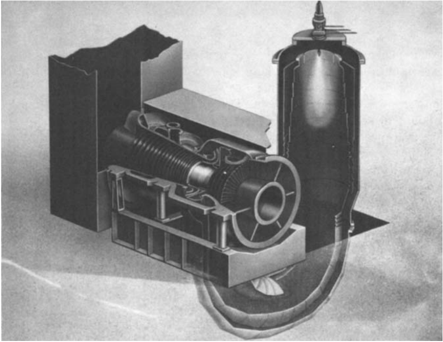
Figure 10-13. Single can combustor. (Courtesy Brown Boveri Turbomachinery, Inc.)
