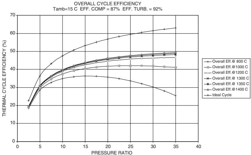
Figure 20-9. Effect of pressure ratio and firing temperature on the performance of a gas turbine.
