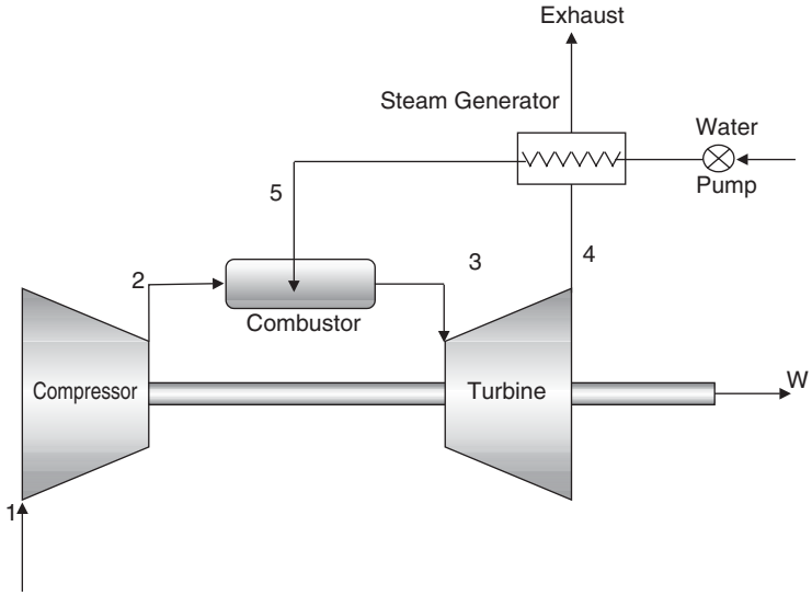
Figure 2-43. Steam injection in the gas turbine combustor.
