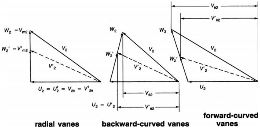
Figure 6-10. Velocity triangles.
