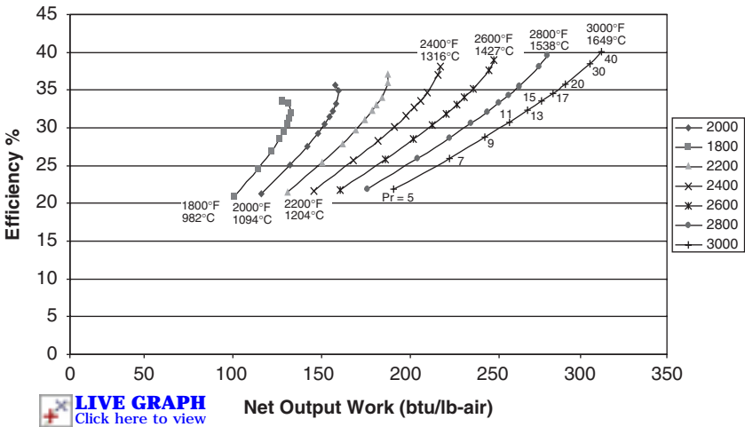
Figure 2-15. The performance map of an intercooled gas turbine cycle.
