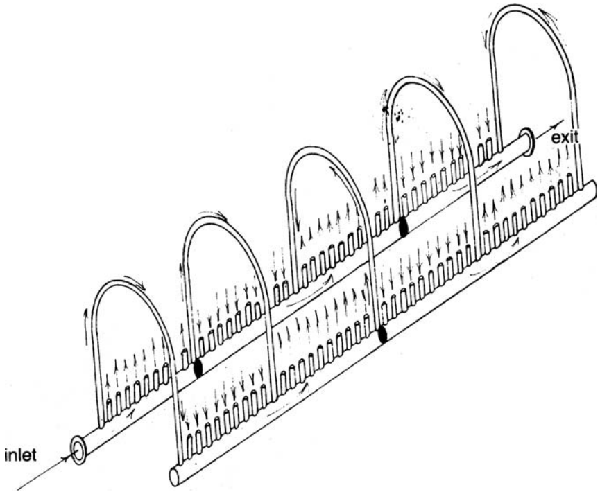
Figure 1-29. An external fired combustor with four passes.
