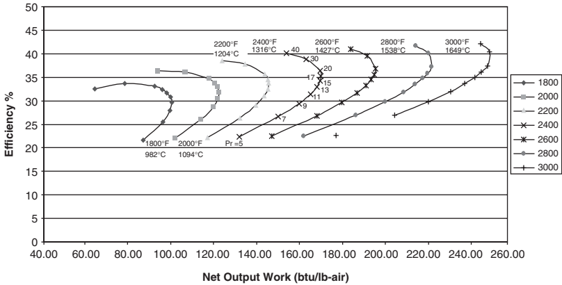
Figure 2-10. The performance map of a simple-cycle gas turbine.
