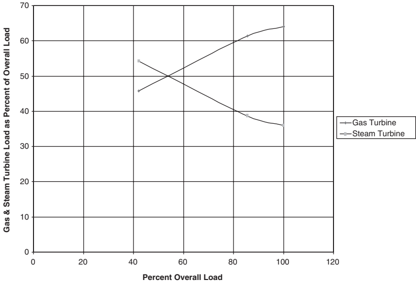
Figure 2-31. Load sharing between prime movers over the entire operating range of a combined cycle power plant.
