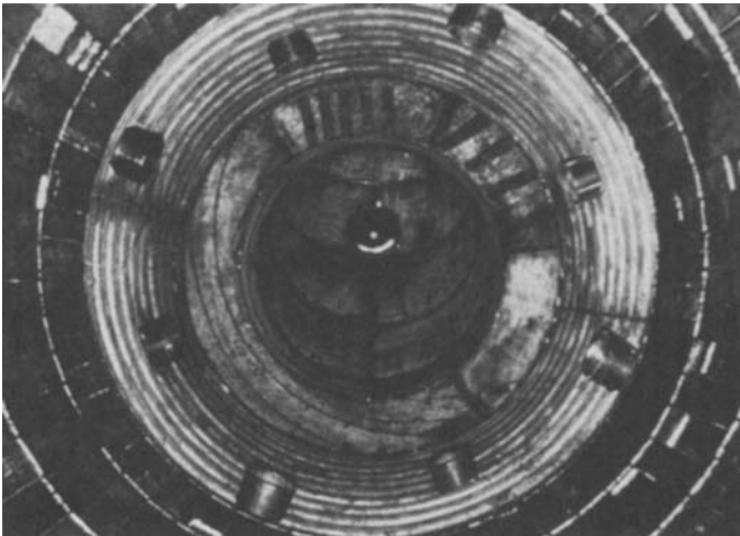
Figure 10-12b. Special tiles for a large side combustor. (Courtesy Brown Boveri Turbomachinery, Inc.)
