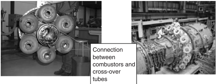
Figure 22-18. A typical can-annular combustion arrangement.
