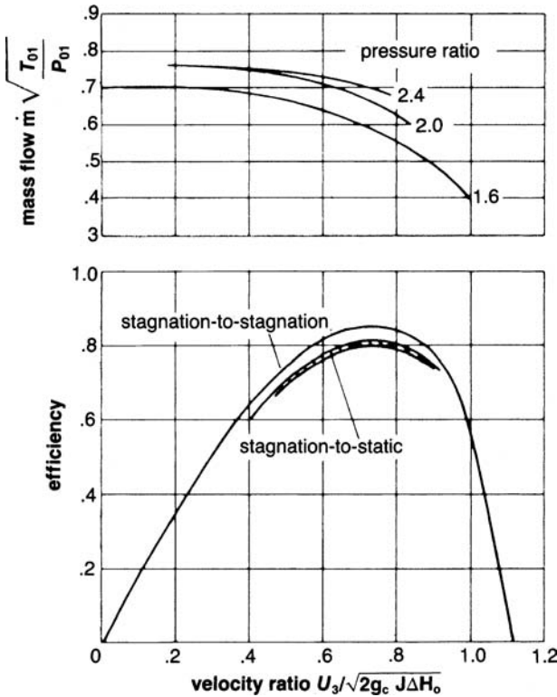
Figure 8-11. An example of a radial-flow turbine characteristic. (Courtesy Institution of Mechanical Engineers.)
