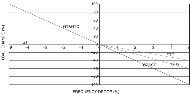
Figure 19-4. Droop curves for Combined Cycle Power Plants.
