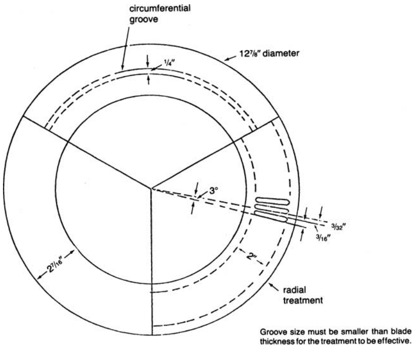
Figure 7-44. Details of the various casing treatments. Each treatment was on a separate disc.
