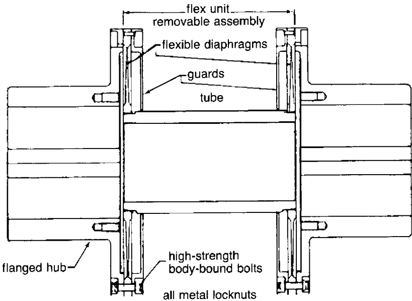
Figure 18-7. Schematic of atypical diaphragm coupling. (Courtesy of Kóppers Company, Inc.)
