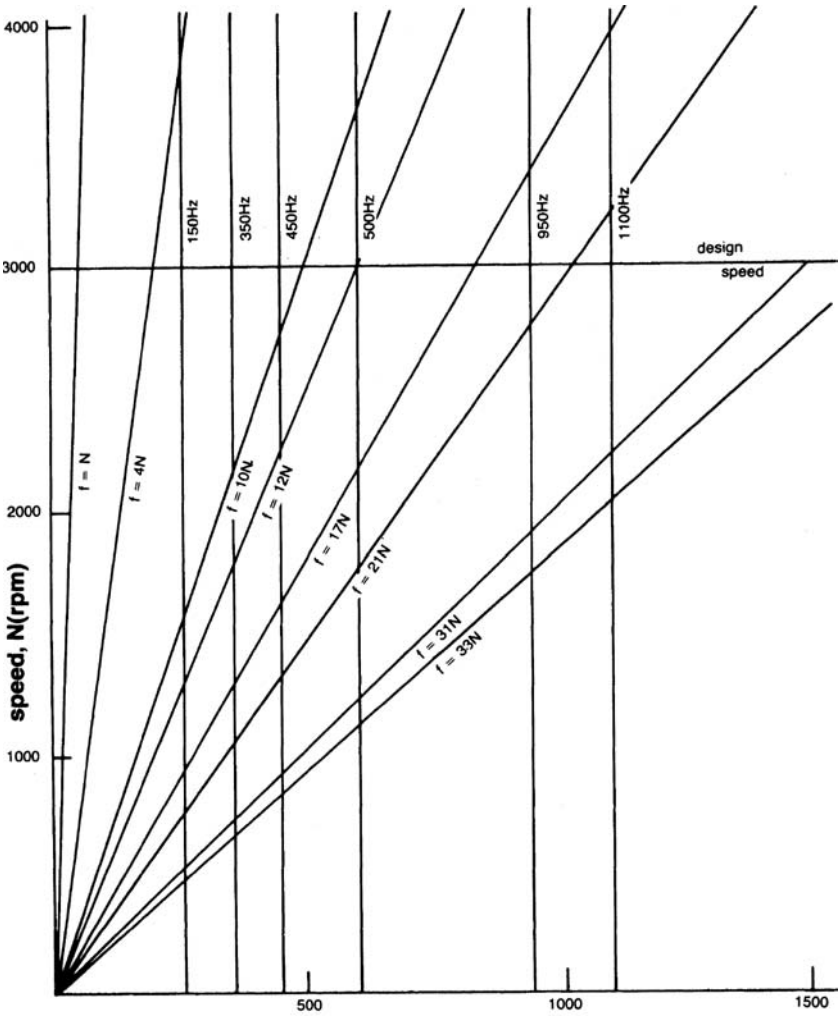
Figure 5-28. Campbell diagram of tested impeller.
