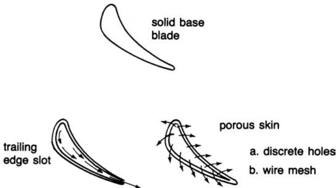
Figure 9-24. Cooled turbine blade types.
