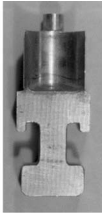
Figure 22-44. Erosion and corrosion in the blade fir tree region.
