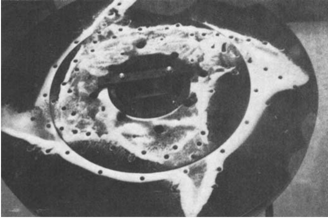
Figure 5-27. Impeller showing nodal points.
