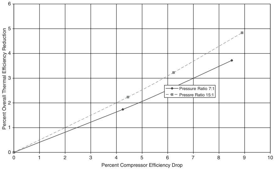
Figure 21-13. Effect of compressor efficiency drop on the overall thermal efficiency reduction.
