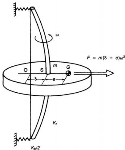
Figure 5-14b. Flexible supports.
