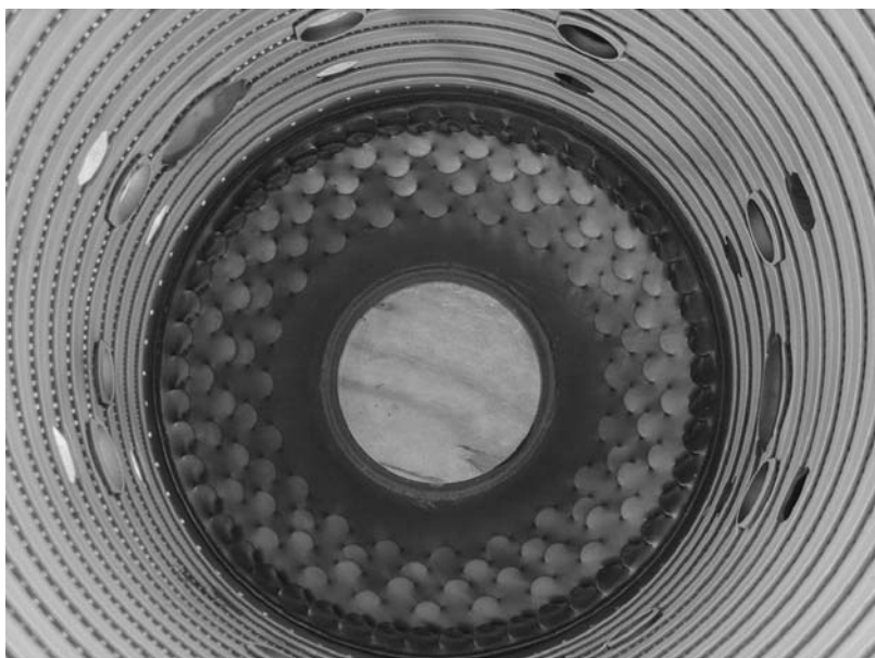
Figure 22-23. Can-annular combustor with TBC.
