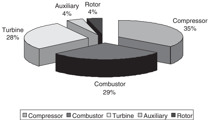
Figure 22-54. Major failures in gas turbines larger than 220 MW.
