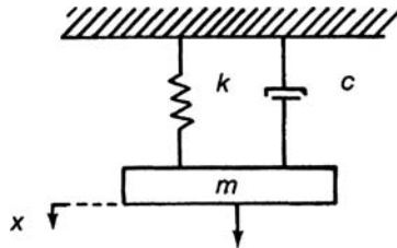
Figure 5-10. Forced vibration system.
