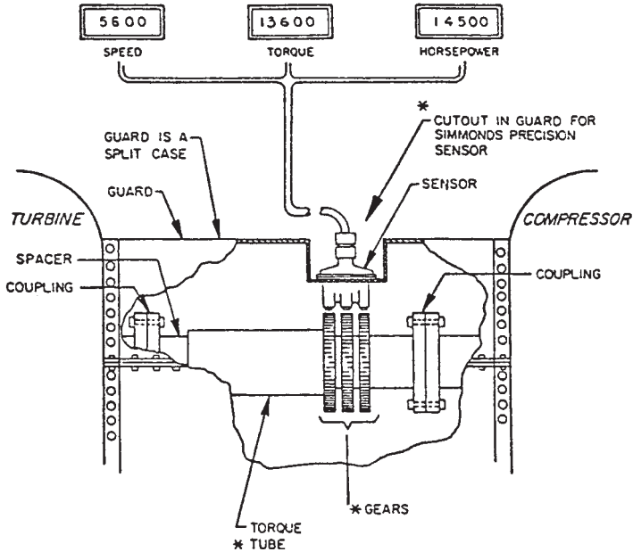
Figure 19-14. Torque meter for a gas turbine.
