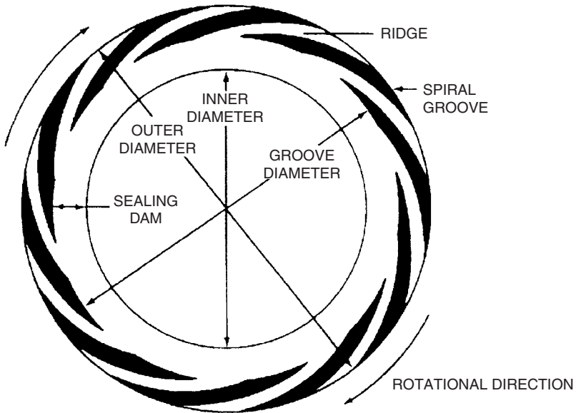
Figure 13-36. Spiral grooved mating ring. (Courtesy Proceedings Seventeenth Turbomachinery Symposium, Dry Gas Compressor Seals by Piyush Shah, John Crane Inc.)
