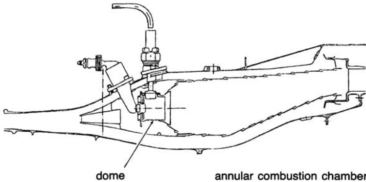
Figure 12-10. Cross section of an annular combustor showing high dome flow configuration. (Courtesy of General Electric Company.)
