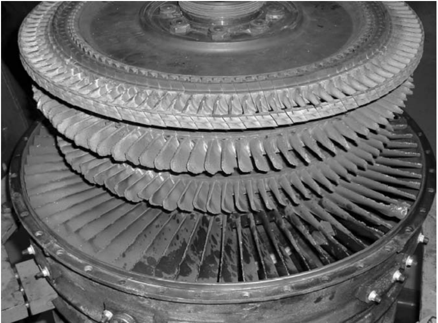
Figure 22-32. Turbine rotor shaft.
