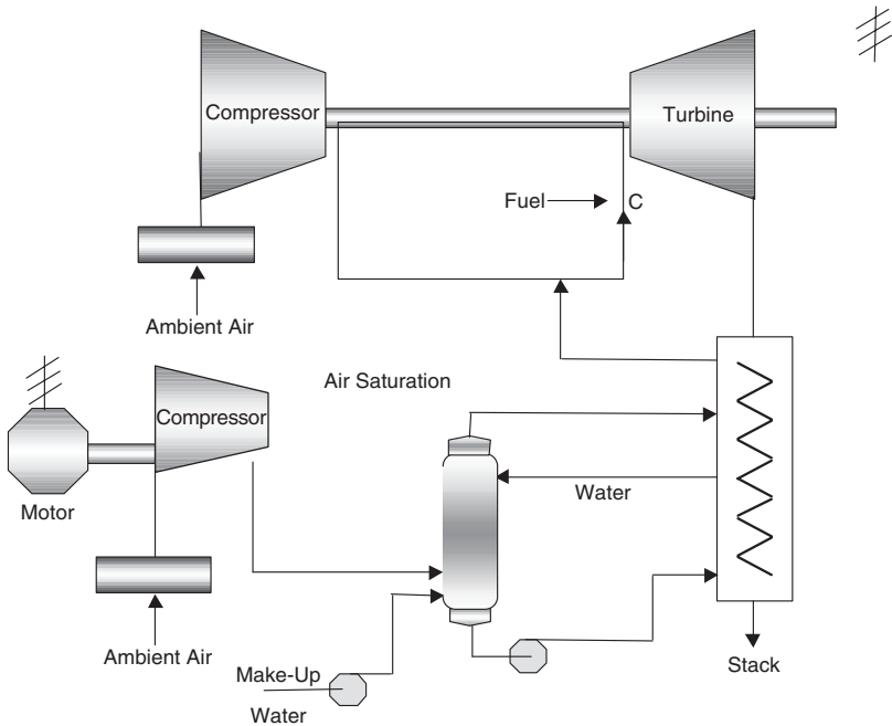
Figure 2-41. Heated and humidified compressed air injection system for power augmentation of a gas turbine.
