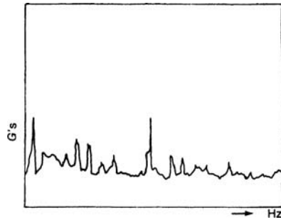
Figure 7-35. Fifth-stage bleed pressure—6800 rpm.
