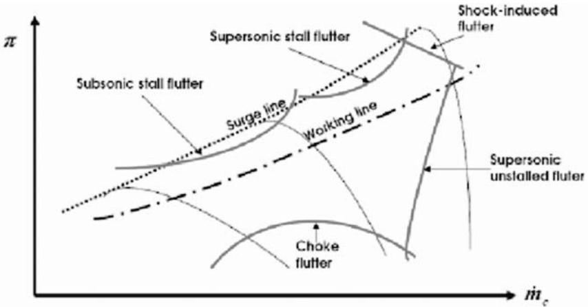
Figure 7-29. Flutter regions on the operating map of a transonic compressor (after Mikolajczak et al., 1975).
