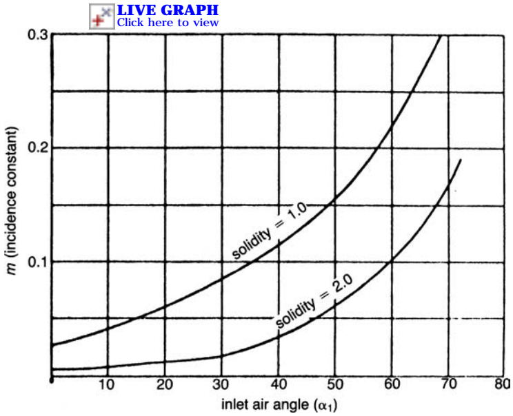
Figure 7-18. Slope of incidence angle variation with air angle.
