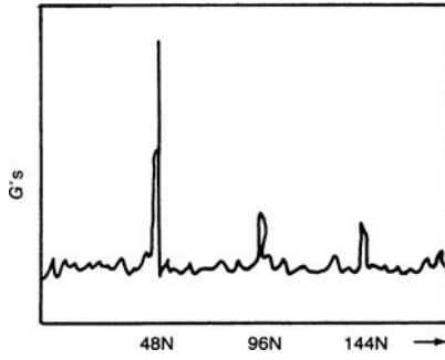
Figure 7-32. High-pressure bleed chamber—8000 rpm.
