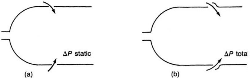
Figure 10-9. Film cooling of a combustor liner.
