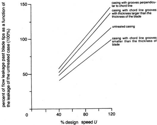
Figure 7-46. Mass flow leakage at tips for various casing treatments.
