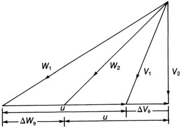
Figure 7-15. Axial-outflow stage velocity diagram.
