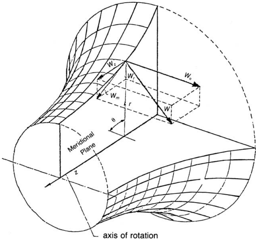
Figure 8-6. Velocity vectors in turbine rotor flow.
