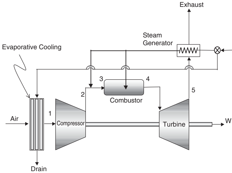
Figure 2-44. Evaporation cooling and steam injection in a gas turbine.
