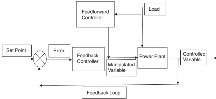
Figure 19-1. Feedforward and feedback control loop.
