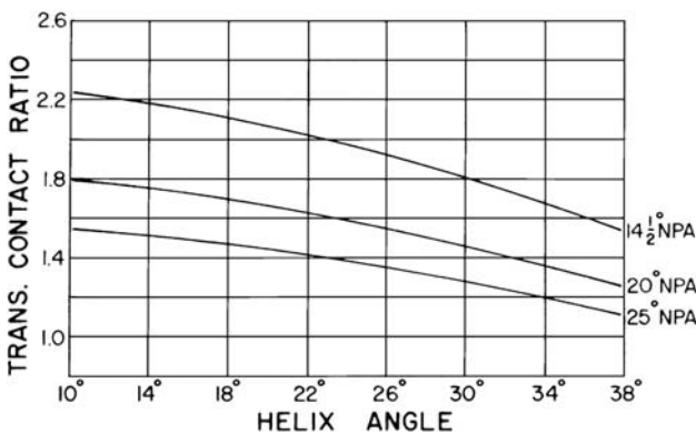
Figure 14-3. Variation of transverse contact ratio with pressure angle and helix angle. (Courtesy of Lufkin Industries, Inc.)
