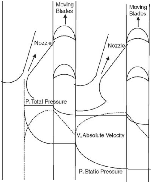
Figure 9-8. Pressure and velocity distributions in a Ratteau-type impulse turbine.
