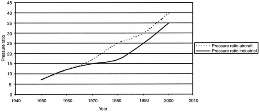
Figure 7-1. Development of pressure ratio over the past 50 years.
