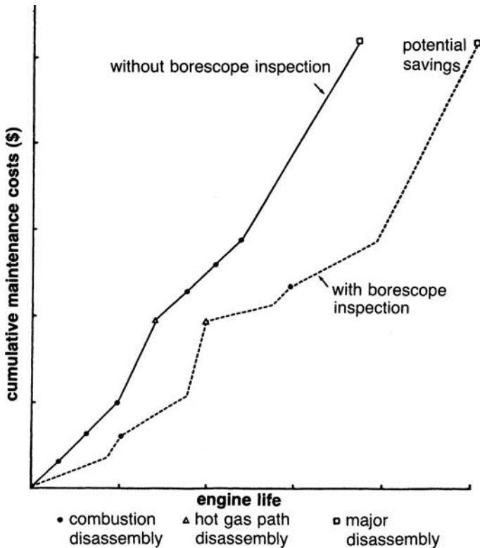
Figure 21-8. Effect of planned maintenance with usage of borescope.
