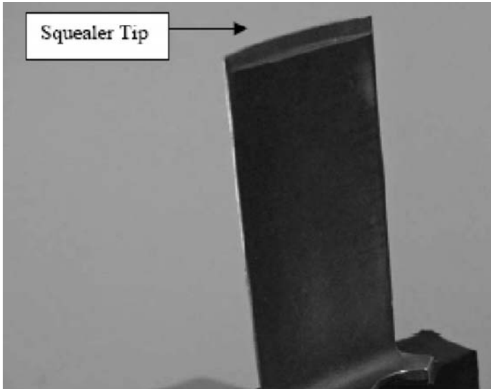
Figure 7-39. Axial-flow compressor rotor blade with squealer tip.
