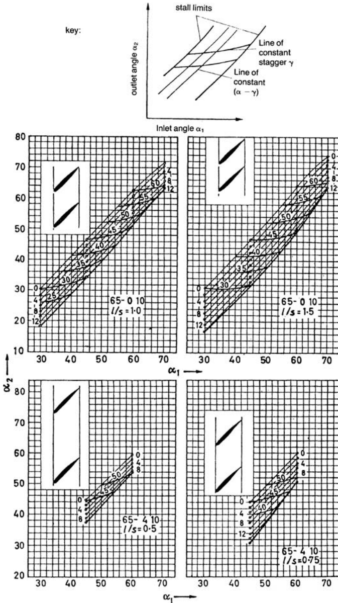
Figure 7-24. The NACA 65 series cascade data. (Courtesy of G. Mellor, Massachusetts Institute of Technology, Gas Turbine Laboratory Publication.)
