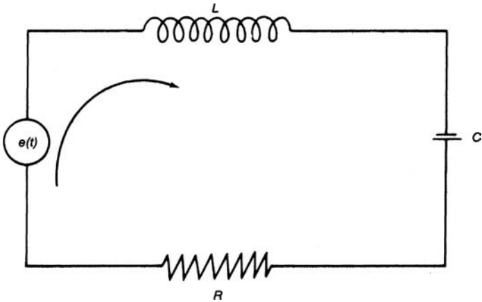
Figure 5-18. A force-voltage system.
