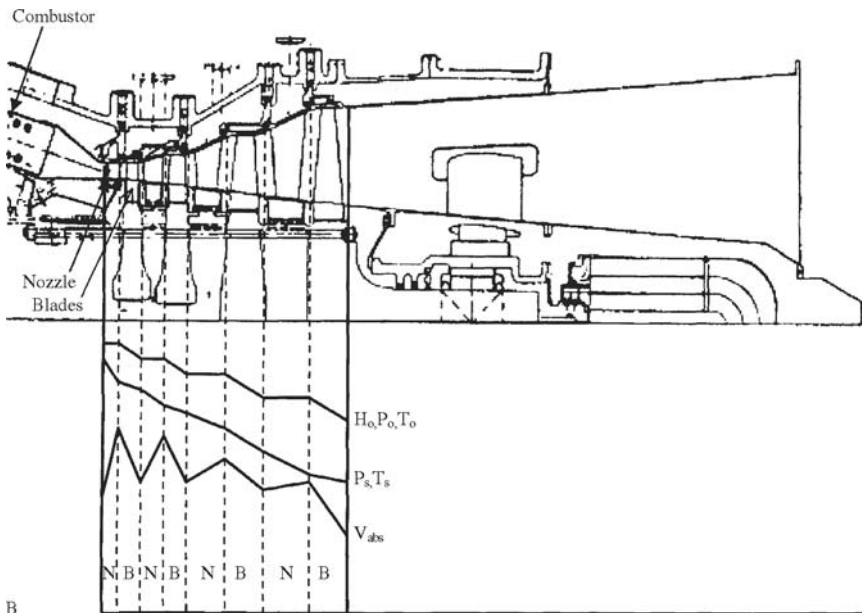
Figure 9-1. Schematic of axial-flow turbine flow characteristics.
