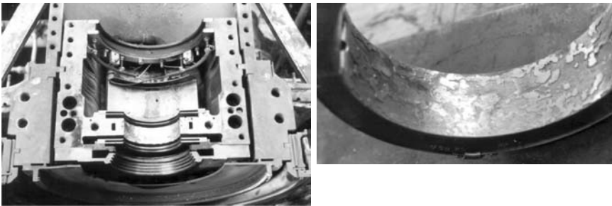
Figure 22-47. Journal bearing babbitt has been mainly wiped out due to excessive rub.
