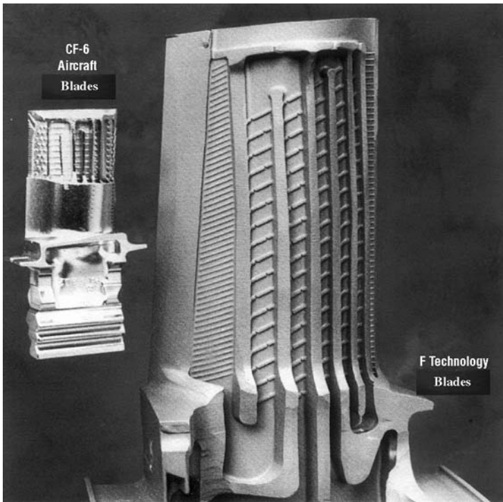
Figure 9-18. Internal of the frame FA blades, showing cooling passage. (Courtesy GE Power Systems.)
