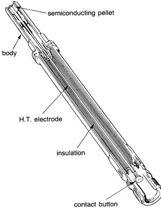
Figure 10-11. An ignitor plug. (© Rolls-Royce Limited.)
