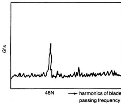
Figure 7-30. High-pressure bleed chamber—4100 rpm.
