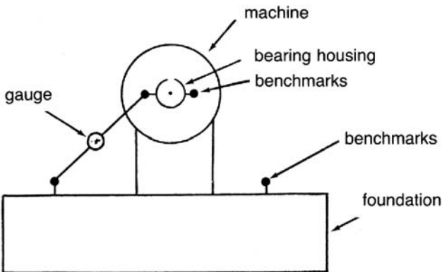
Figure 18-18. Hot alignment system with dial indicator.
