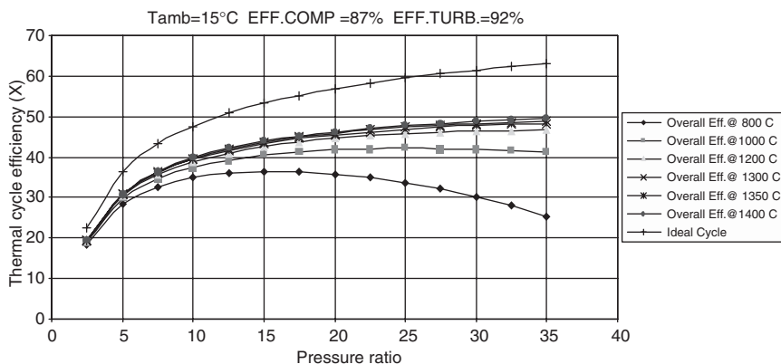
Figure 1-5. Overall cycle efficiency.
