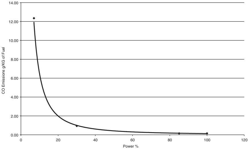
Figure 20-19. CO emissions for a typical gas turbine.
