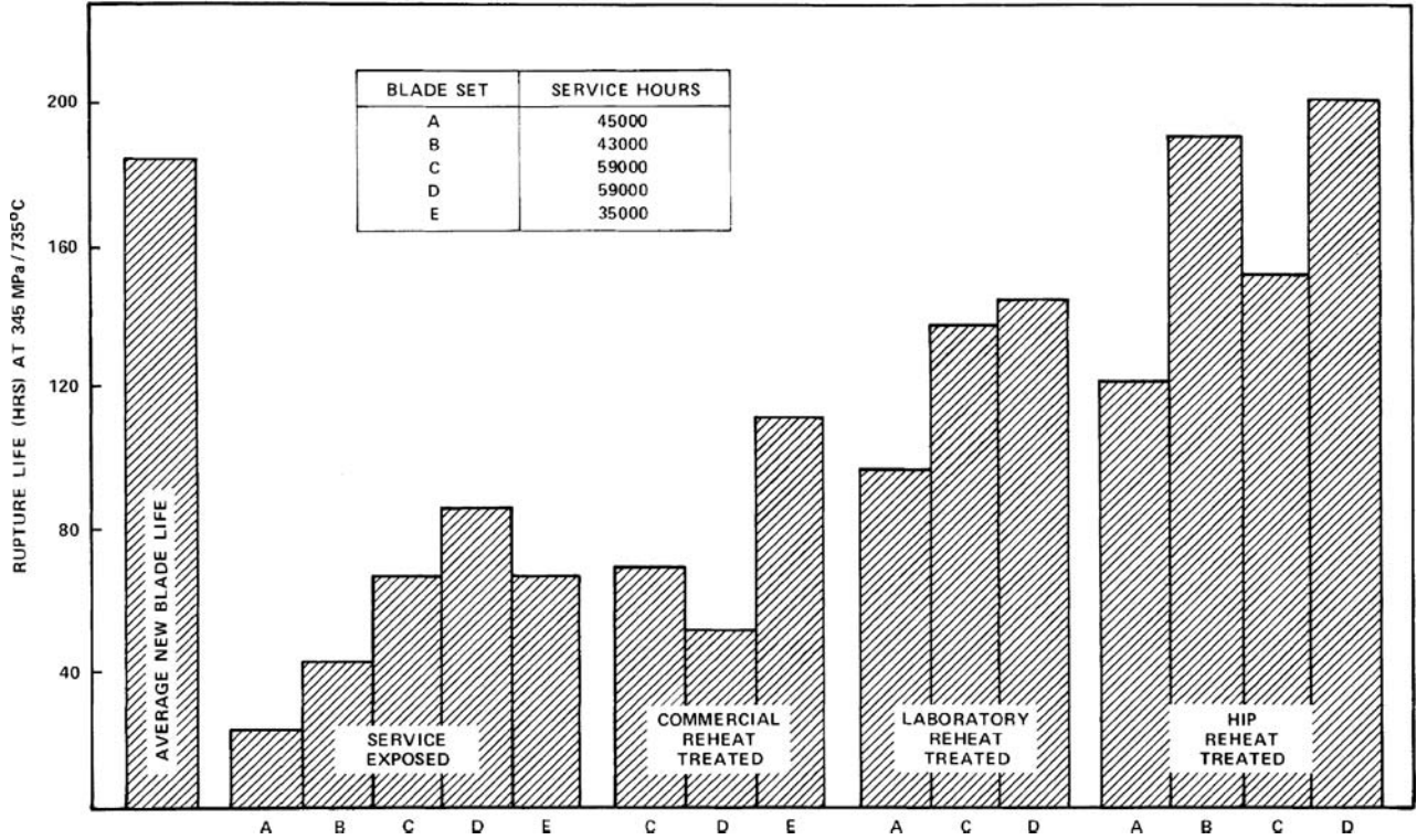
Figure 21-19. Comparison of stress rupture life at 50 ksi/1350°F (345 Mpa/735°C) in service exposed, commercially reheat-treated, laboratory reheat-treated, and HIP reheat-treated used Inconel X-750 turbine blades. (Courtesy of Westinghouse Electric Corp., Gas Turbine Div.)
