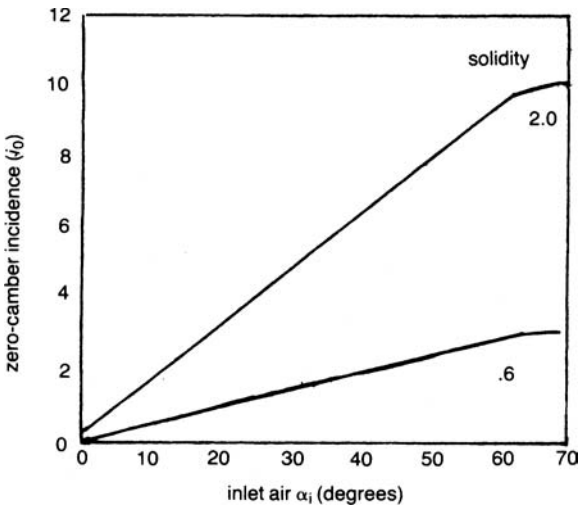
Figure 7-17. Incidence angle for zero-camber airfoil.
