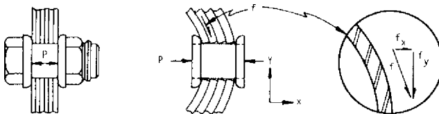
Figure 18-11. Frictional damping in a metal-disc coupling.
