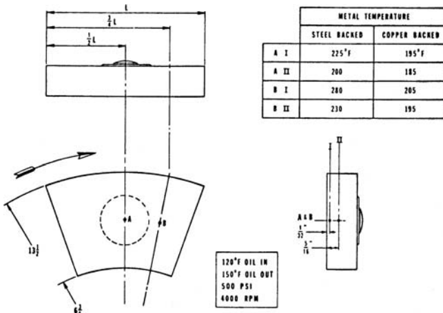
Figure 21-21. Temperature distribution in bearing surfaces.
