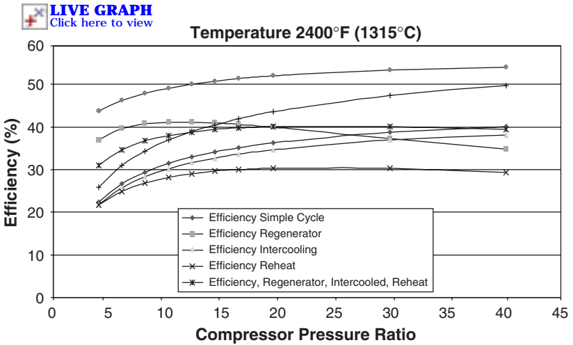
Figure 2-29. Comparison of thermal efficiency of various cycles' temperature.
