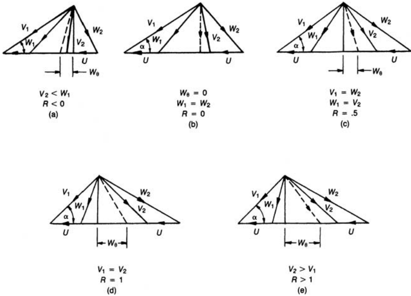
Figure 9-4. Turbine velocity triangles showing the effect of various degrees of reaction.
