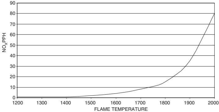
Figure 10-21. Correlation of adiabatic flame temperature with NO x emissions.
