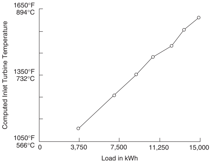
Figure 3-17. Turbine inlet temperature as a function of turbine load.
