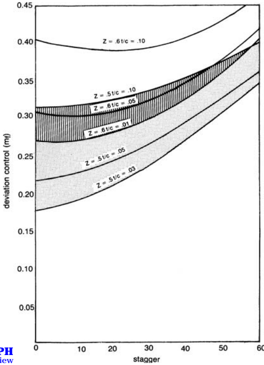
Figure 7-21. Position of maximum thickness effect on deviation.
