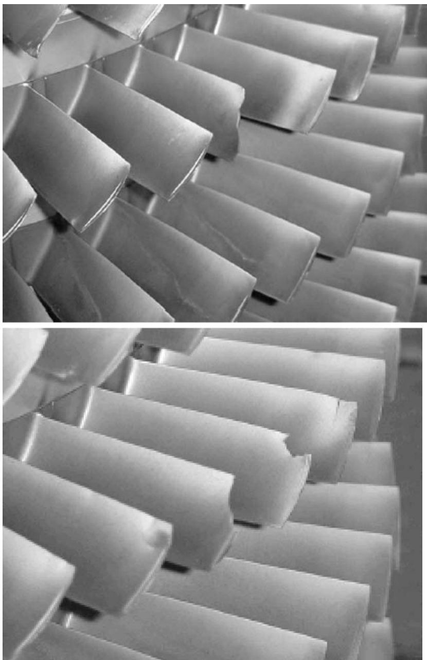
Figure 22-10. Blade failures due to excessive tip rubs.
