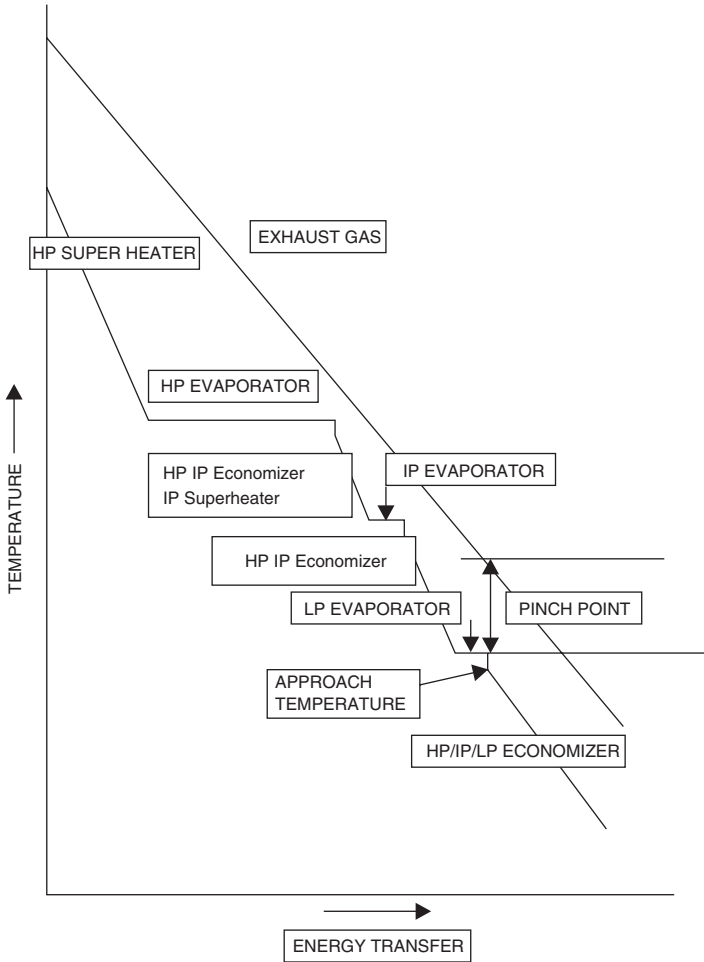
Figure 2-33. Energy/temperature diagram of the triple pressure HRSG.
