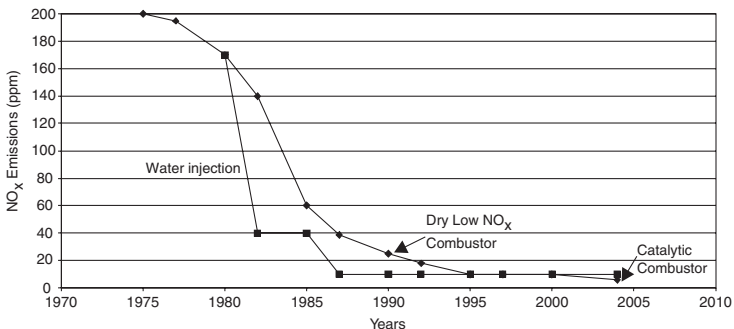
Figure 10-18. Control of gas turbine \text{NO}_x emissions over the years.
