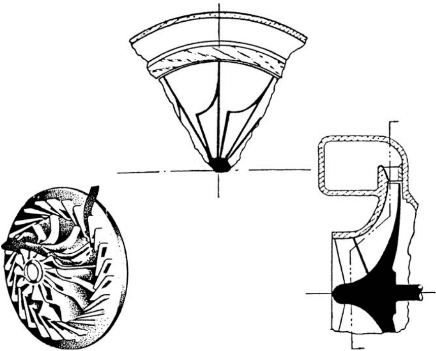
Figure 8-4. Mixed-flow-type radial-inflow turbine.
