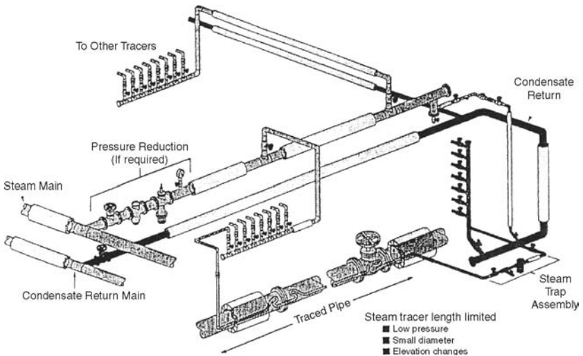
Figure 12-15. Steam tracing system.
