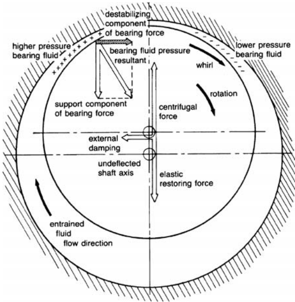
Figure 5-23a. Oil whirl. (Ehrich, F.F., "Identification and Avoidance of Instabilities and Self-Excited Vibrations in Rotating Machinery," Adopted from ASME Paper 72-DE-21, General Electric Co., Aircraft Engine Group, Group Engineering Division, May 11, 1972.)
