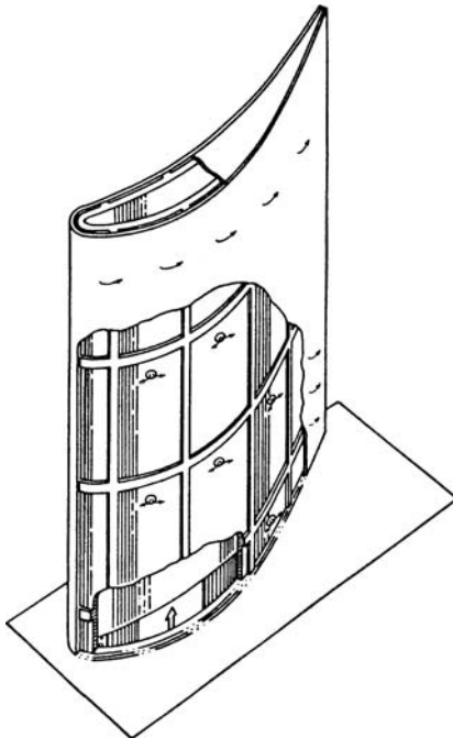
Figure 9-19. Transpiration-cooled blade.
