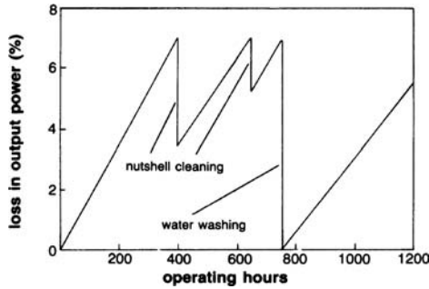
Figure 12-13. Effect of cleaning on power output.
