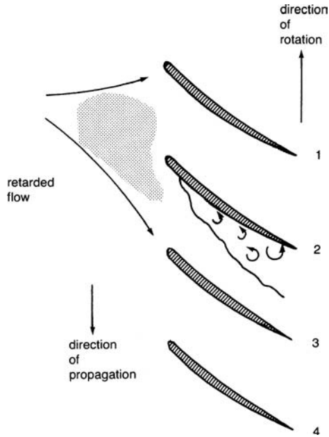
Figure 7-28. Propagating stall in a blade cascade.
