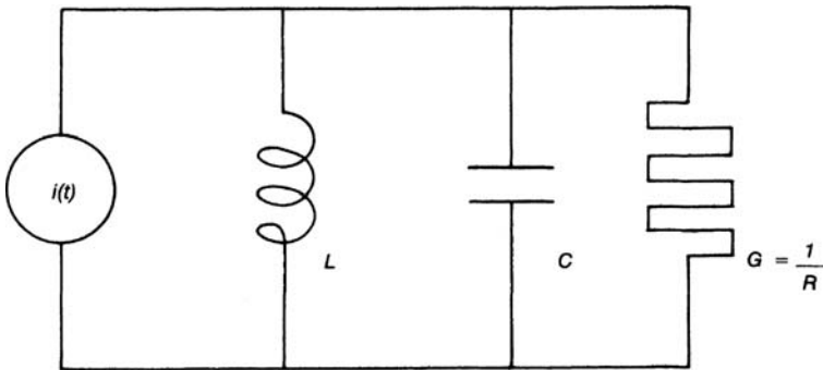
Figure 5-19. Force-current analogy.
