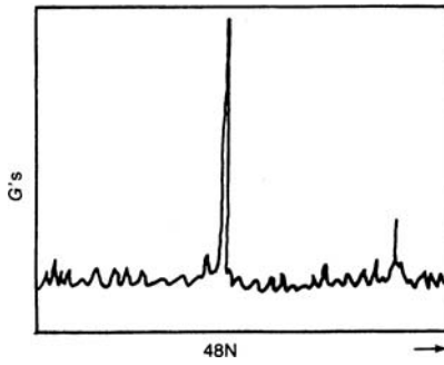
Figure 7-31. High-pressure bleed chamber—5400 rpm.
