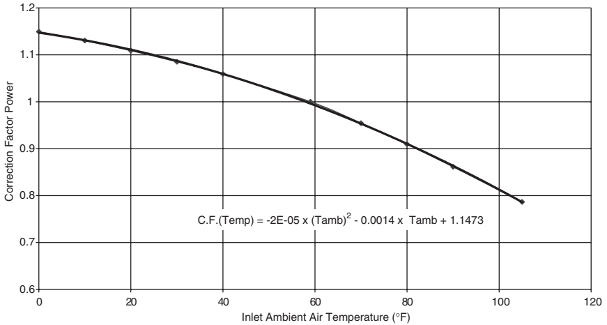
Figure 20-15. Correction factor for power as a function of inlet ambient air temperature.
