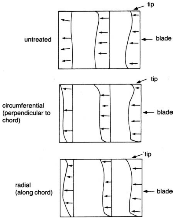
Figure 7-47. Velocity patterns observed in the side view of the blade passage for various casing treatments.
