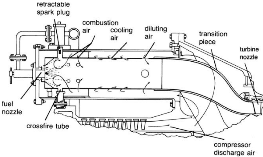
Figure 10-14. Tubo-annular or can-annular combustor for a heavy-duty gas turbine. (Courtesy of General Electric Company.)
