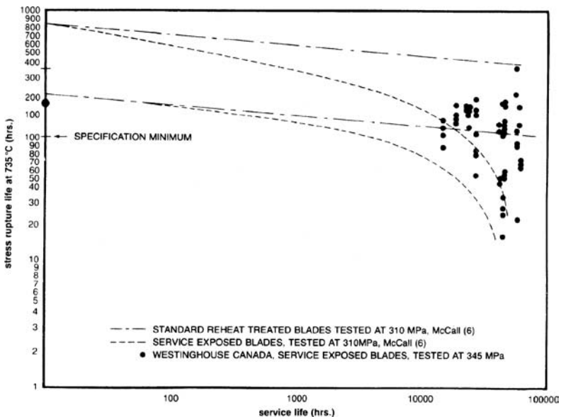
Figure 21-18. The variation of remaining stress rupture life at 1350 °F (735 °C) with service time in forged Inconel alloy X-750 turbine blades. (Courtesy of Westinghouse Electric Corp., Gas Turbine Div.)
