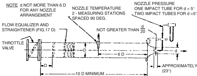
Figure 20-3. Flow nozzle for subcritical flow. (Power Test Code 10, Compressors and Exhausters , American Society of Mechanical Engineers, 1965.)
