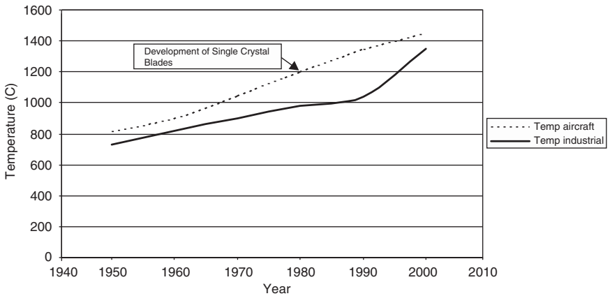
Figure 1-4. Trend in improvement in firing temperature.
