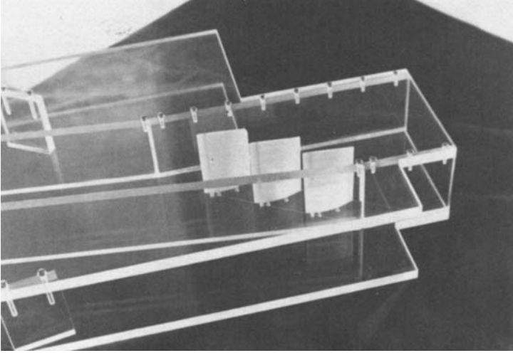
Figure 7-41. Cascade model in axial-flow test tank.
