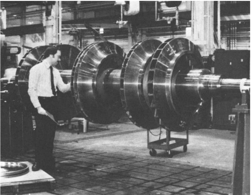
Figure 6-5. Closed impeller. (Courtesy Elliott Company, Jeannette, PA.)
