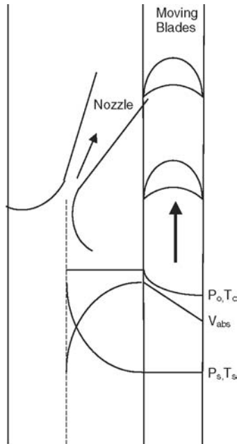
Figure 9-6. Schematic of an impulse turbine showing the variation of the thermodynamic and fluid mechanic properties.
