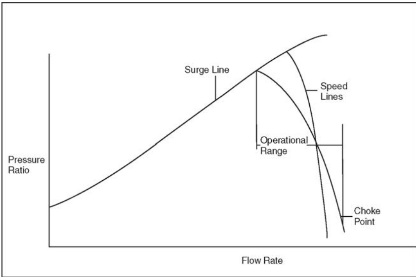
Figure 7-27. A high-pressure multistage axial-flow compressor map.
