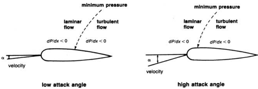
Figure 7-10. Laminar flow airfoils.
