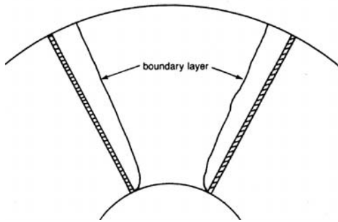
Figure 6-23. Boundary-layer development.
