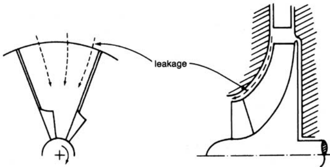
b. shrouded impeller
