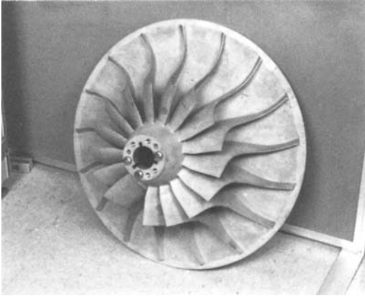
Figure 6-6. Open-faced impeller.
