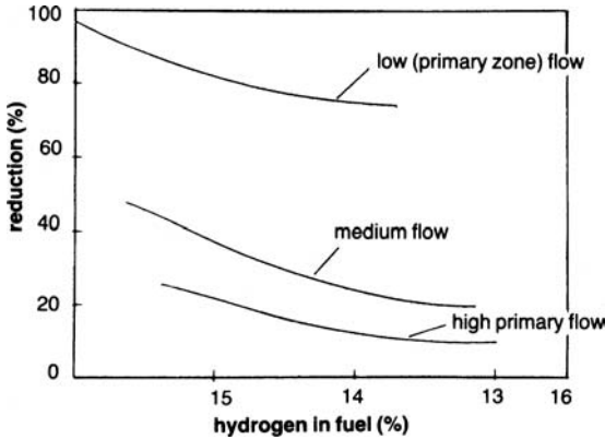
Figure 12-9. Effect of hydrogen saturation in primary flow on smoke.
