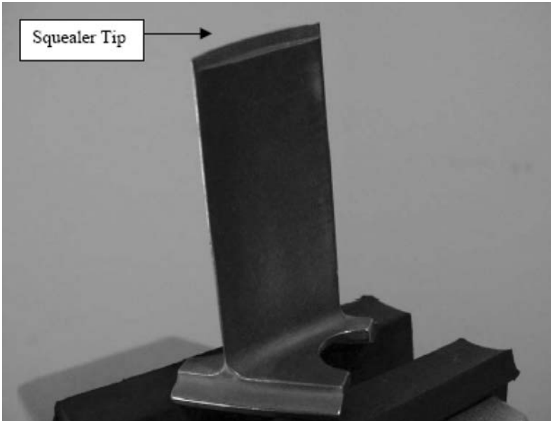
Figure 22-9. Compressor blade showing the blade tip squealer.
