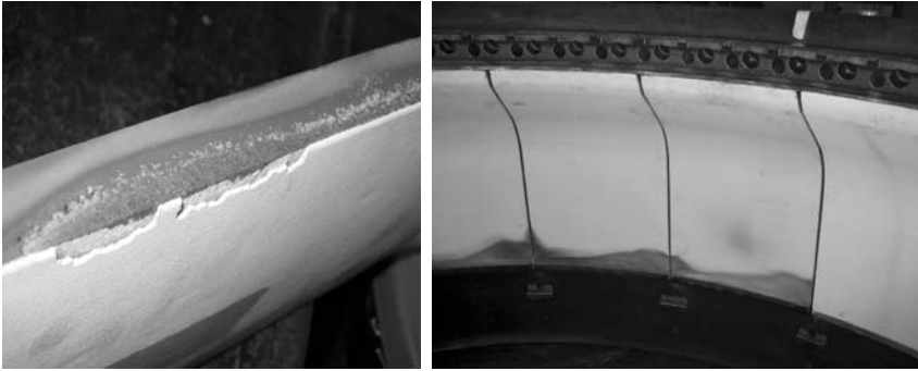
Figure 22-24. Combustor liner plates from an annular combustor.
