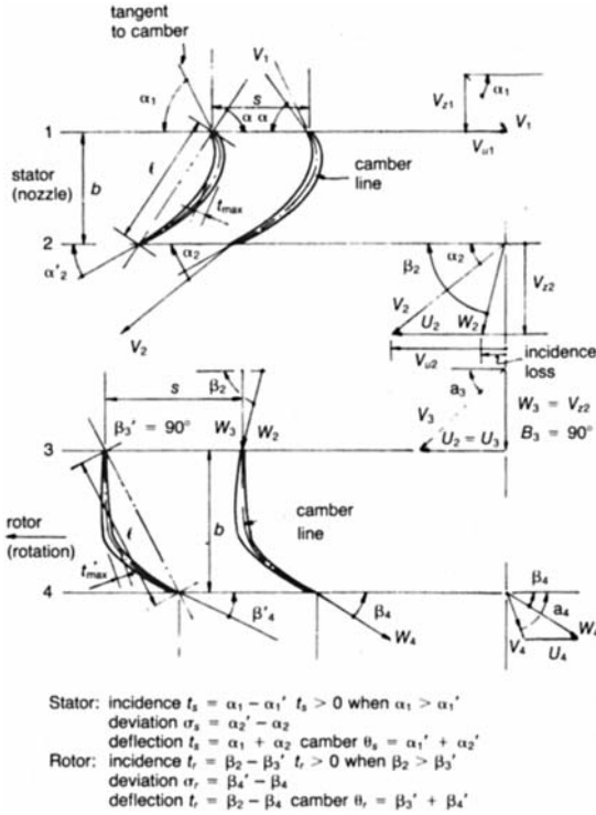
Figure 9-2. Stage nomenclature and velocity triangles.
