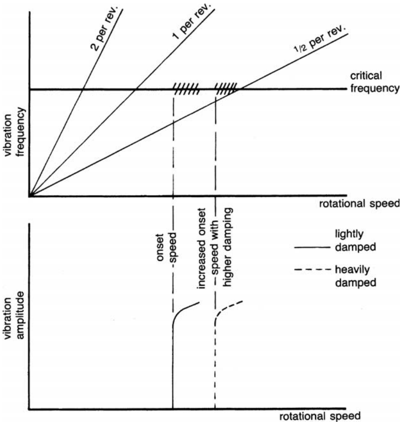
Figure 5-21. Characteristic of instabilities or self-excited vibration in rotating machinery. (Ehrich, F.F., "Identification and Avoidance of Instabilities and Self-Excited Vibrations in Rotating Machinery," Adopted from ASME Paper 72-DE-21, General Electric Co., Aircraft Engine Group, Group Engineering Division, May 11, 1972.)
