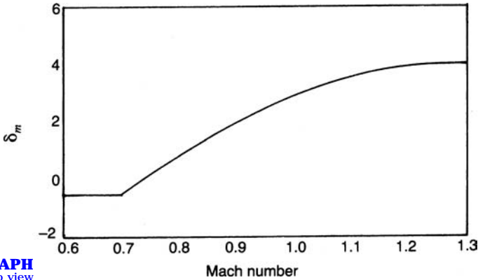
Figure 7-20. Mach-number correction for incidence angle.
