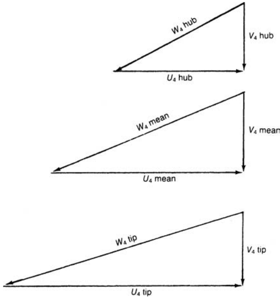
Figure 8-12. Exit velocity diagram for a radial-inflow turbine.
