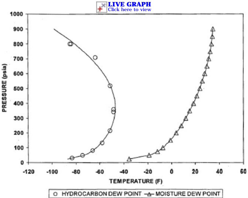
Figure 12-11. Hydrocarbon and moisture dew point.
