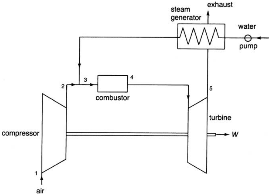
Figure 2-20. The steam injection cycle.
