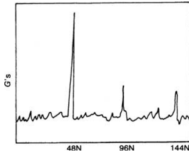
Figure 7-33. High-pressure bleed chamber—9400 rpm.
