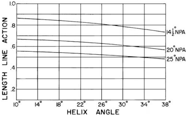
Figure 14-4. Length of line of action change with pressure angle and helix angle. (Courtesy of Lufkin Industries, Inc.)
