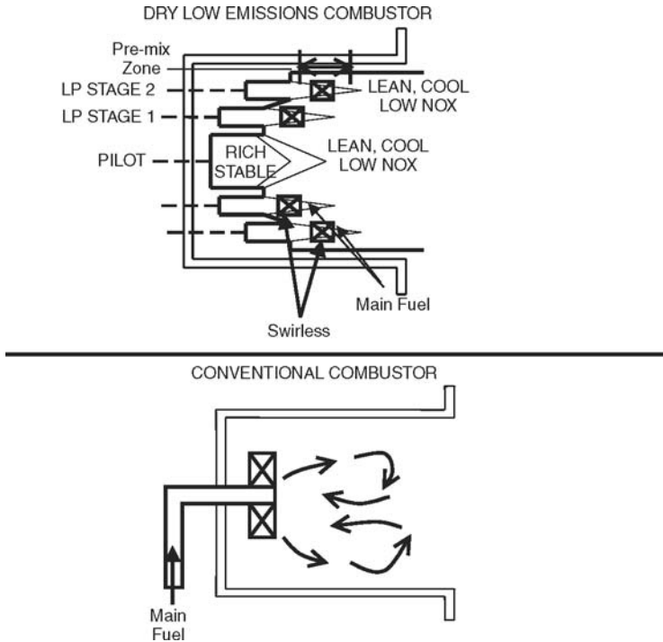
Figure 10-23. A schematic comparison of a typical dry low emission \text{NO}_x combustor and a conventional combustor.
