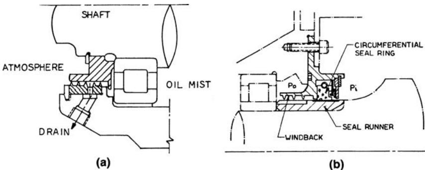
Figure 13-23. Windback seal.
