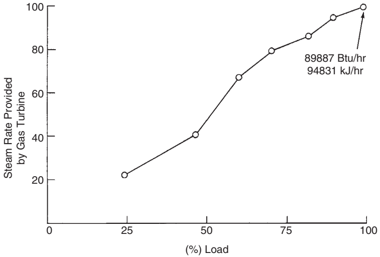
Figure 3-21. Steam generated by exhaust gases of gas turbine as a function of gas turbine load.
