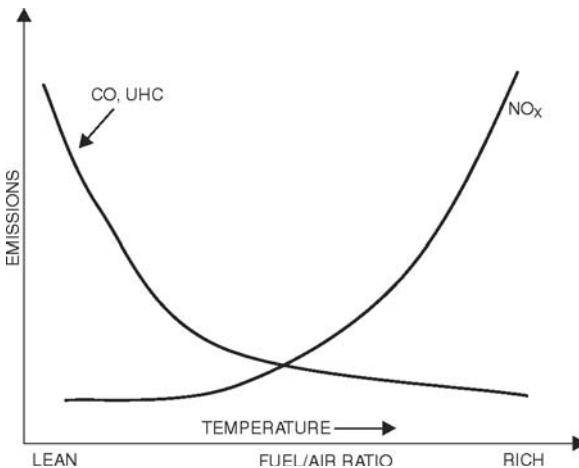
Figure 10-20. The effect of flame temperature on emissions.
