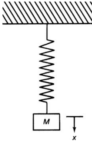
Figure 5-1. System with single degree of freedom.
