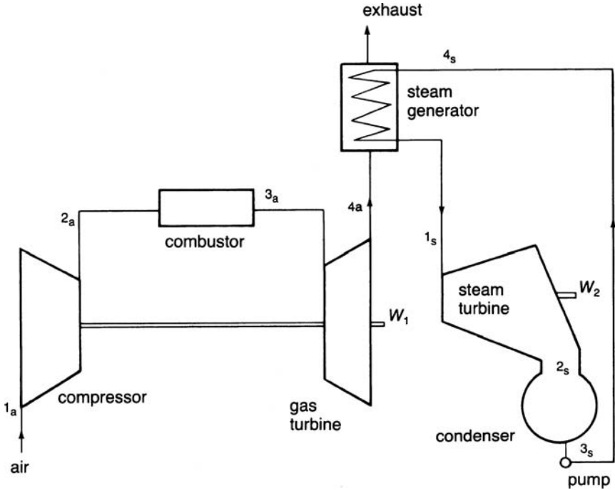
Figure 2-26. The Brayton-Rankine combined cycle.
