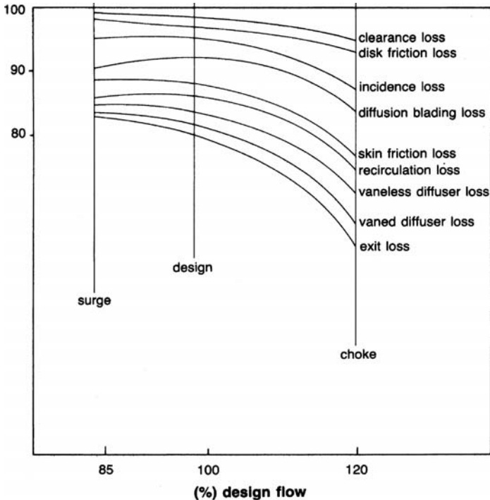
Figure 6-35. Losses in a centrifugal compressor.
