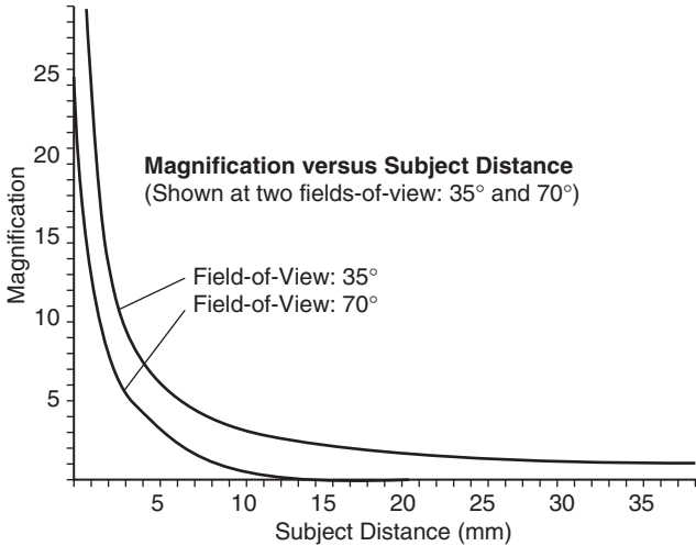
Figure 21-7. Borescope magnification.
