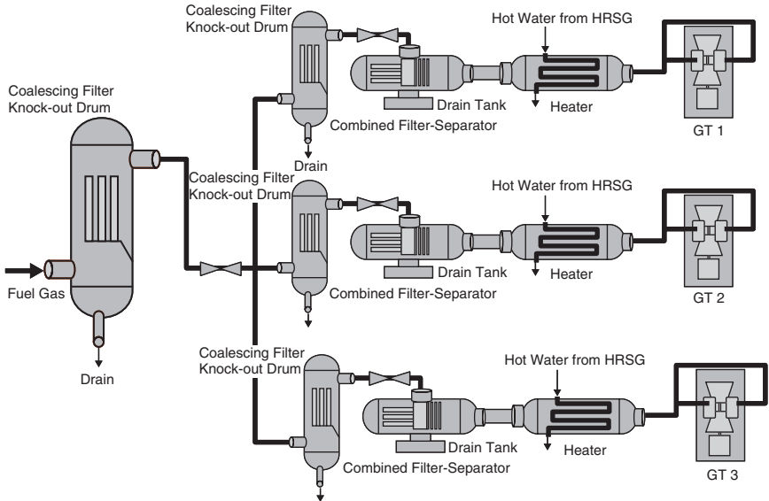
Figure 12-12. Natural gas fuel handling system.
