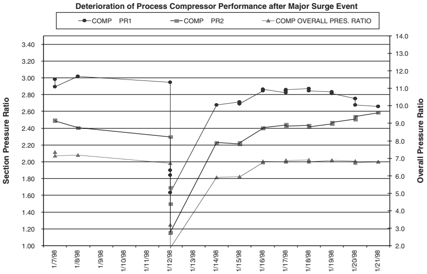
Figure 22-14. Deterioration of the axial-flow compressor.
