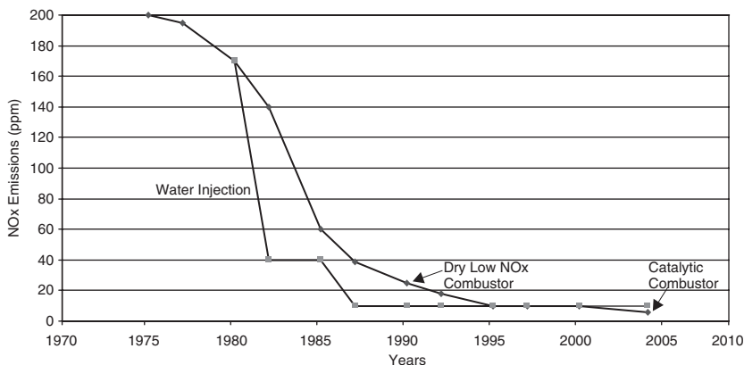
Figure 1-33. Control of gas turbine NO x emission over the years.
