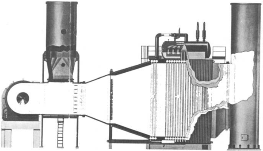
Figure 1-41. Supplementary fired exhaust gas steam generator.
