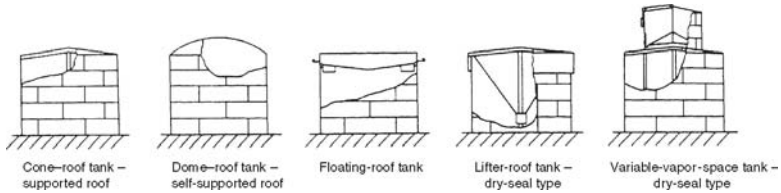
Figure 12-17. Some types of atmospheric storage tanks.
