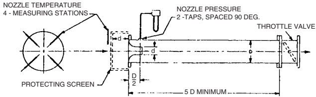
Figure 20-5. Flow nozzle for exhausters. (Power Test Code 10, Compressors and Exhausters , American Society of Mechanical Engineers, 1965.)
