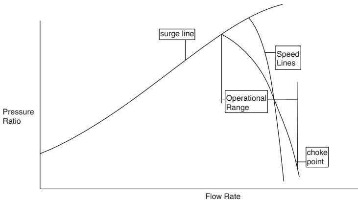
Figure 19-18. Performance map of an axial-flow compressor used in most gas turbines.
