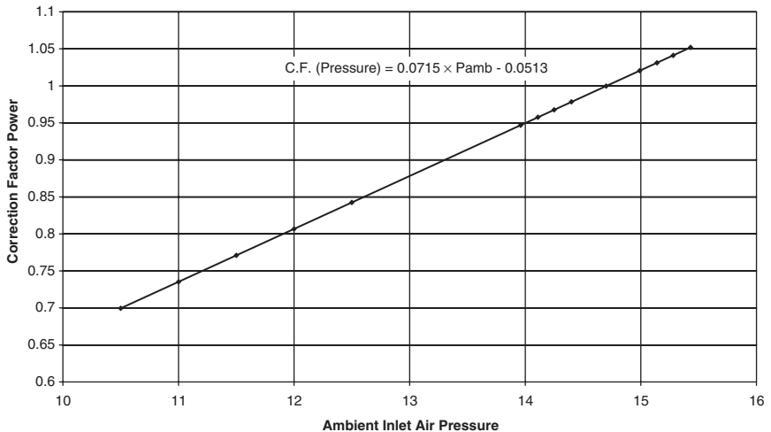
Figure 20-14. Correction factor for power as a function of inlet ambient pressure.
