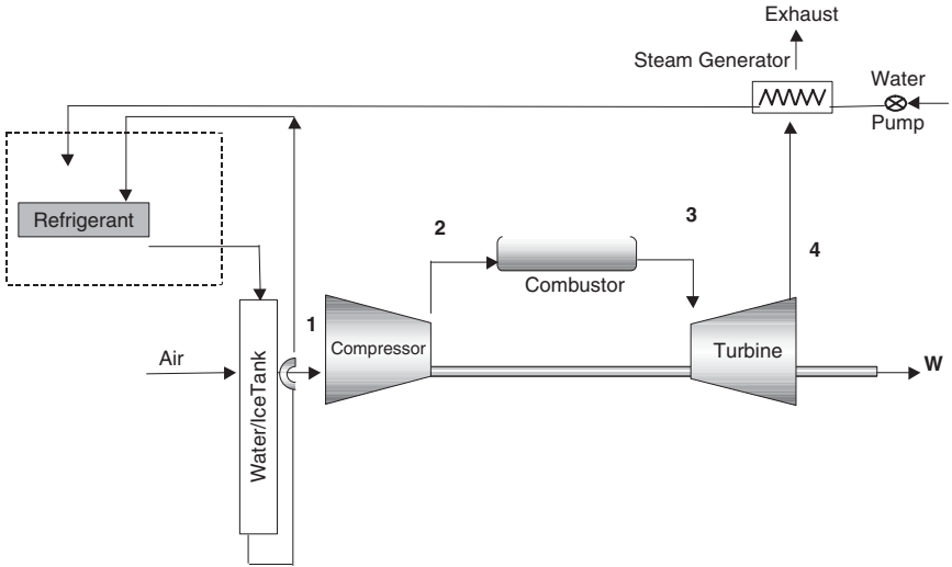
Figure 2-39. Thermal storage inlet system.
