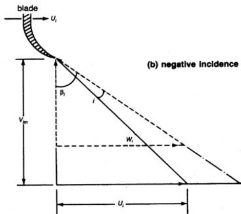
Figure 6-31. Inlet velocity triangle at nonzero incidents.
