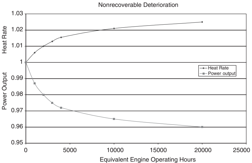
Figure 21-11. Nonrecoverable losses in a gas turbine as a function of equivalent operating hours.
