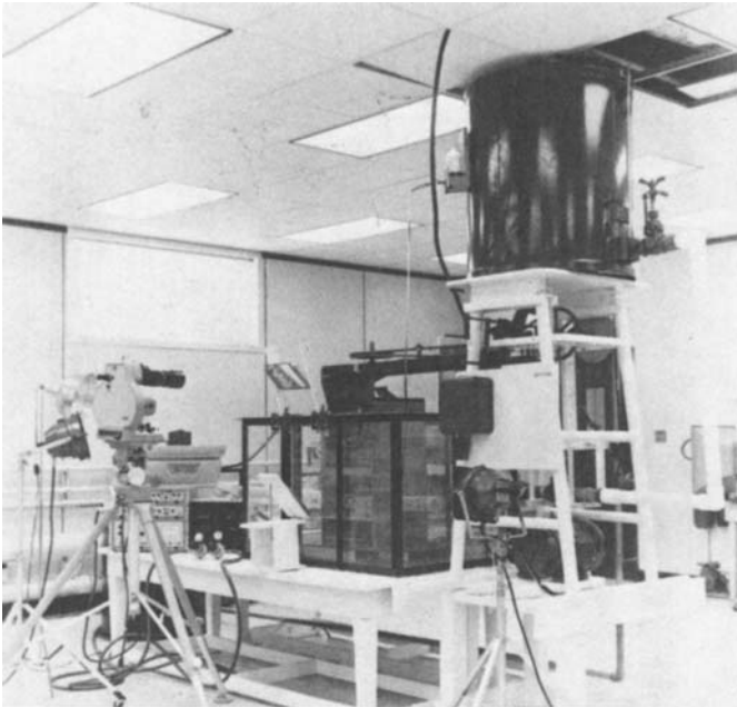
Figure 7-42. Apparatus for testing axial-flow cascade model.
