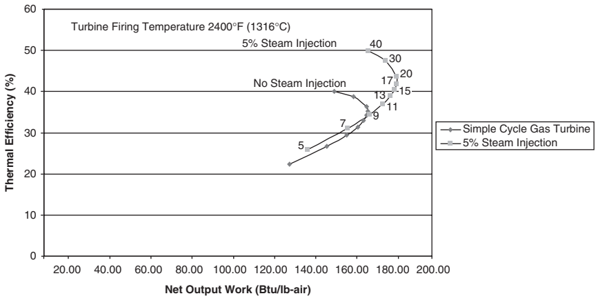
Figure 2-21. Comparison between 5% steam injection and simple-cycle gas turbine.
