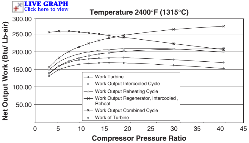
Figure 2-28. Comparison of net work output of various cycles' temperature.
