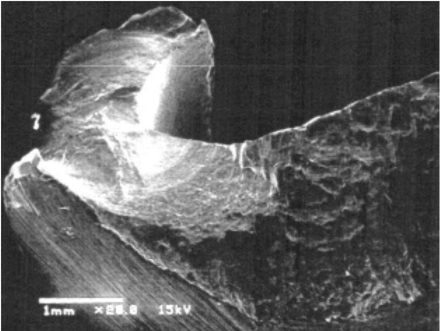
Figure 22-16. Electron microscope photograph of the first-stage failed blade.
