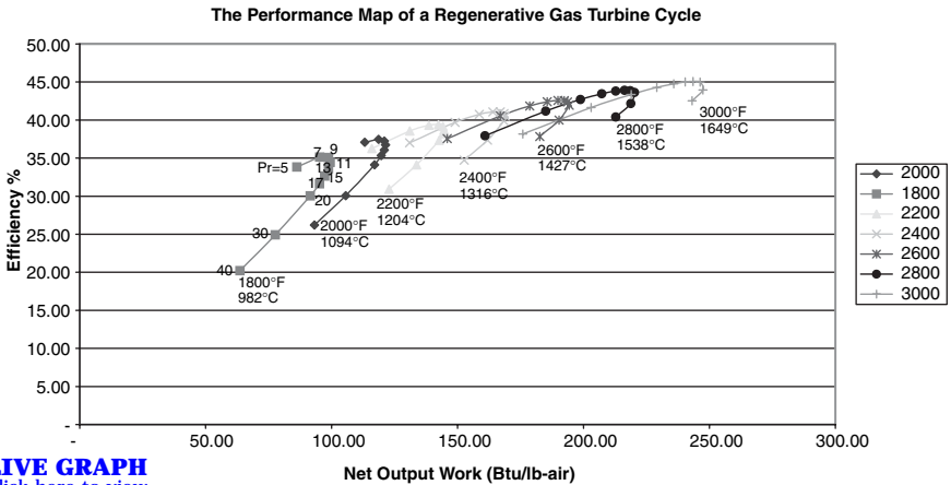
Figure 1-7. Performance map of a regenerative gas turbine.
