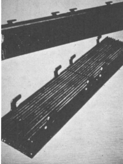
Figure 10-12a. Top view of a large side combustor with special tiles. (Courtesy Brown Boveri Turbomachinery, Inc.)
