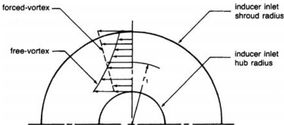
Figure 6-13. Prewhirl distribution patterns.
