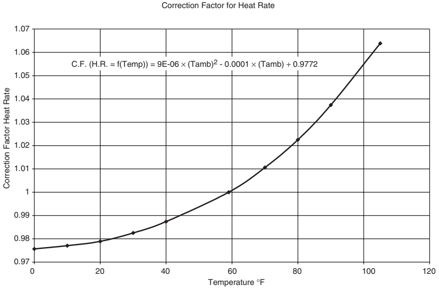
Figure 20-16. Correction factor for heat rate as a function of inlet ambient air temperature.
