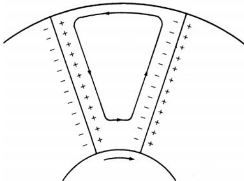
Figure 6-22. Coriolis circulation.
