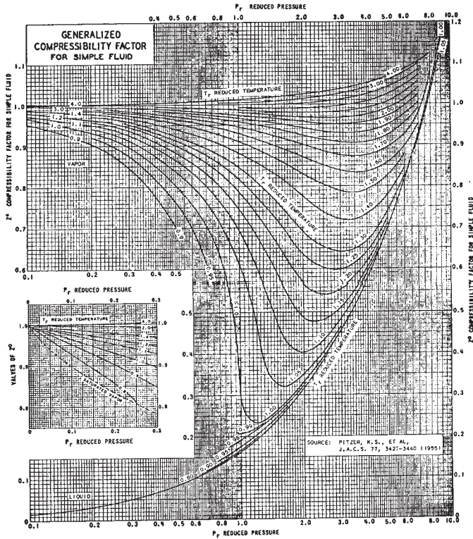
Figure 3-1. Generalized compressibility factor for simple fluid. (Adapted with permission from Journal of the American Chemical Society , © 1955, American Chemical Society.)
