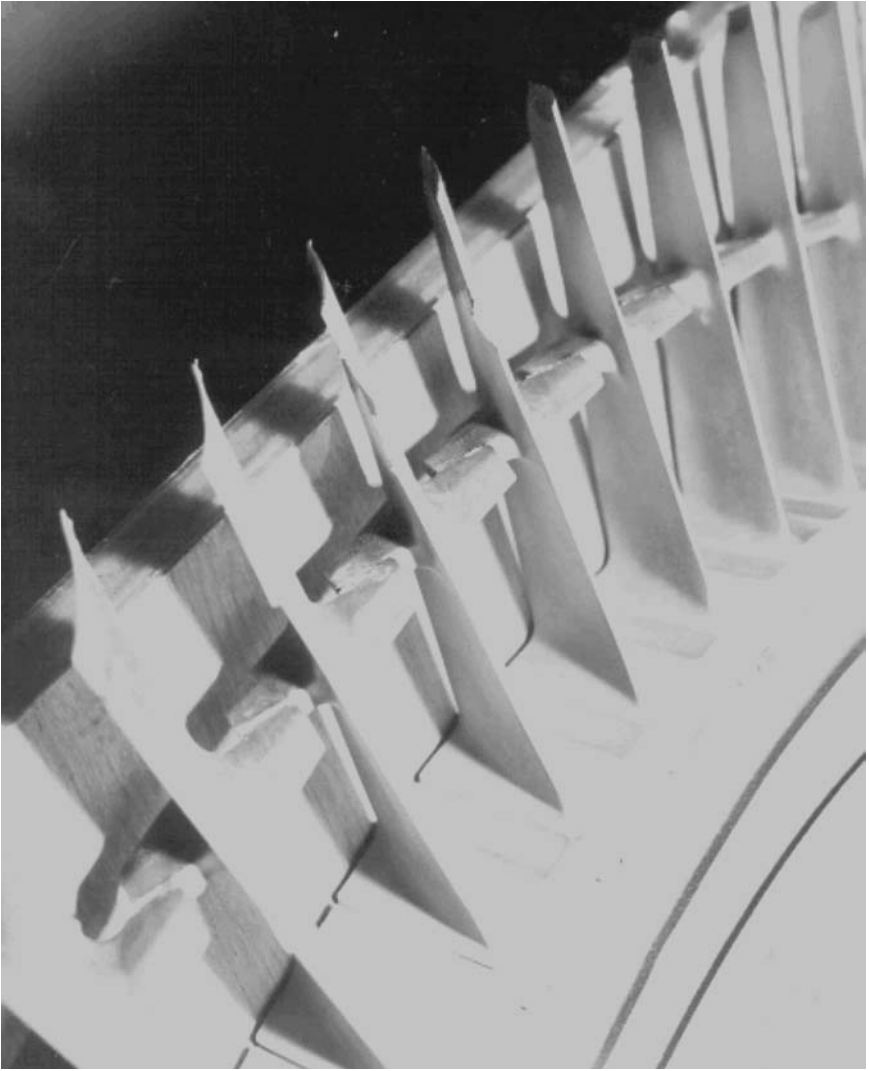
Figure 22-6. Mid-span shrouds on compressor blades.
