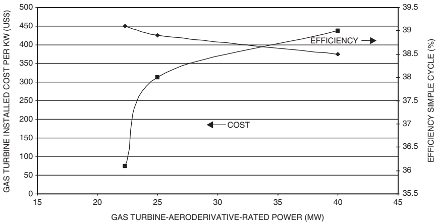
Figure 4-4. Installed cost and efficiency of aero-derivative type turbines.
