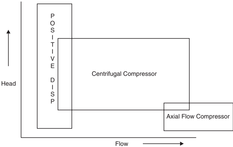
Figure 1-17. Performance characteristics of different types of compressors.
