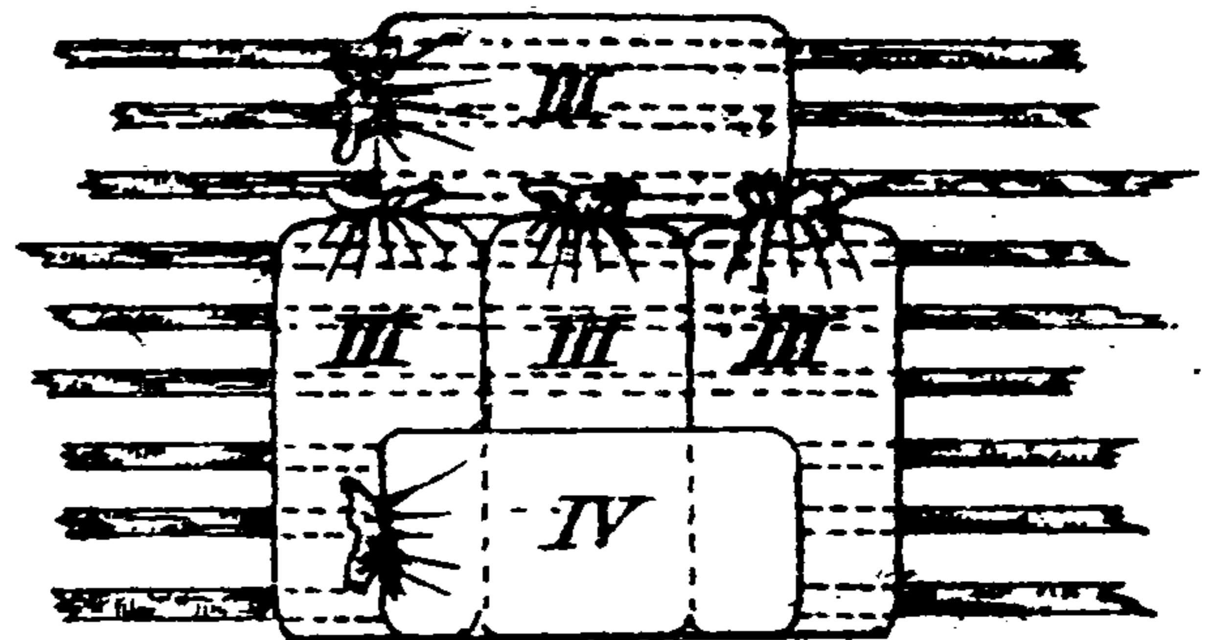
PLAN OF III & IV COURSES
