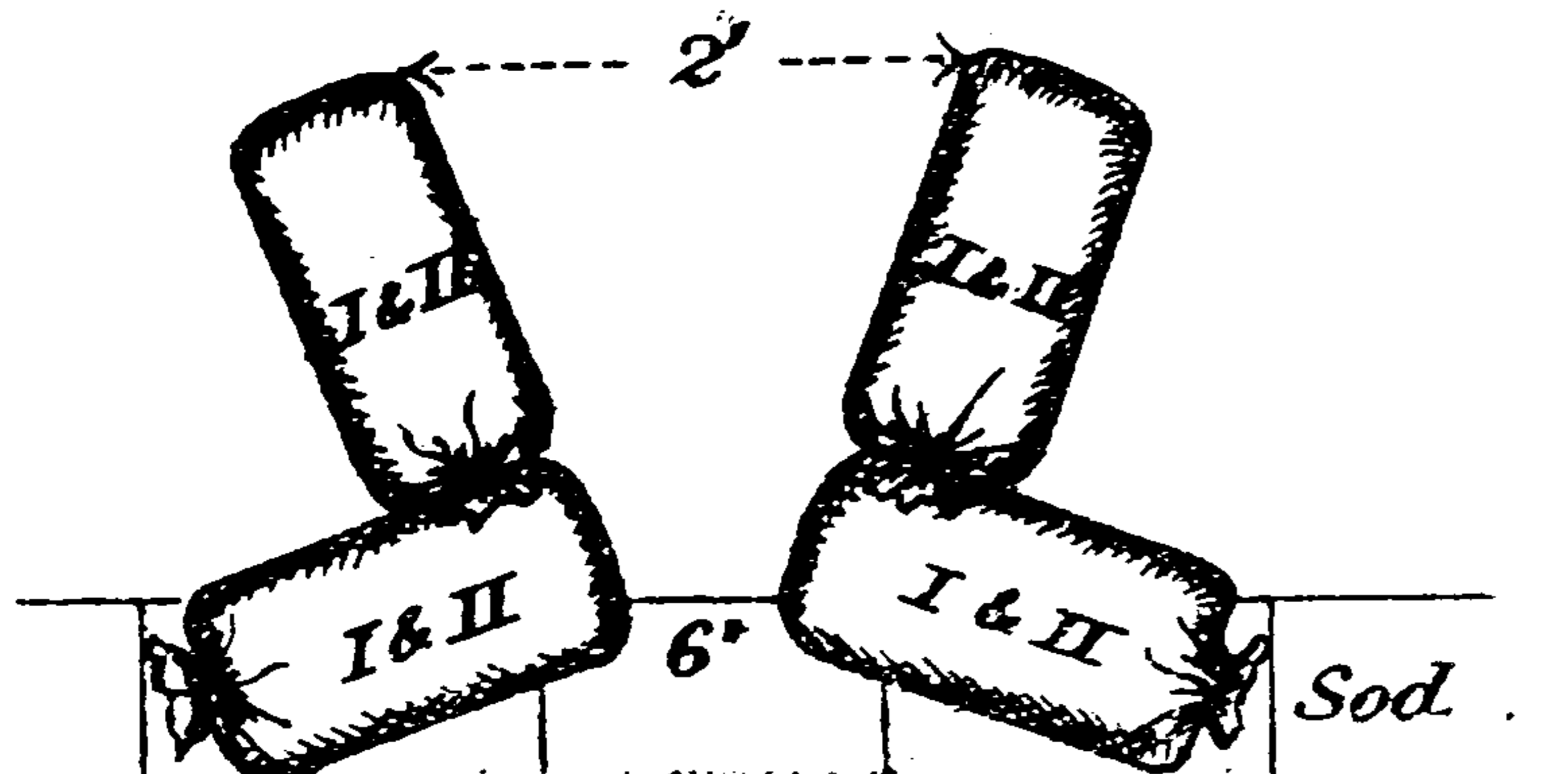
PLAN OF I & II COURSES
