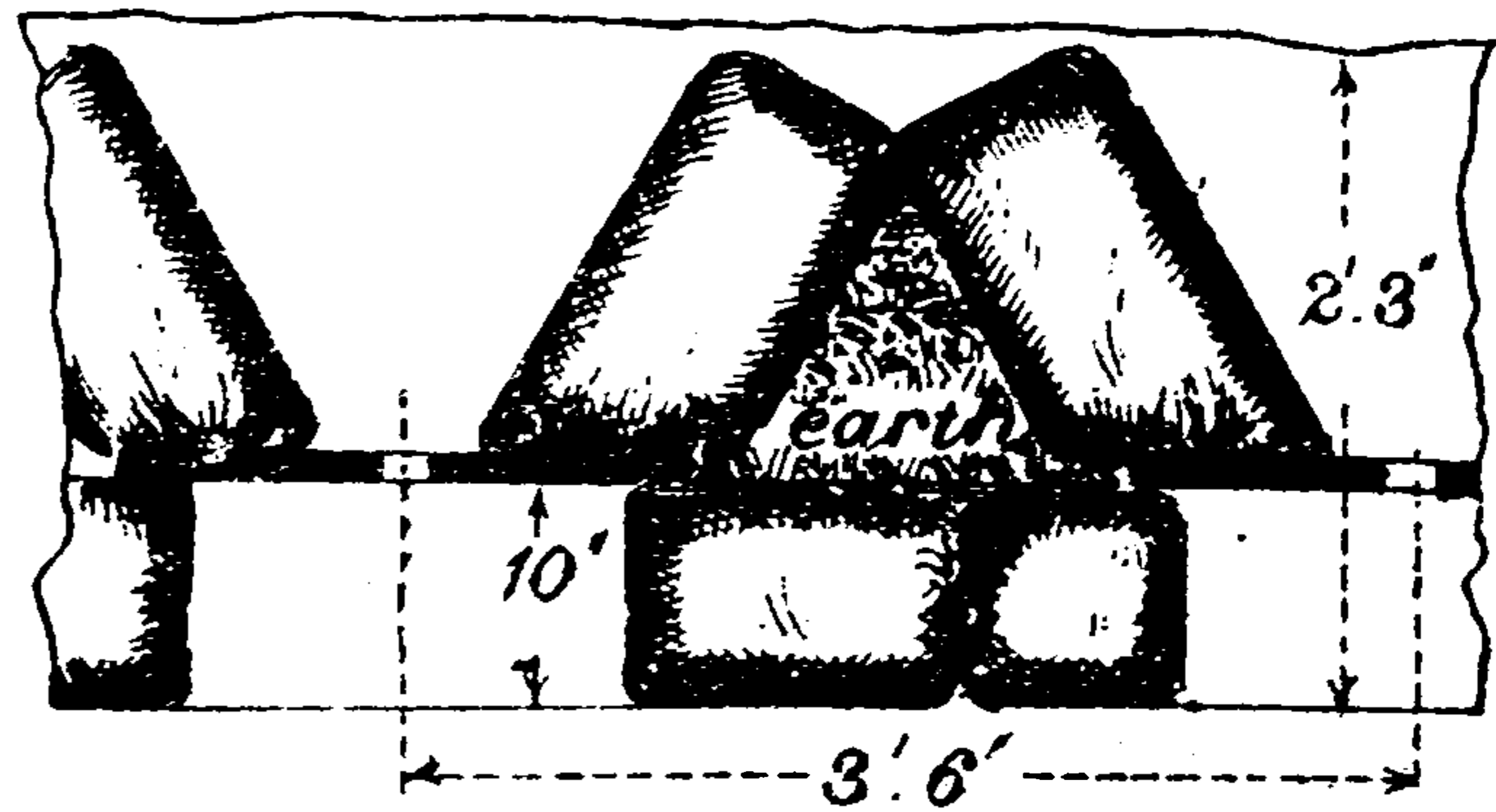
PLAN
