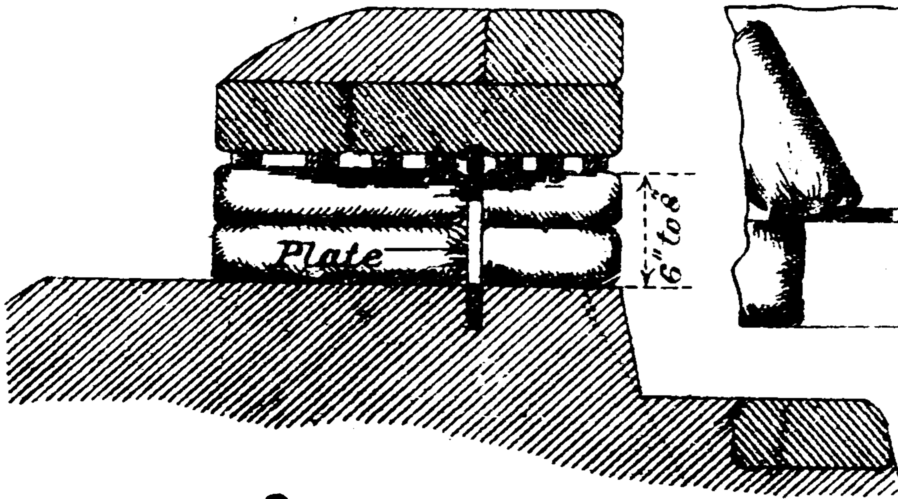
SECTION
