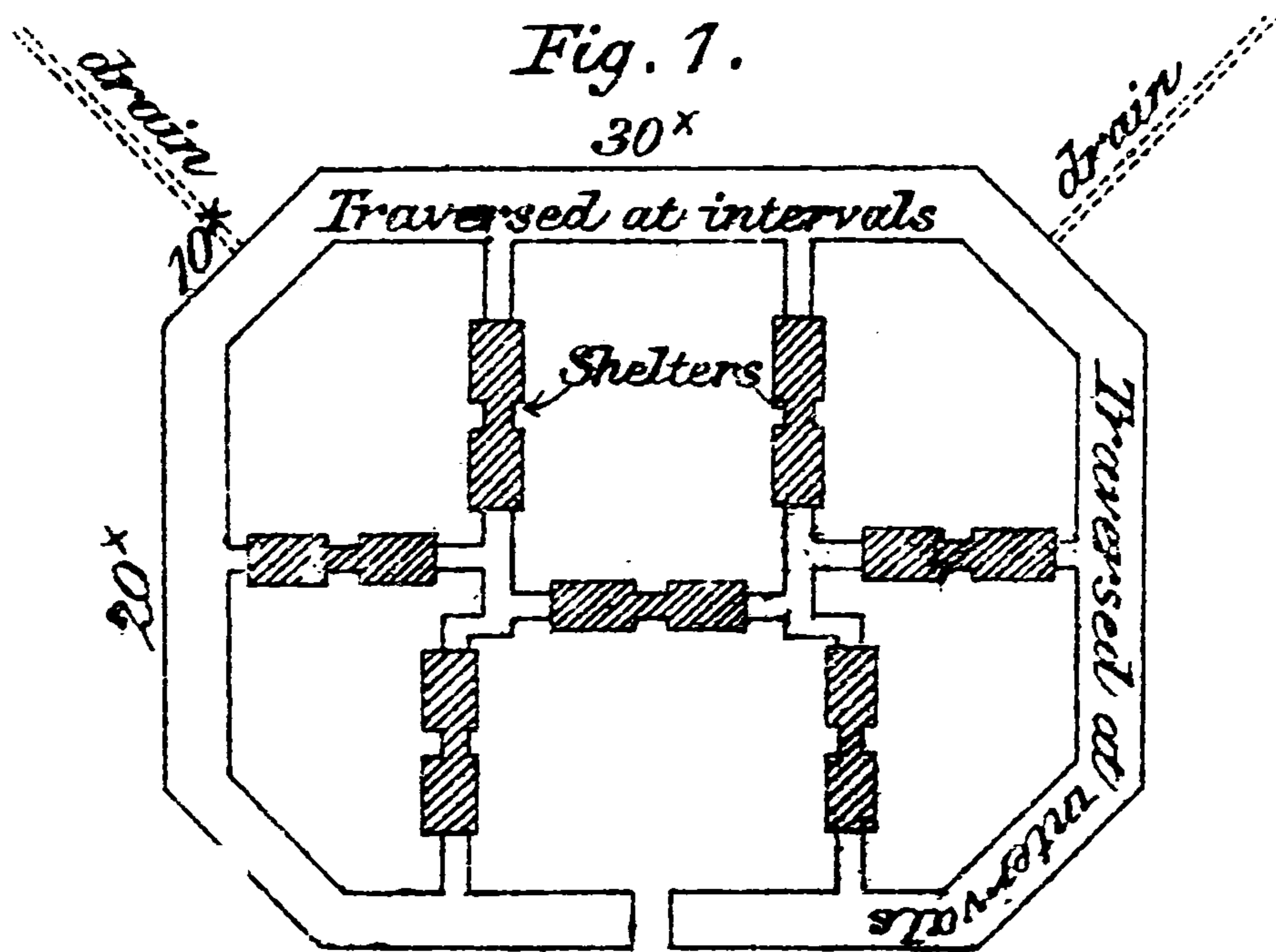
General Plan
