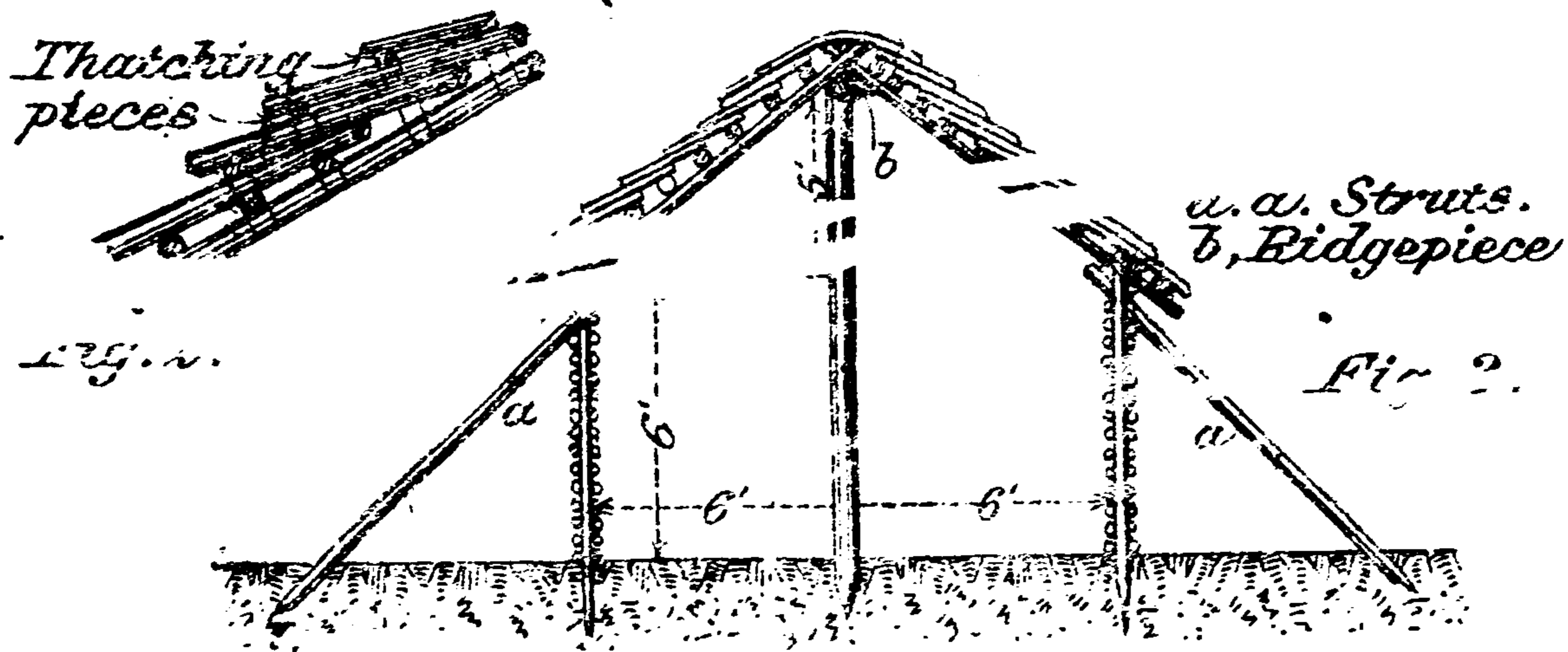
Details of Thatching see Fig. 8.
