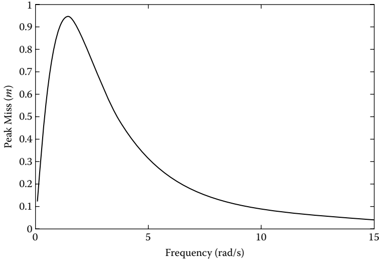
FIGURE 4.7 Peak miss distance for 1-g target maneuver amplitude.
