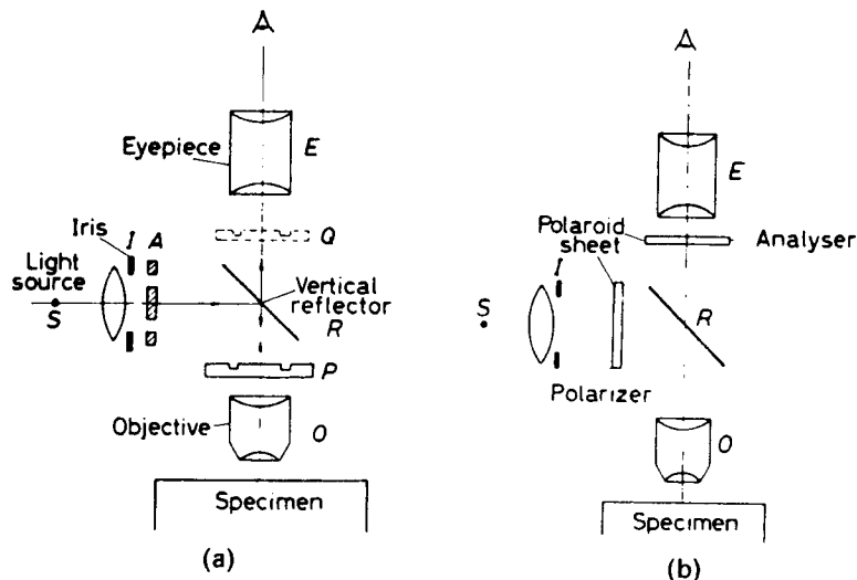
Figure 5.4 Schematic arrangement of microscope system for (a) phase-contrast and (b) polarized light microscopy.
