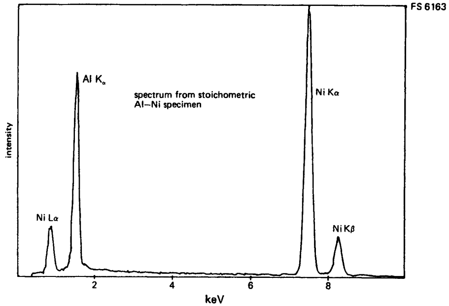
Figure 5.35 EDX spectrum from a stoichiometric Ni-Al specimen.
