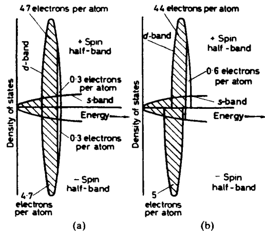
Figure 6.32 Schematic representation of (a) paramagnetic nickel and (b) ferromagnetic nickel (after Raynor, 1958; by courtesy of Inst. of Materials).
