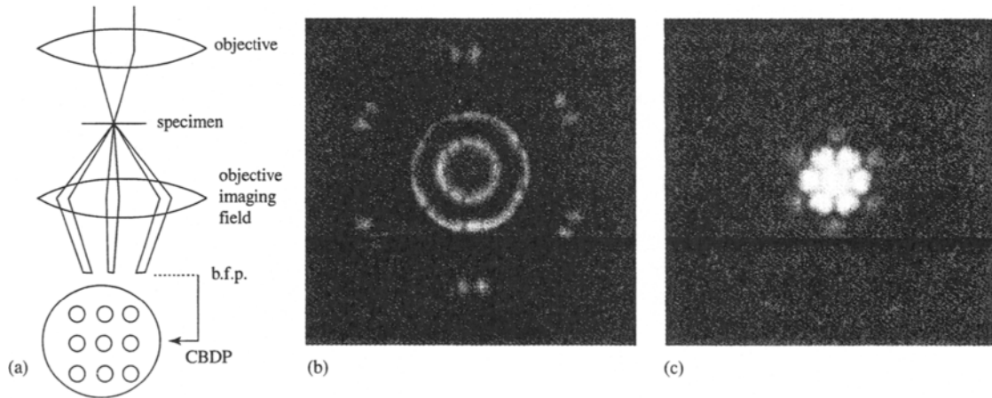
Figure 5.31 (a) Schematic formation of convergent beam diffraction pattern in the backfocal plane of the objective lens, (b) and (c) (1 1 1) CBDPs from Si; (b) zero layer and HOLZ (Higher Order Laue Zones) in direct beam and (c) zero layer + FOLZ (First Order Laue Zones).
