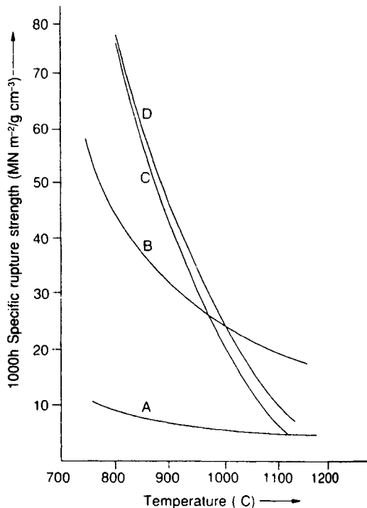
Figure 9.10 Comparison of MA 6000 with other high-strength nickel alloys: (A) TD-Nickel, (B) MA 6000, (C) directionally-solidified Mar-M200 and (D) single-crystal PWA 454.
