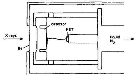
Figure 5.34 Schematic diagram of Si-Li X-ray detector.
