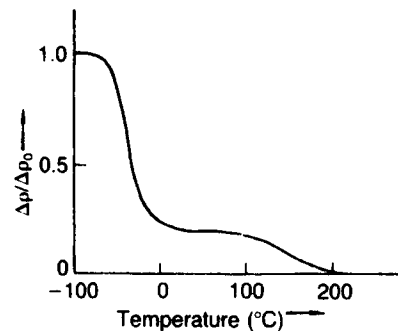
Figure 4.8 Variation of quenched-in resistivity with temperature of annealing for aluminium (after Panseri and Federighi, 1958, 1223).
