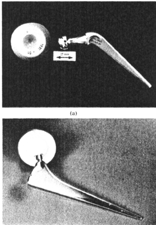
Figure 13.5 (a) Conventional hip joint made of stainless steel and UHMWPE acetabular cup (courtesy R. Grimer, Royal Orthopaedic Hospital, Birmingham). (b) Modular artificial hip made of titanium stem, alumina head and UHMWPE acetabular cup (courtesy P. Marquis, Dental School, Birmingham).
