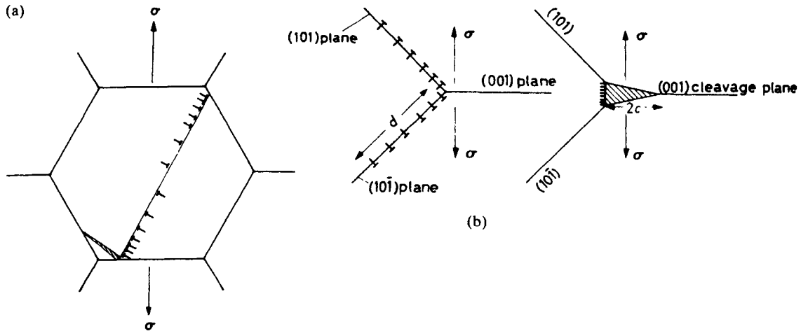
Figure 8.33 Formation of a crack (a) by the piling up of dislocations against a grain boundary after strain and (b) by the dislocations on (101) and (10\bar{1}) planes running together (after Cottrell, 1958, p. 192).
