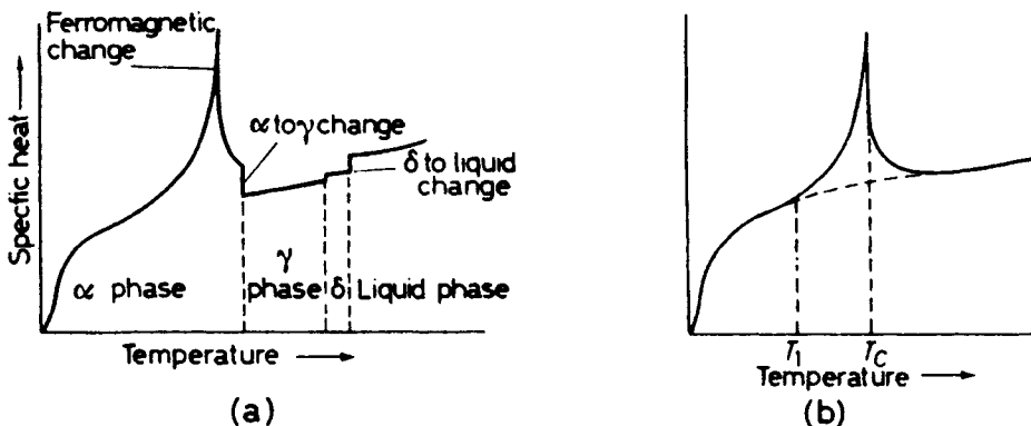
Figure 6.4 The effect of solid state transformations on the specific heat-temperature curve.
