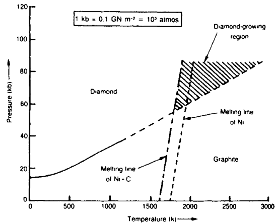
Figure 10.14 Pressure versus temperature diagram for carbon (after Bovenkerk et al., 1959, pp. 1094–8).
