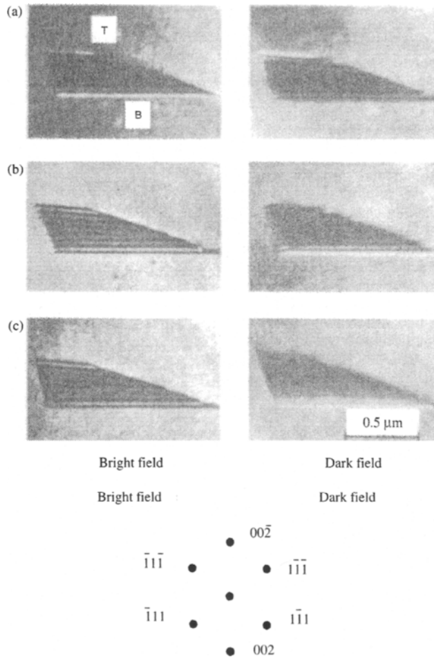
Figure 5.43 Bright-field and dark-field micrographs of an intrinsic stacking fault in a copper–aluminium alloy; the operating diffraction vectors are (a) \bar{1}11 (b) 1\bar{1}\bar{1} and (c) \bar{1}\bar{1}\bar{1} (after Howie and Valdre, 1963; courtesy of Taylor and Francis).
