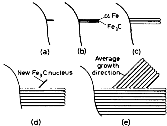
Figure 8.20 Nucleation and growth of pearlite nodules. (a) Initial Fe_3C nucleus; (b) Fe_3C plate full grown, \alpha -Fe now nucleated; (c) \alpha -Fe plates now full grown, new Fe_3C plates nucleated; (d) Fe_3C nucleus of different orientation forms and original nodule grows; (e) new nodule at advanced stage of growth (after Mehl and Hagel; courtesy of Pergamon Press).
