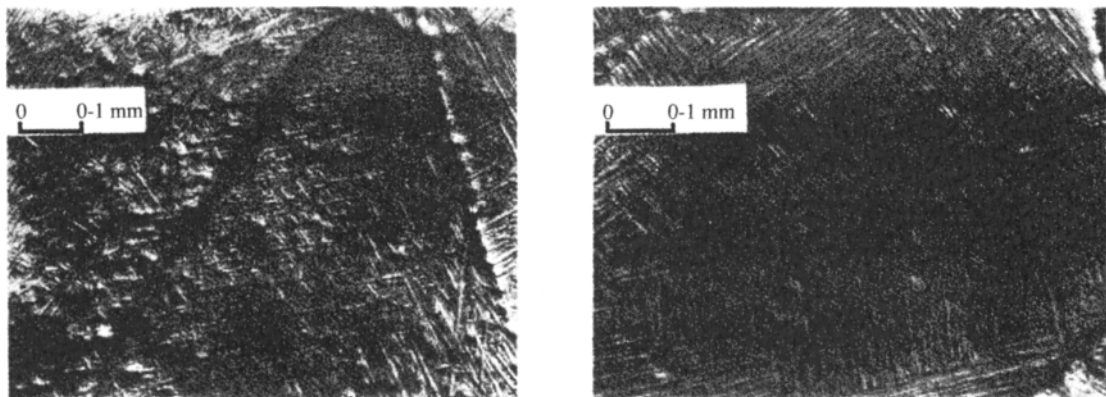
Figure 9.13 Microstructure of near- \alpha titanium alloy ( IMI 829 ) initially \beta -heat-treated at 1050°C for 1 h. (a) Oil quenched and (b) air cooled (after Woodfield, Loretto and Smallman, 1988).
