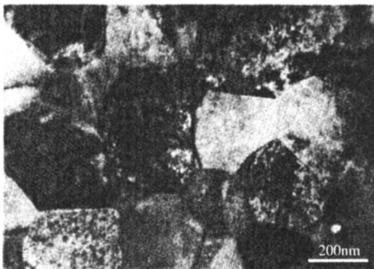
Figure 10.8 Electron micrograph of tetragonal-zirconia polycrystal stabilized with 3 mol.% yttria (with acknowledgement to M. G. Cain, Centre for Advanced Materials Technology, University of Warwick, UK).
