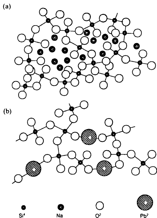
Figure 2.22 Schematic representation of action of modifiers in silica glass. (a) \text{Na}_2\text{O} breaking-up network; (b) \text{PbO} entering network.
