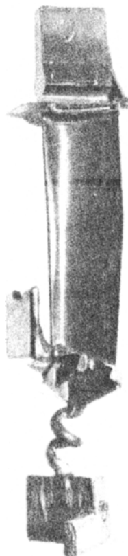
Figure 3.6 A single-crystal blade embodying a DS-starter block and helical constriction and a test plate facilitating orientation check by XRD.
