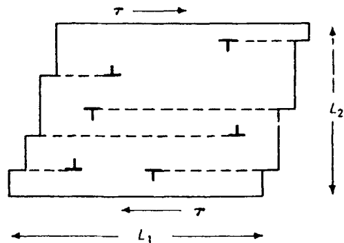
Figure 7.20 Shear produced by gliding dislocations.
