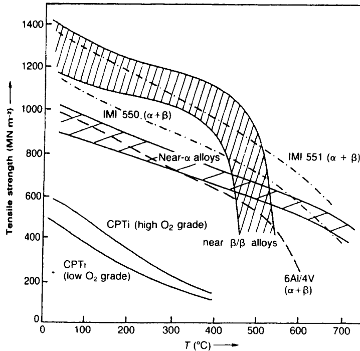
Figure 9.14 Variation of tensile strength with temperature for a range of commercial titanium alloys.
