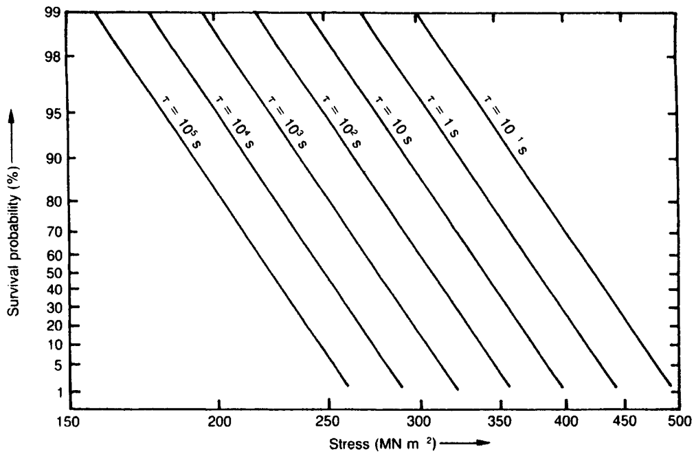
Figure 10.23 Strength-probability-time diagram for alumina derived from bend tests at 293 K: the lifetime \tau of 10^5 s is regarded as a tentative stress-corrosion limit (after Davidge, 1986, p. 145; by courtesy of Cambridge University Press).
