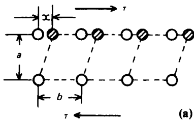
Figure 4.10 Slip of crystal planes (a); shear stress versus displacement curve (b).
