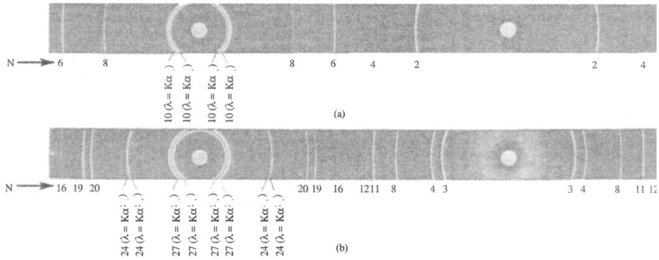
Figure 5.12 Powder photographs taken in a Philips camera (114 mm radius) of (a) iron with cobalt radiation using an iron filter and (b) aluminium with copper radiation using a nickel filter. The high-angle lines are resolved and the separate reflections for \lambda = K\alpha_1 and \lambda = K\alpha_2 are observable..
