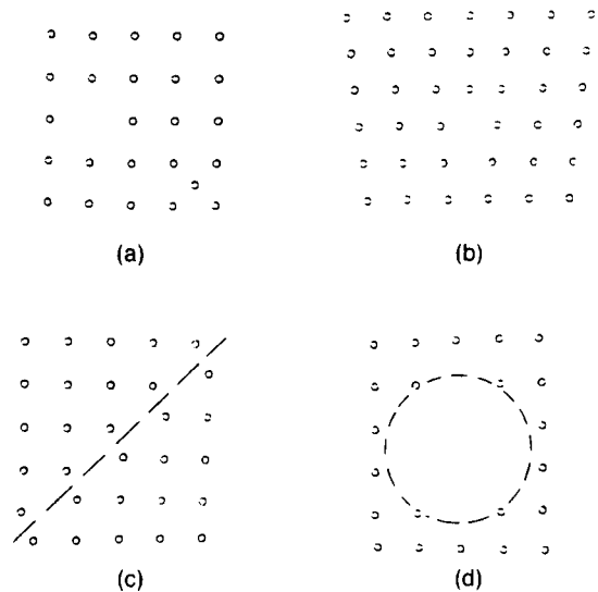
Figure 4.1 (a) Vacancy-interstitial, (b) dislocation, (c) stacking fault, (d) void.
