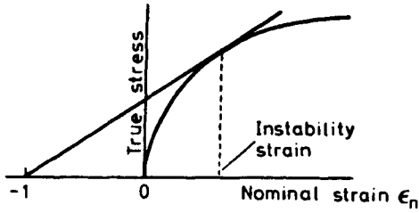
Figure 7.2 Considère's construction.
