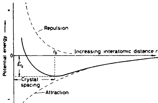
Figure 6.2 Variation in potential energy with interatomic distance.
