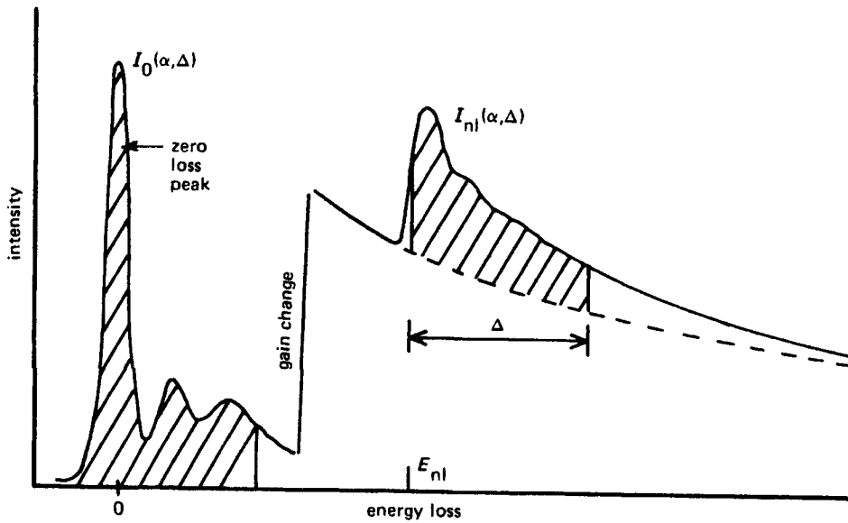
Figure 5.36 Schematic energy-loss spectrum, showing the zero-loss and plasmon regions together with the characteristic ionization edge, energy E_{nl} and intensity I_{nl} .
