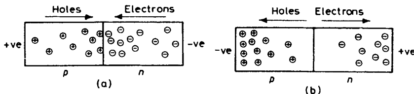
Figure 6.24 Schematic illustration of p - n junction rectification with (a) forward bias and (b) reverse bias.
