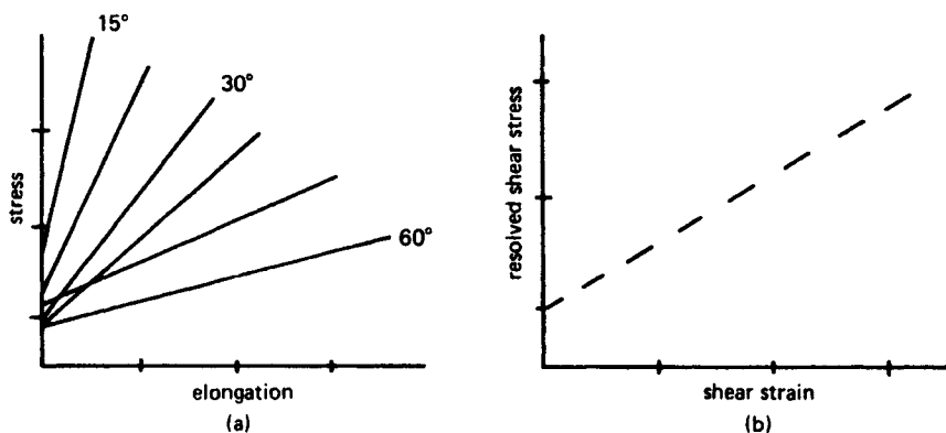
Figure 7.11 Schematic representation of (a) variation of stress versus elongation with orientation of basal plane and (b) constancy of resolved shear stress.
