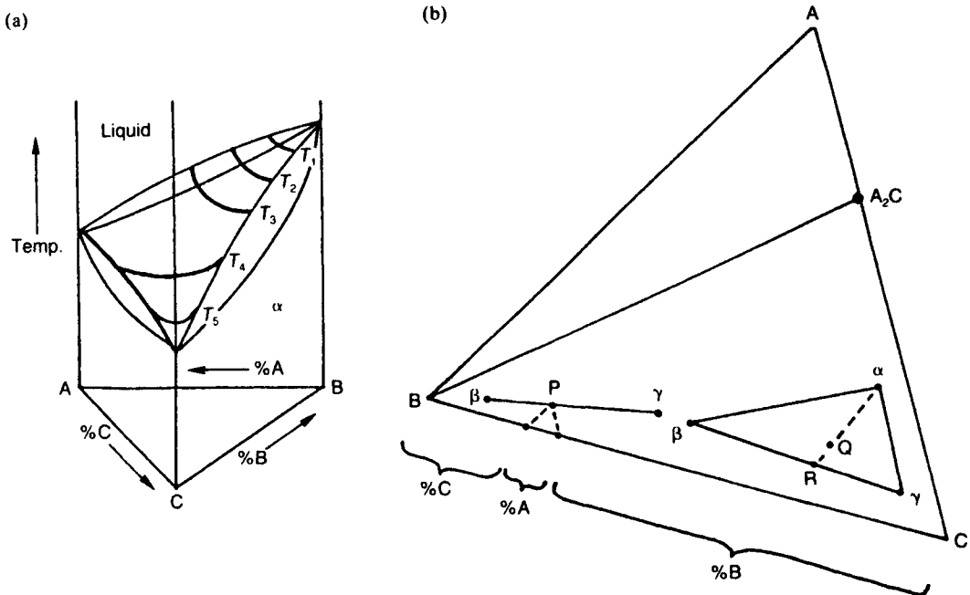
Figure 3.27 (a) Ternary system with complete miscibility in solid and liquid phases and (b) the Gibbs triangle.
