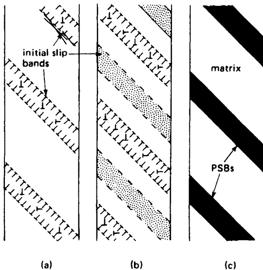
Figure 7.72 Formation of persistent slip bands (PSBs) during fatigue.
