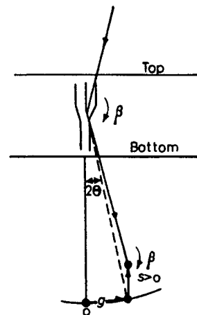
Figure 5.39 Schematic diagram showing the dependence of the dislocation image position on diffraction conditions.
