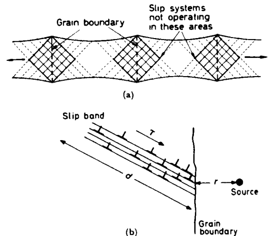
Figure 7.31 (a) Grain-boundary blocking of slip. (b) Blocking of a slip band by a grain boundary.
