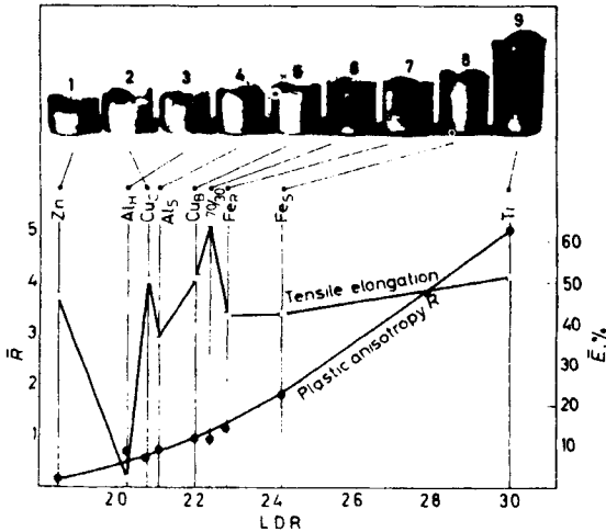
Figure 7.46 Limiting draw ratios (LDR) as a function of average values of R and of elongation to fracture measured in tensile tests at 0^\circ , 45^\circ and 90^\circ to the rolling direction (after Wilson, 1966; courtesy of the Institute of Metals).
