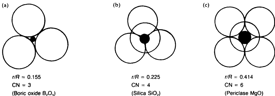
Figure 2.14 Nesting of cations within anionic groups.
