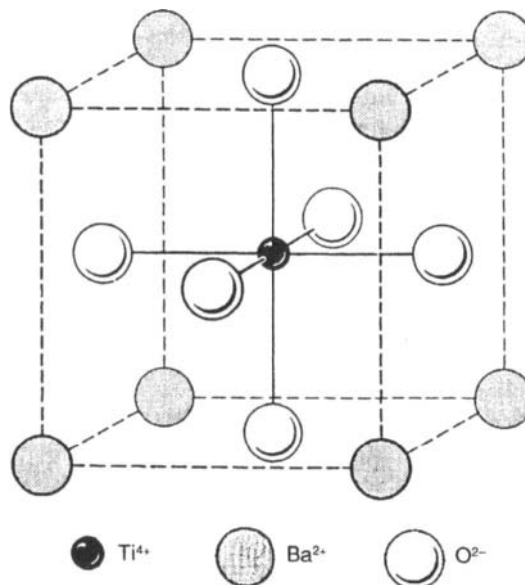
Figure 2.19 Unit cell of cubic \text{BaTiO}_3 ( \text{CN} = 6:12 ) (from Kingery, Bowen and Uhlmann, 1976; by permission of Wiley-Interscience).
