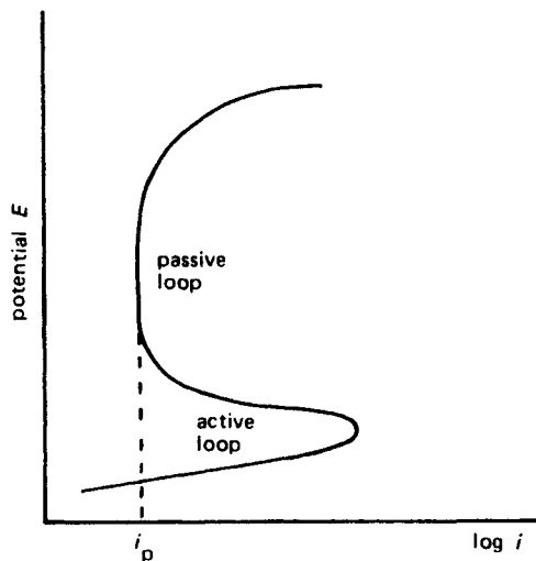
Figure 12.9 Anode polarization curve for stainless steel.
