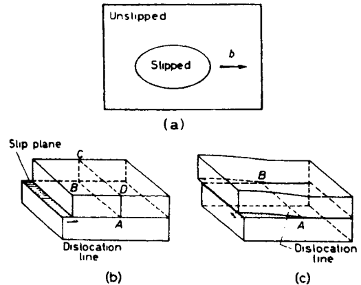
Figure 4.11 Schematic representation of (a) a dislocation loop, (b) edge dislocation and (c) screw dislocation.
