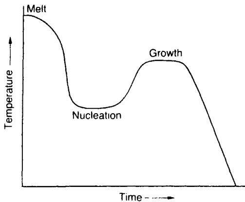
Figure 10.10 Temperature/time schedule for producing a glass-ceramic.
