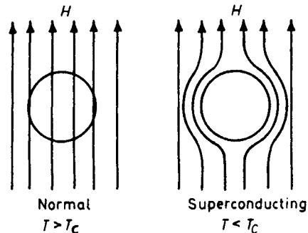
Figure 6.28 The Meissner effect; shown by the expulsion of magnetic flux when the specimen becomes superconducting.
