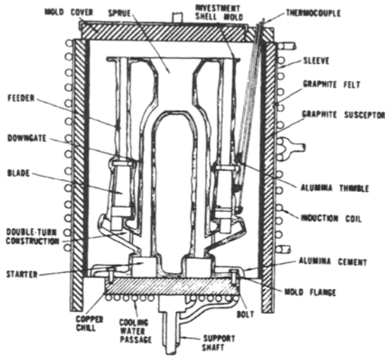
Figure 3.7 Schematic diagram of directional solidification plant for turbine blades.
