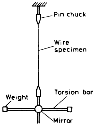
Figure 6.10 Schematic diagram of a K&eacute; torsion pendulum.
