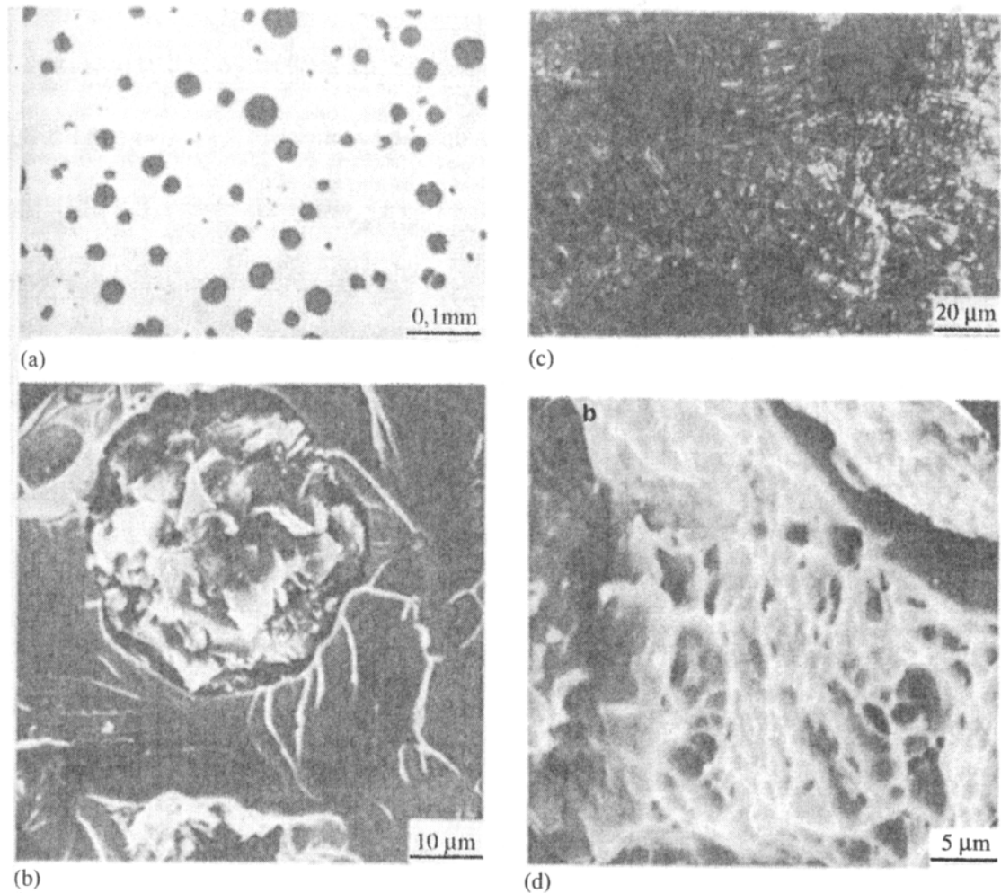
Figure 9.8 Microstructure and fracture mode of silicon spheroidal graphite (SG) iron, (a) and (b) as-cast and (c) and (d) austempered at 350 °C for 1 h (L. Sidjanin and R. E. Smallman, 1992; courtesy of Institute of Metals).
