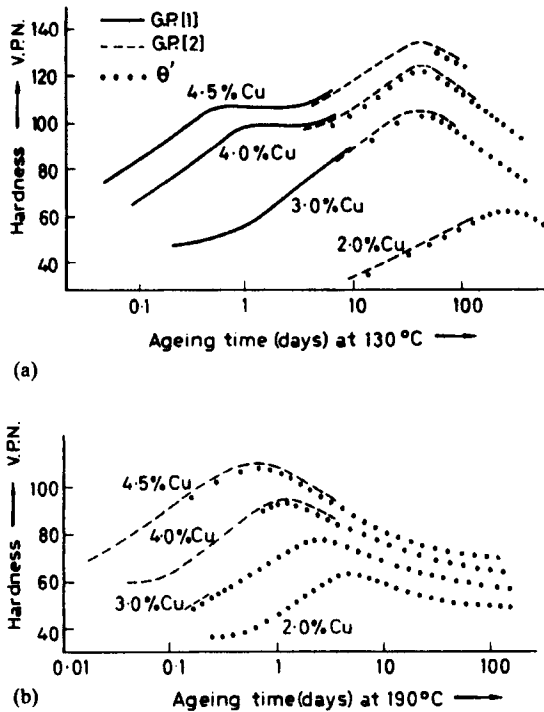
Figure 8.2 The ageing of aluminium-copper alloys at (a) 130°C and (b) at 190°C (after Silcock, Heal and Hardy, 1953-4).
