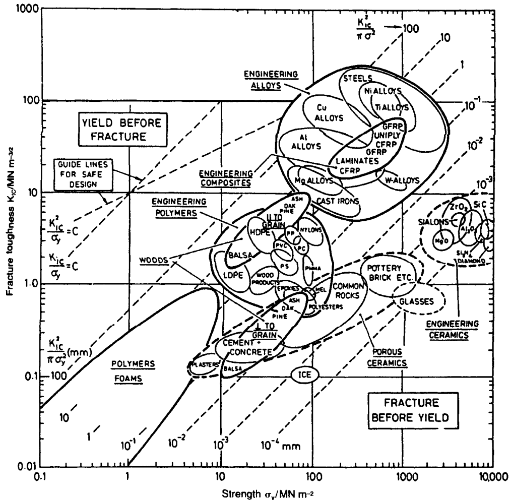
Fracture-toughness, K_{Ic} , plotted against strength, \sigma_y . The contours show the value of K_{Ic}^2/\pi\sigma_y^2 —roughly, the diameter of the process-zone at a crack tip (units: mm). The guide lines of constant K_{Ic}/\sigma_y and K_{Ic}^2/\sigma_y are used in yield-before-break and leak-before-break design.
