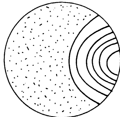
Figure 7.76 A schematic fatigue fracture.
