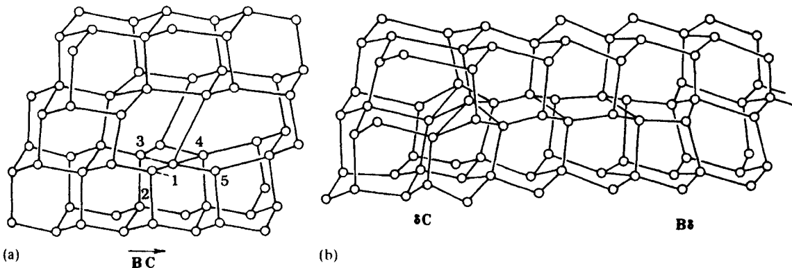
Figure 4.34 (a) The 60^\circ dislocation BC , (b) the dissociation of BC into \delta\text{C} and \text{B}\delta .
