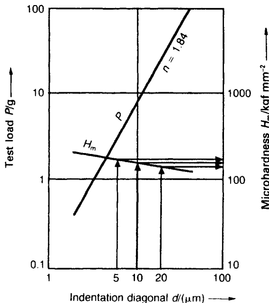
Figure 5.5 Meyer line for material with load-independent hardness (by courtesy of Carl Zeiss, Germany).
