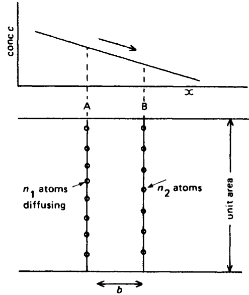
Figure 6.6 Diffusion of atoms down a concentration gradient.
