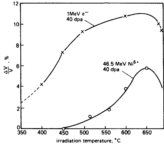
Figure 4.61 Plots of void swelling versus irradiation temperature for 1050°C solution-treated Type 316 irradiated with 1 MeV electrons and 46 MeV Ni ^{6+} to a dose of 40 dpa (after Nelson and Hudson, p. 19).
