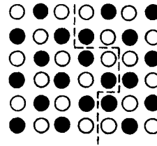
Figure 6.13 An antiphase domain boundary.
