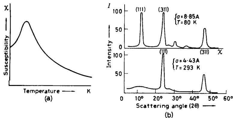
Figure 6.34 (a) Variation of magnetic susceptibility with temperature for an anti-ferromagnetic material, (b) neutron diffraction pattern from the anti-ferromagnetic powder \text{MnO} above and below the critical temperature for ordering (after Shull and Smart, 1949).
