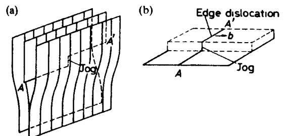
Figure 4.17 Climb of an edge dislocation in a crystal.
