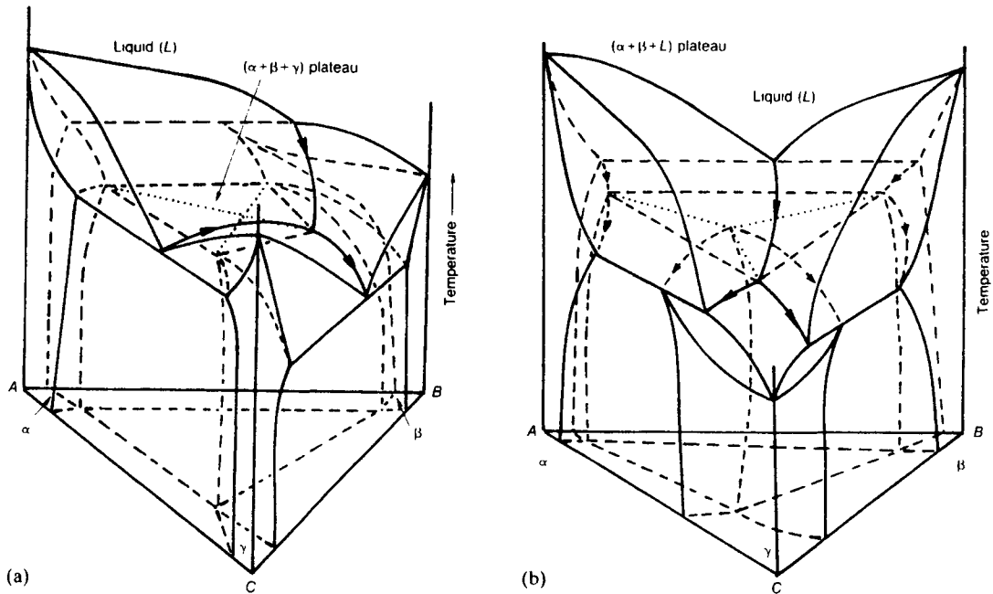
Figure 3.34 Phase diagrams illustrating (a) Class II equilibrium ( Liquid + \alpha \rightleftharpoons \beta + \gamma ), and (b) Class III equilibrium ( Liquid + \alpha + \beta \rightleftharpoons \gamma ) (after Rhines, 1956).
