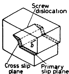
Figure 4.16 Cross-slip of a screw dislocation in a crystal.
