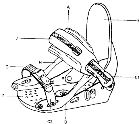
Figure 14.7 Snowboard binding utilizing: thermoplastic elastomer ( Hytrel )—ankle strap A, spoiler B, ratchet strap G, nylon ( Zytel )—side frames D and H, base and disc F, top frame J; acetal homopolymer ( Delrin )—strap buckles C1 and C2 (courtesy of Fritschi Swiss Bindings AG and Du Pont UK Ltd).
