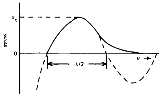
Figure 8.29 Model for estimating the theoretical fracture strength \sigma_t .
