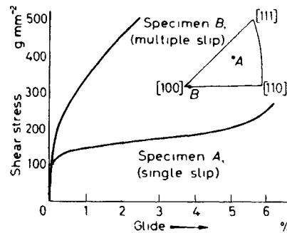
Figure 7.14 Stress-strain curves for aluminium deformed by single and multiple slip (after Lücker and Lange, 1950).
