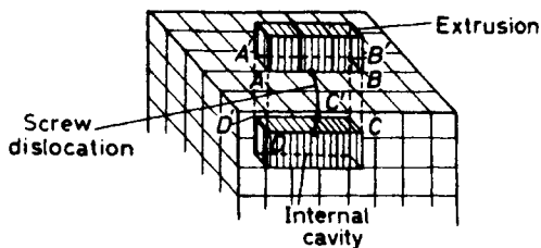
Figure 7.75 Formation of an extrusion and associated cavity by the Mott mechanism.
