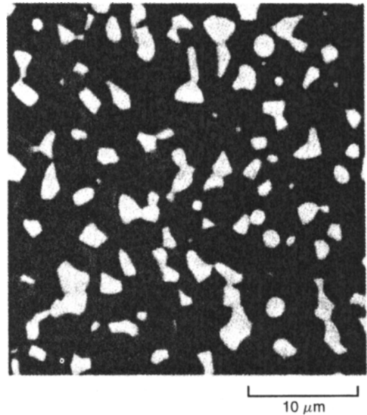
Figure 10.9 Duplex structure of ZT ( \text{Al}_2\text{O}_3 ) consisting of alumina and t -zirconia grains (back-scattered electron image). (from Green, 1984, p. 84; by permission of Marcel Dekker Inc.).
