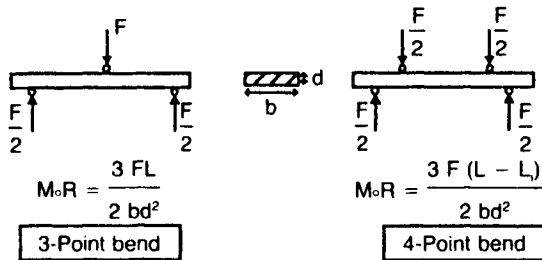
Figure 7.6 Bend test configurations. MoR = modulus of rupture, F = applied force, L = outer span, L_i = inner span, b = breadth of specimen, d = depth of specimen.
