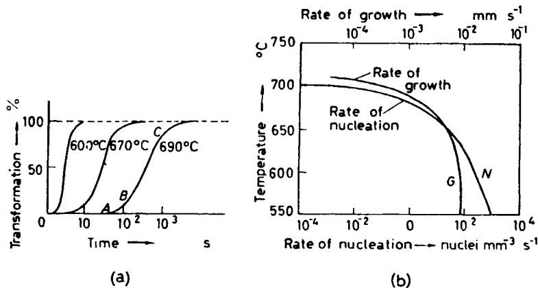
Figure 8.19 Effect of temperature on (a) amount of pearlite formed with time and (b) rate of nucleation and rate of growth of pearlite (after Mehl and Hagel, 1956; courtesy of Pergamon Press).
