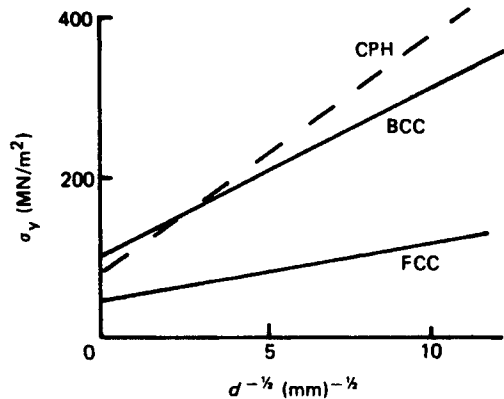
Figure 7.32 Schematic diagram showing the grain size-dependence of the yield stress for crystals of different crystal structure.
