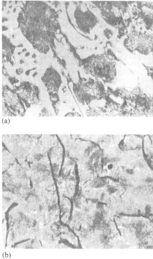
Figure 9.7 Microstructure of cast irons: (a) white iron and (b) grey iron (400 \times ). (a) shows cementite (white) and pearlite; (b) shows graphite flakes, some ferrite (white) and a matrix of pearlite.
