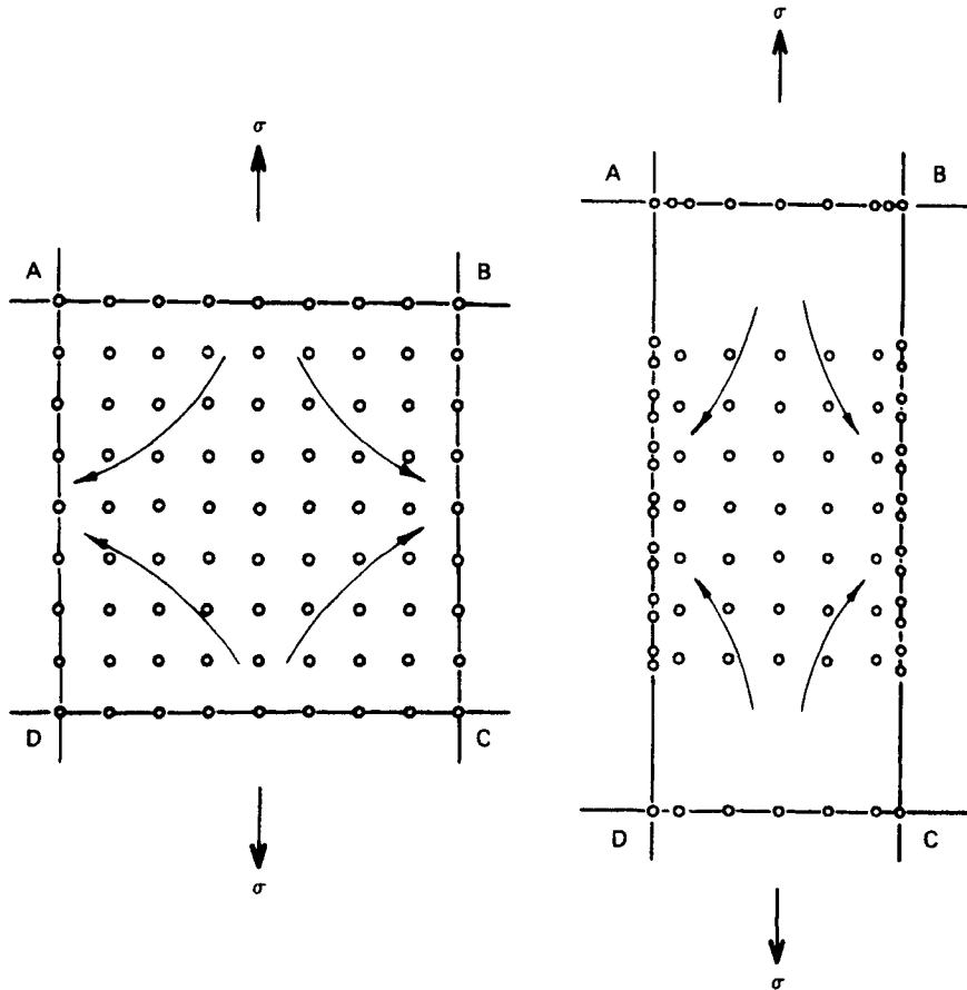
Figure 7.67 Schematic diagram showing the distribution of second-phase particles before and after diffusion creep.
