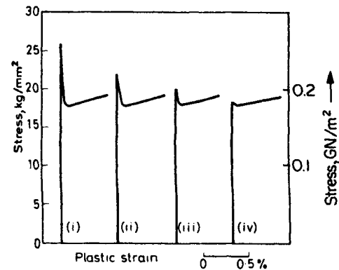
Figure 7.26 Calculated stress-strain curves showing influence of initial dislocation density on the yield drop in iron for n = 35 with (i) 10^1 \text{ cm}^{-2} , (ii) 10^3 \text{ cm}^{-2} , (iii) 10^5 \text{ cm}^{-2} and (iv) 10^7 \text{ cm}^{-2} (after Hahn, 1962; courtesy of Pergamon Press).
