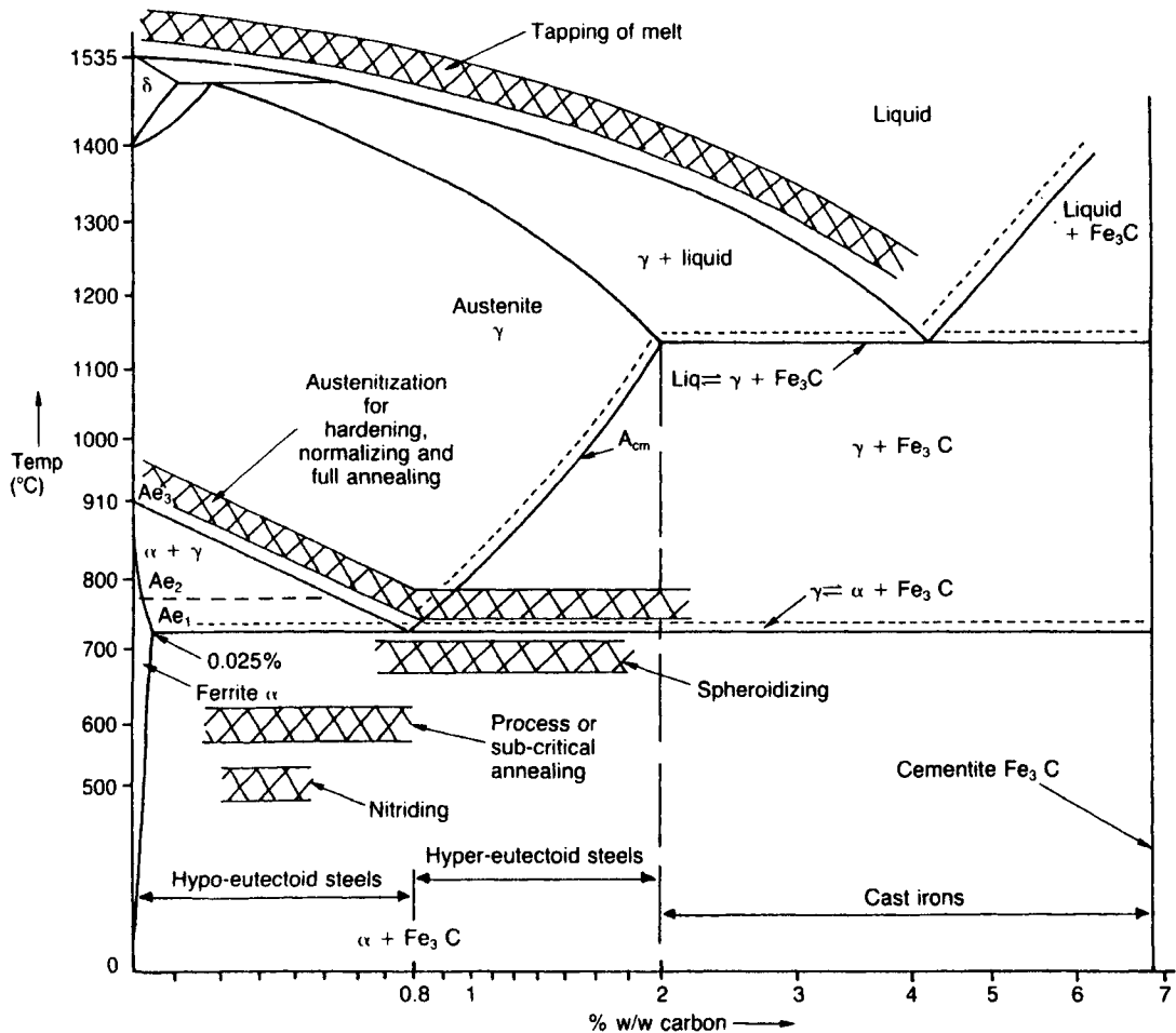
Figure 3.21 Phase diagram for Fe-C system (dotted lines represent iron-graphite equilibrium).
