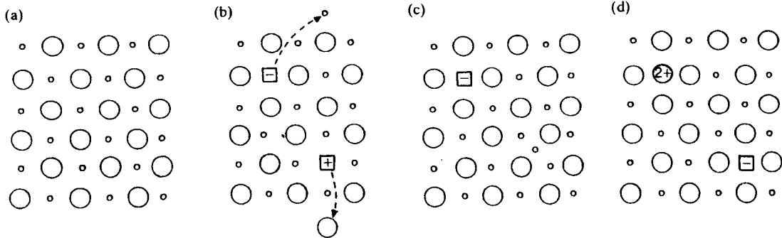
Figure 4.5 Representation of point defects in two-dimensional ionic structure: (a) perfect structure and monovalent ions, (b) two Schottky defects, (c) Frenkel defect, and (d) substitutional divalent cation impurity and cation vacancy.
