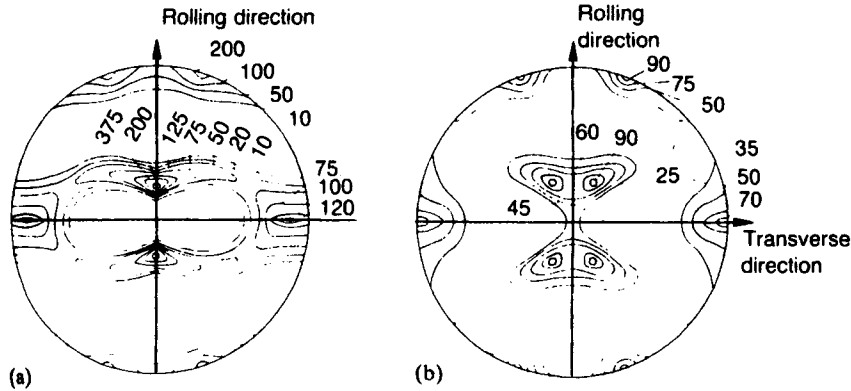
Figure 7.44 (111) pole figures from (a) copper, and (b) \alpha -brass after 95% deformation (intensities in arbitrary units).
