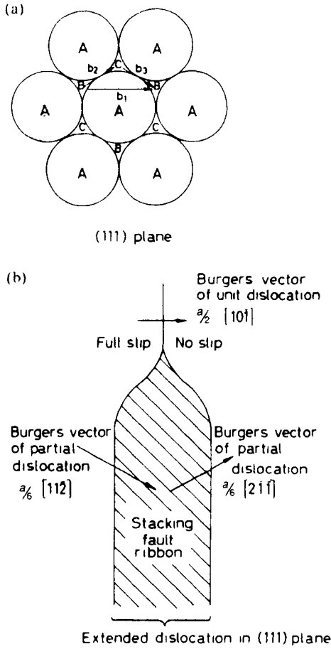
Figure 4.28 Schematic representation of slip in a (111) plane of a fcc crystal.
