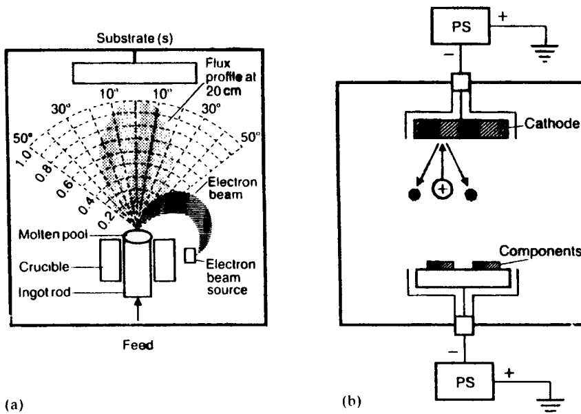
Figure 12.12 (a) Evaporation-dependent and (b) sputter-dependent PVD (from Barrell and Rickerby, Aug 1989, pp. 468–73; by permission of the Institute of Materials).
