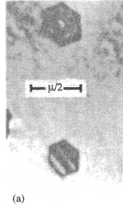
Figure 4.41 Triple-loop and Frank sessile loop in Al-0.65% Mg (after Kritzing, Smallman and Dobson, 1969; courtesy of Pergamon Press).
