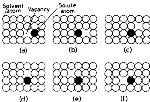
Figure 6.7 Solute atom–vacancy association during diffusion.
