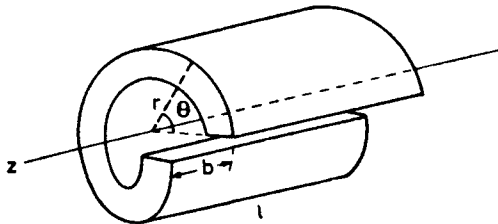
Figure 4.21 Screw-dislocation in an elastic continuum.
