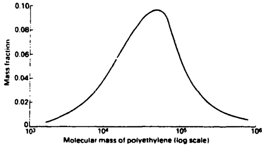
Figure 2.23 The molecular mass distribution of a polyethylene, determined using GPC (from Mills, 1986; by permission of Edward Arnold).
