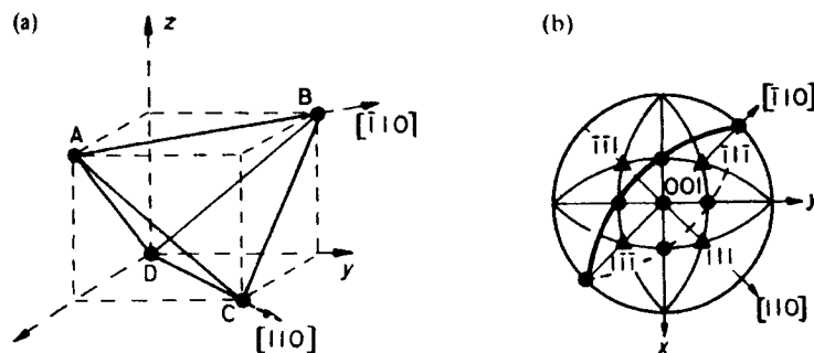
Figure 4.36 (a) Construction and (b) orientation of the Thompson tetrahedron ABCD. The slip directions in a given \{111\} plane may be obtained from the trace of that plane as shown for the (111) plane in (b).
