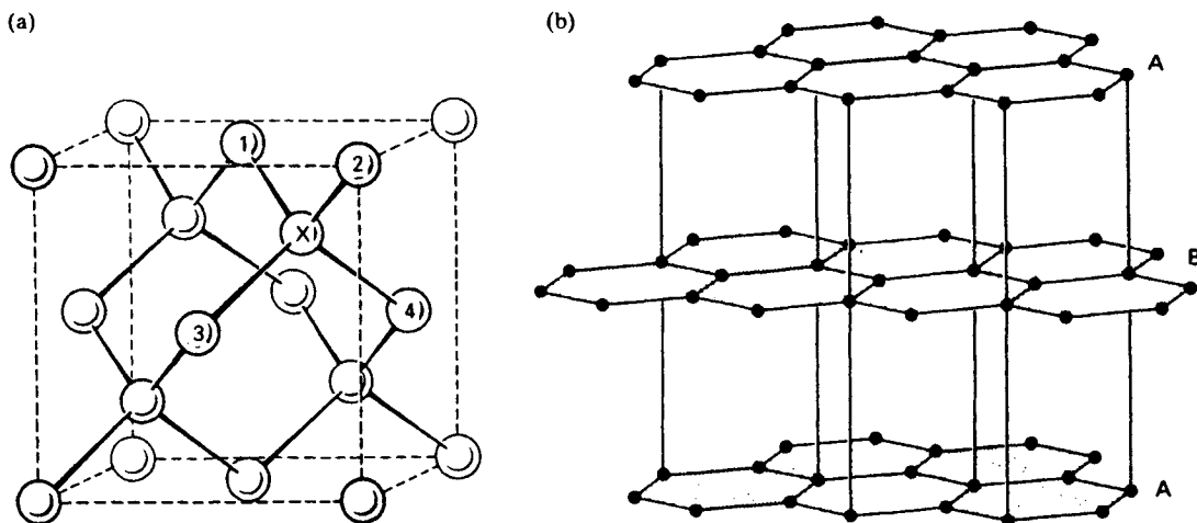
Figure 2.13 Two crystalline forms of carbon: (a) diamond and (b) graphite (from Kingery, Bowen and Uhlmann, 1976; by permission of Wiley-Interscience).
