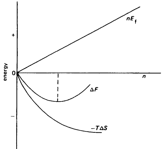
Figure 4.3 Variation of the energy of a crystal with addition of n vacancies.
