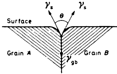
Figure 4.27 Grain boundary/surface triple junction.
