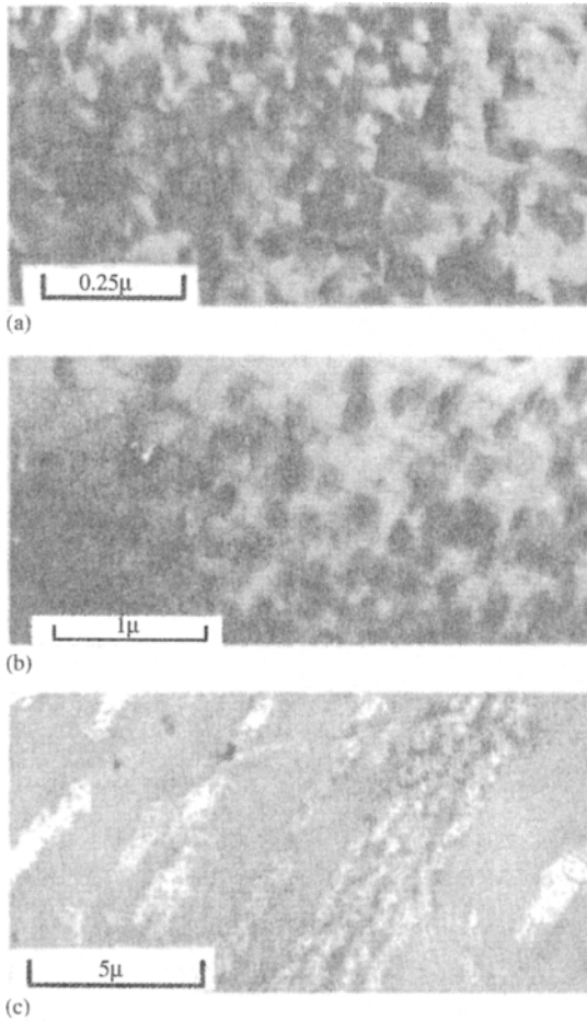
Figure 8.4 Electron micrographs from Al–4Cu (a) aged 5 hours at 160°C showing \theta'' plates, (b) aged 12 hours at 200°C showing a dislocation ring round \theta'' plates, (c) aged 3 days at 160°C showing \theta'' precipitated on helical dislocations (after Nicholson, Thomas and Nutting, 1958–9).
