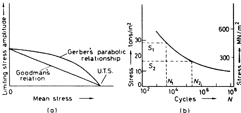
Figure 7.69 Fatigue relationships.
