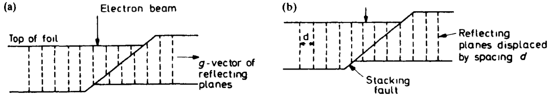
Figure 5.41 Schematic diagram showing (a) displacement of reflecting planes by a stacking fault and (b) the condition for g \cdot \mathbf{R} = n when the fault would be invisible.
