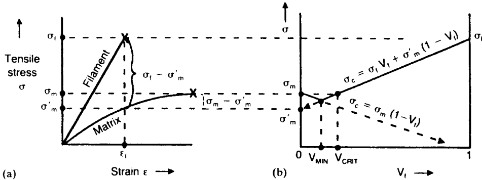
Figure 11.12 (a) Stress–strain curves for filament and matrix and (b) dependence of composite strength on volume fraction of continuous filaments.
