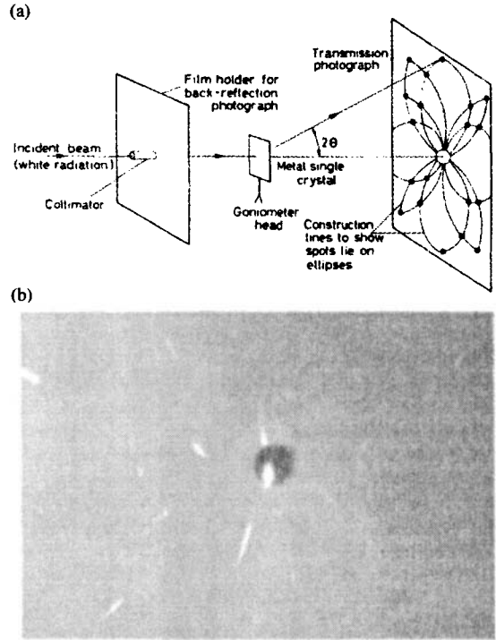
Figure 5.10 (a) Laue method of X-ray diffraction. (b) Asterisms on a Laue transmission photograph of deformed zinc (after Cahn, 1949).
