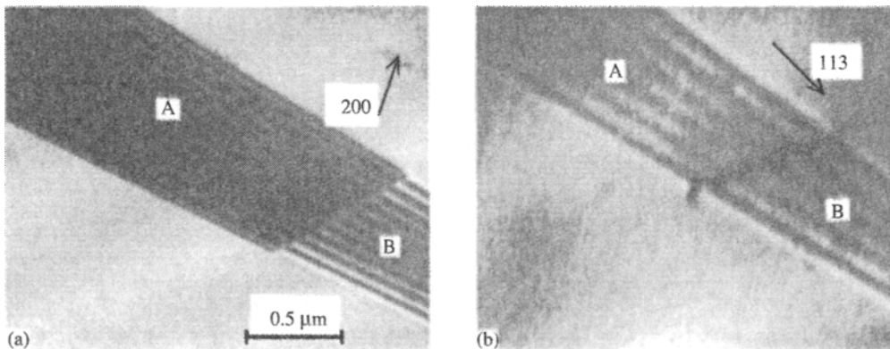
Figure 8.25 Electron micrographs showing (a) contrast from overlapping faults on (1\ 1\ 1) ; A is extrinsic and B is intrinsic in nature. (b) Residual contrast arising from a supplementary displacement across the faults which is intrinsic in nature for both faults A and B (after Brooks, Loreto and Smallman, 1979).
