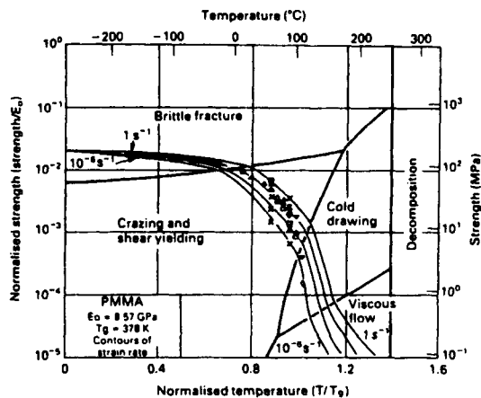
Figure 11.5 Deformation map for PMMA showing deformation regions as a function of normalized stress versus normalized temperature (from Ashby and Jones, 1986; permission of Elsevier Science Ltd, UK).
