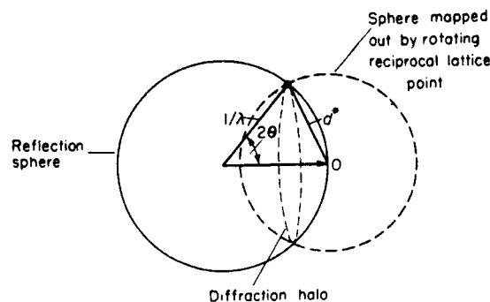
Figure 5.19 Principle of the powder method.
