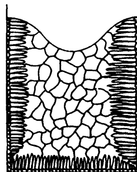
Figure 3.5 Chill-cast ingot structure.
