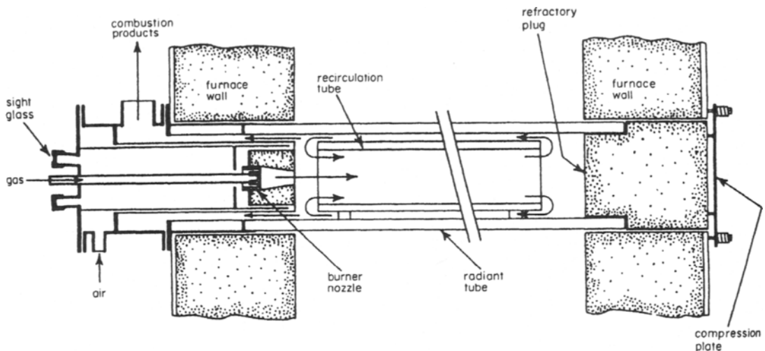
Figure 10.13 Operating principle of the ceramic radiant tube (from Wedge, Jan 1987, pp. 36–8; by courtesy of the Institute of Materials).
