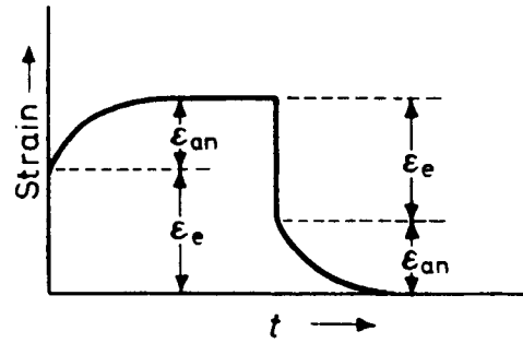
Figure 6.9 Anelastic behaviour.
