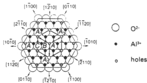
Figure 2.18 Structure of \alpha -alumina (corundum) viewed perpendicular to (0\ 0\ 0\ 1) basal plane (from Hume-Rothery, Smallman and Haworth, 1988).
