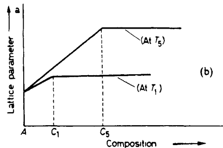
Figure 5.16 (a) and (b) Phase-boundary determination using lattice parameter measurements.
