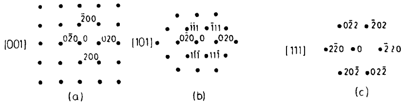
Figure 5.28 fcc cross-grating patterns (a) [0\ 0\ 1] , (b) [1\ 0\ 1] and (c) [1\ 1\ 1] .
