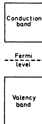
Figure 6.22 Schematic diagram of an intrinsic semiconductor showing the relative positions of the conduction and valency bands.
