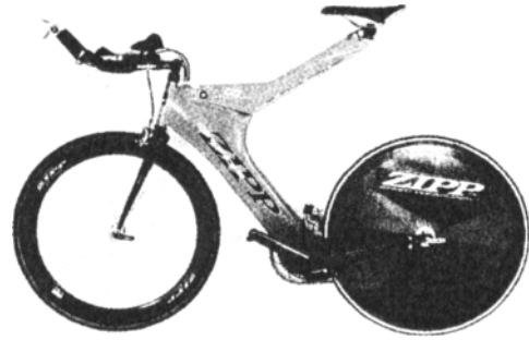
Figure 14.6 High-performance Zipp bicycle with monocoque frame (courtesy of Julian Ormandy, School of Metallurgy and Materials, University of Birmingham, UK).
