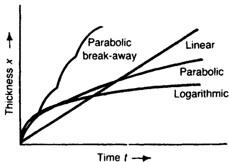
Figure 12.2 Different forms of oxidation behaviour in metals.
