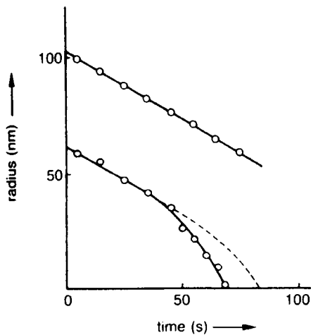
Figure 4.57 Variation of loop radius with time of annealing for Frank dislocations in Al showing the deviation from linearity at small r .
