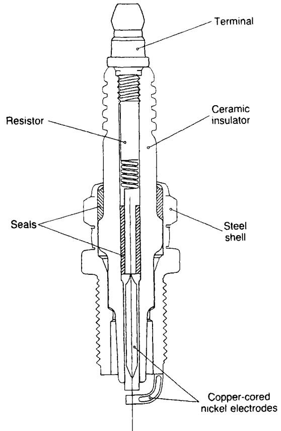
Figure 10.1 Spark plug for petrol engine (with acknowledgements to Champion Spark Plug Division of Cooper GB Ltd).
