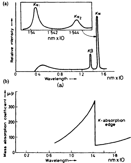
Figure 5.8 (a) Distribution of X-ray intensity from a copper target and (b) dependence of mass absorption coefficient on X-ray wavelength for nickel.
