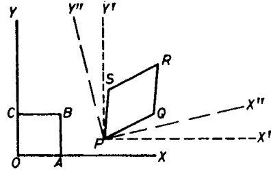
Figure 7.8 Deformation of a square OABC to a parallelogram PQRS involving (i) a rigid body translation OP allowed for by redefining new axes X'Y' , (ii) a rigid body rotation allowed for by rotating the axes to X''Y'' , and (iii) a change of shape involving both tensile and shear strains.
