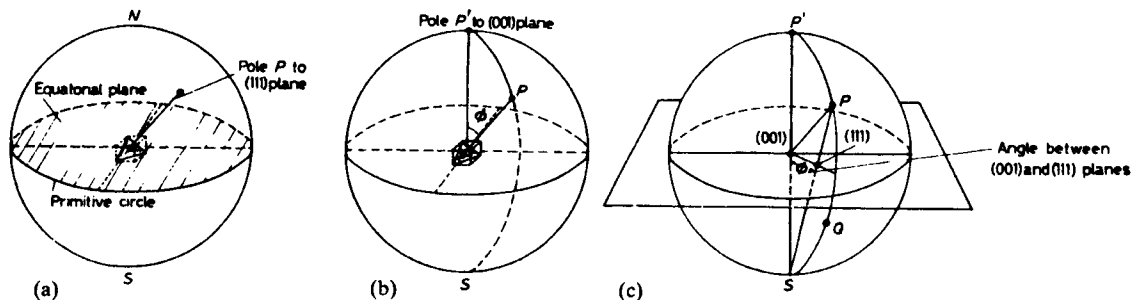
Figure 2.7 Principles of stereographic projection, illustrating (a) the pole P to a (111) plane, (b) the angle between two poles, P , P' and (c) stereographic projection of P and P' poles to the (111) and (001) planes, respectively.
