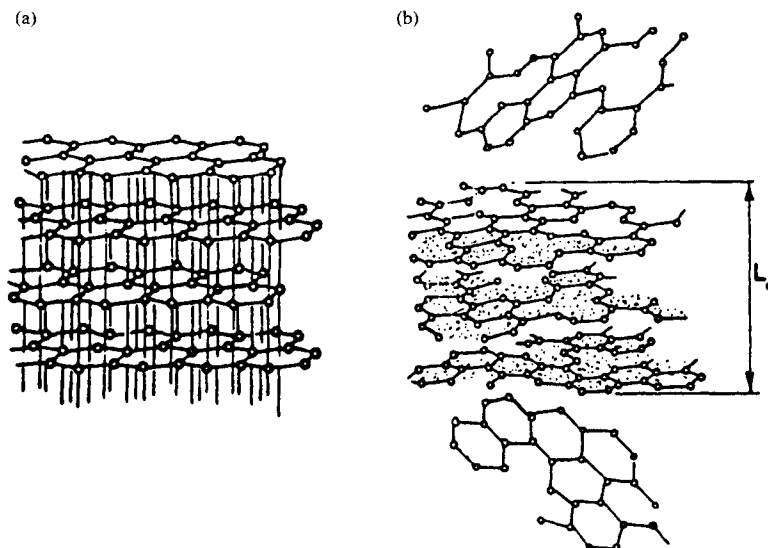
Figure 10.15 Structures of (a) crystalline graphite and (b) turbostratic carbon (from Cahn and Harris, 11 Jan, 1969, pp. 132–41; by permission of Macmillan Magazines Ltd).
