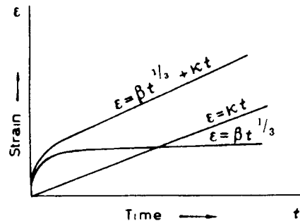
Figure 7.60 Combination of transient and steady-state creep.
