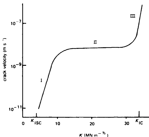
Figure 12.10 Variation of crack growth rate with stress intensity during corrosion.
