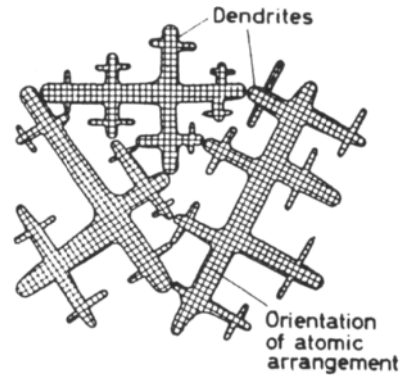
Figure 3.2 Schematic diagram of three dendrites interlocking.
