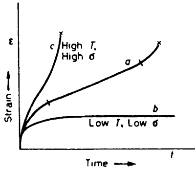
Figure 7.3 Typical creep curves.
