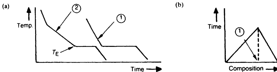
Figure 3.17 (a) Typical cooling curves for hypo-eutectic alloy 2 and eutectic alloy 1 in Figure 3.16 and (b) dependence of duration of cooling arrest at eutectic temperature T_E on composition.
